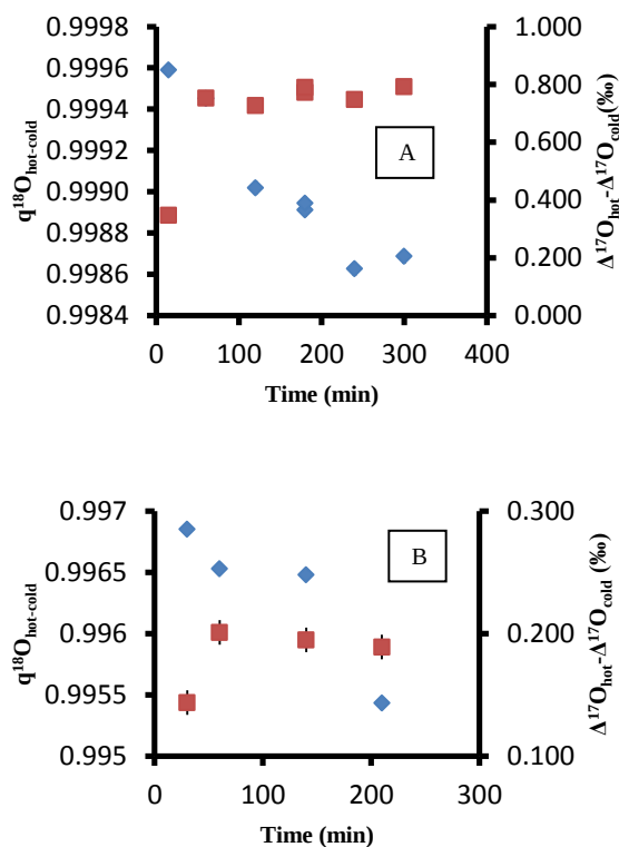
Figure 1, Time course for isotope fractionation factor ( q_{\text{hot-cold}} , blue diamonds) and for \Delta\Delta^{17}\text{O} ( \Delta^{17}\text{O}_{\text{hot}} - \Delta^{17}\text{O}_{\text{cold}} , red square) difference between hot and cold reservoir. A) 5.3 Torr pressure with upper +20°C-lower -196°C, B) 12 Torr pressure with upper +20°C-lower +260°C. Error bars (s. e. \times t) are 0.00002 and 0.01‰ for q_{\text{hot-cold}} and \Delta\Delta^{17}\text{O} , respectively. Error bar is smaller than symbol size if not shown.
