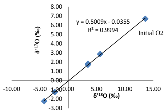
Figure 2, Relationships between the \delta^{17}\text{O} and the \delta^{18}\text{O} for final \text{CeO}_2 and initial \text{O}_2 gas. The overall slope is much shallower than either diffusion slope ( \sim 0.511 ) or isotope exchange at 700^\circ\text{C} ( \sim 0.529 ).
