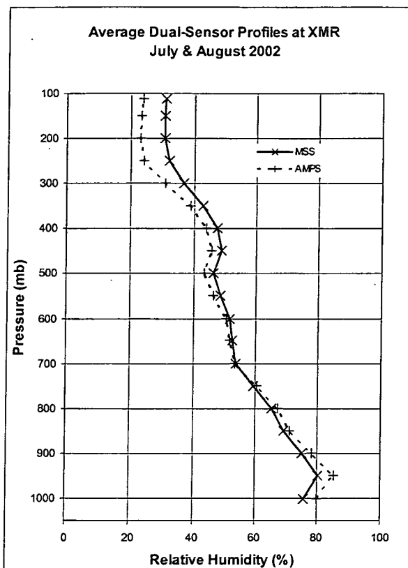
Figure 6. Vertical profiles of average relative humidity from the MSS (solid) and AMPS (dashed) sensors for twenty dual-sensor ascents taken in July and August 2002.
