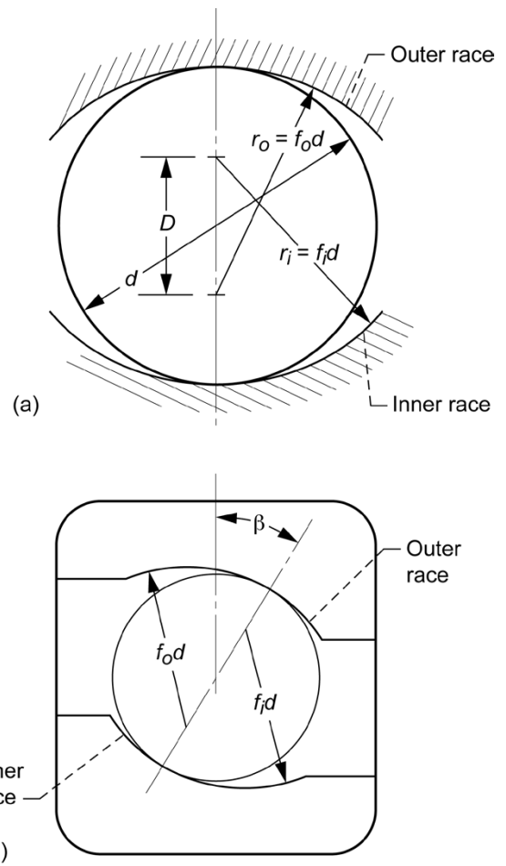
Figure 7.—Ball-race conformity. (a) Deep-groove ball bearing. (b) Angular-contact ball bearing.
