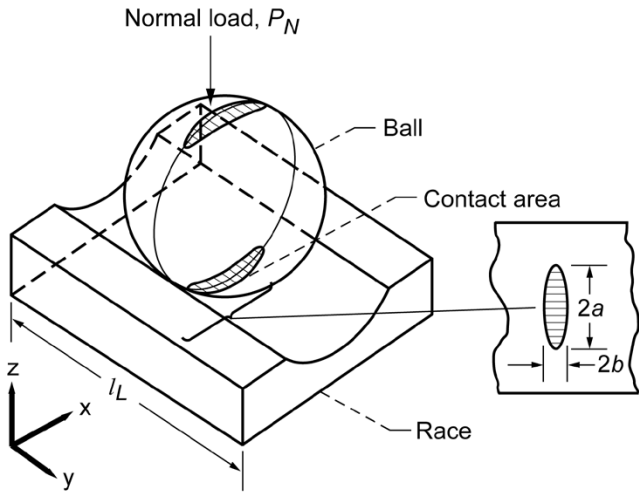
Figure 3.—Ball-race model for point contact.
