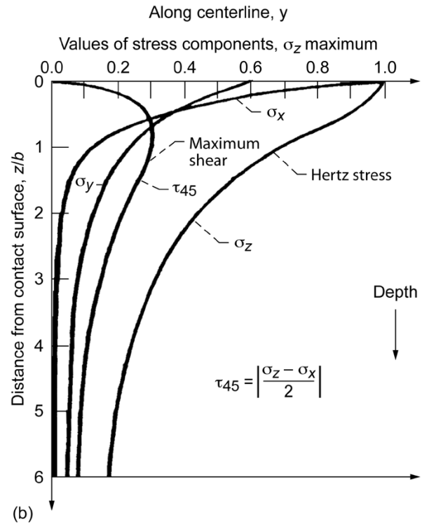
Figure 5.—Subsurface stress field under line contact.
