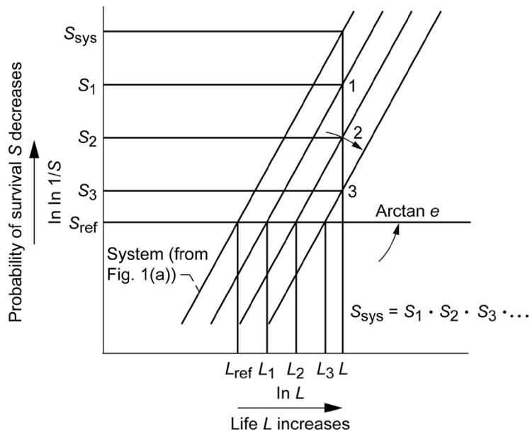
Figure 27.—Sketch of multiple Weibull plots where each numbered plot represents cumulative distribution of each component in system and system Weibull plot represents combined distribution of plots 1, 2, 3, etc. (all plots are assumed to have same Weibull slope e ) (Ref. 98).
