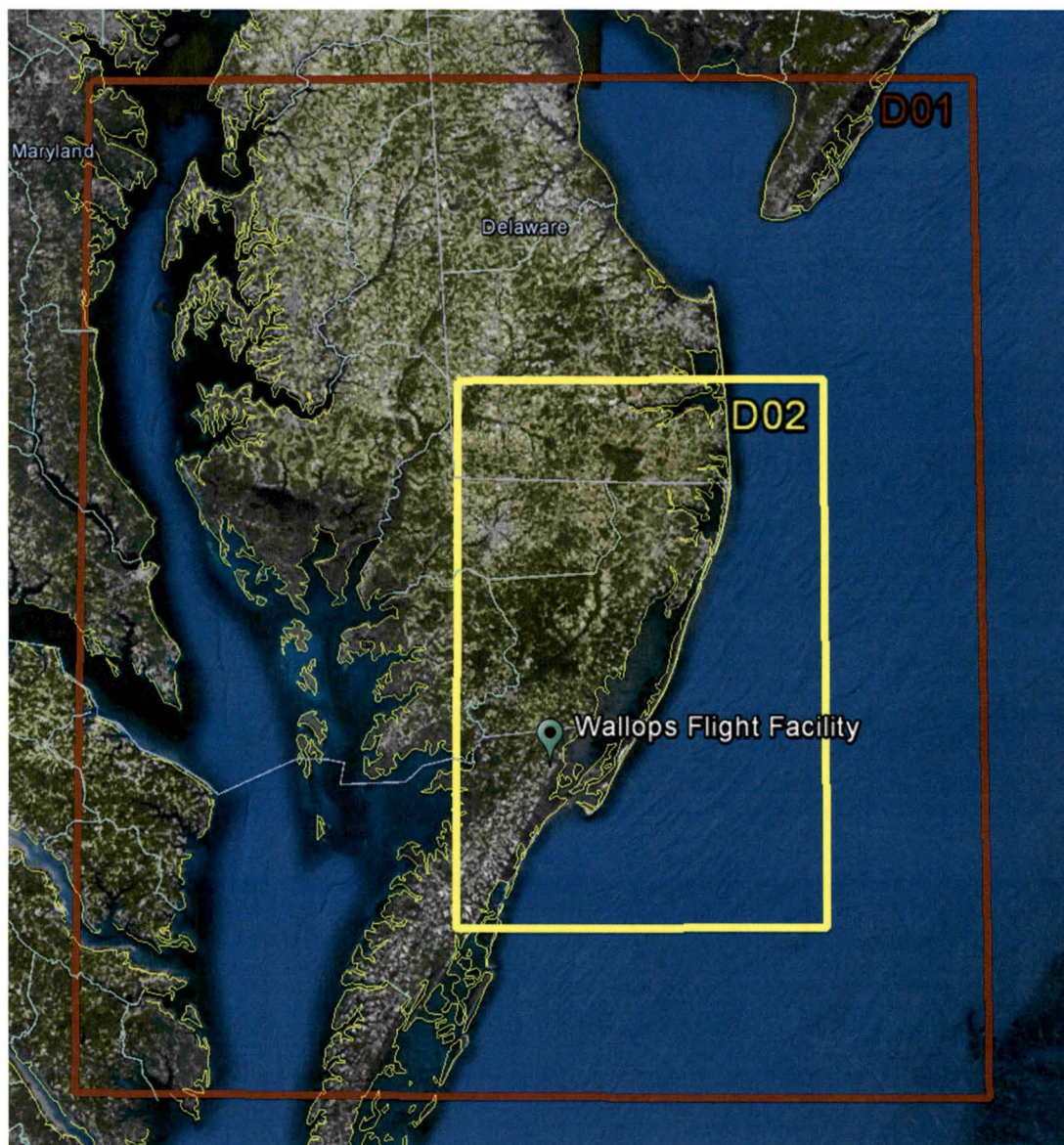
Figure 4. Map of the Delmarva Peninsula showing the WRF NMM model domain boundaries. The red rectangle shows the outer 3 km domain and the yellow rectangle the inner 1 km domain.
