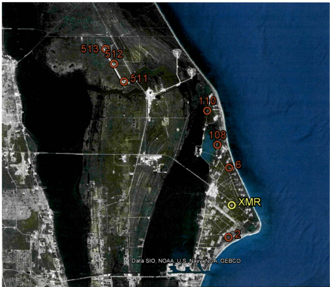
Figure 2. The locations of the seven KSC/CCAFS wind towers and their numbers that were used to validate the WRF forecasts on the ER are shown in red. The XMR RAOB site used to validate the upper air forecasts is shown in yellow.
