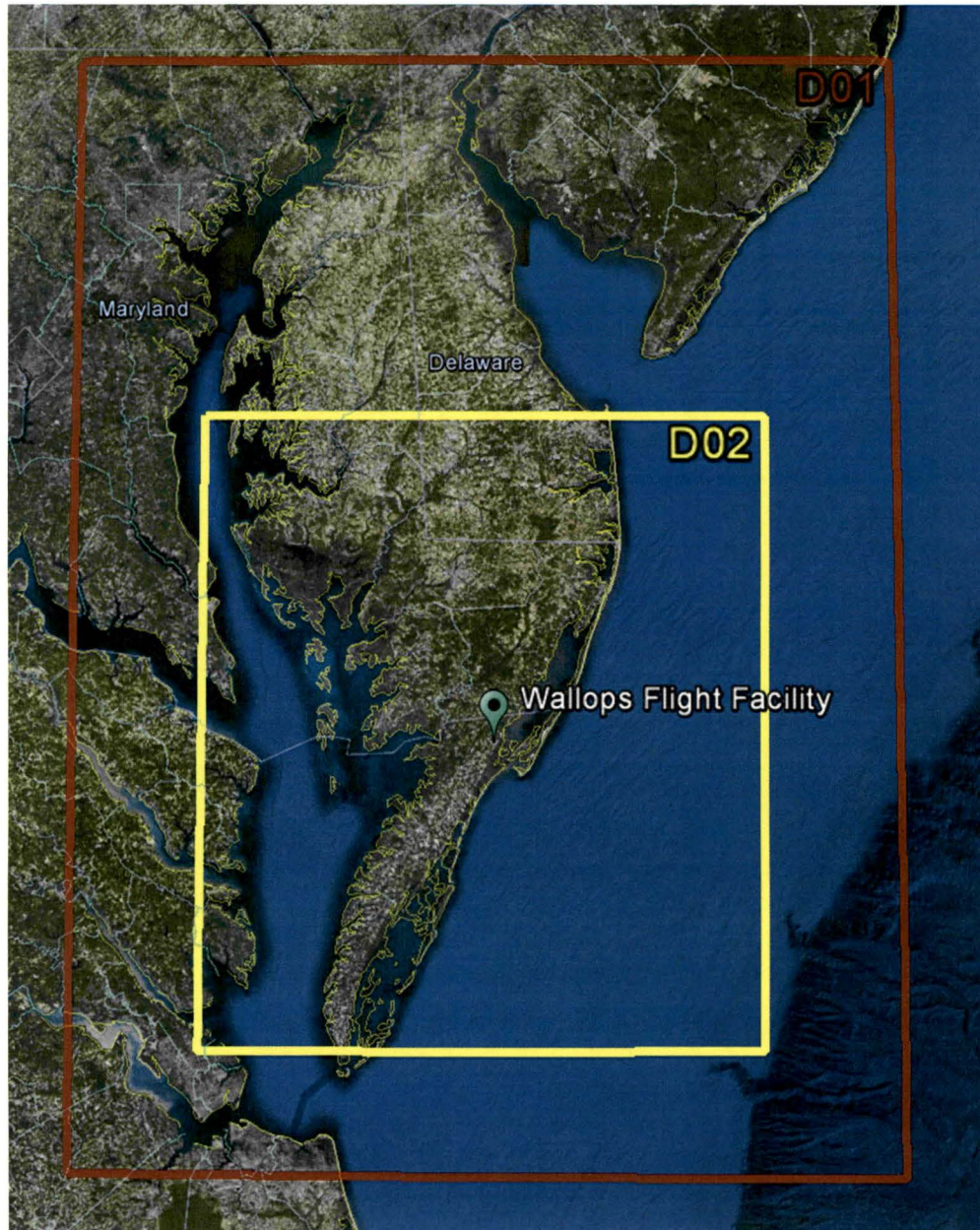
Figure 3. Map of the Delmarva Peninsula showing the WRF ARW model domain boundaries. The red rectangle shows the outer 4 km domain and the yellow rectangle the inner 1.33 km domain.
