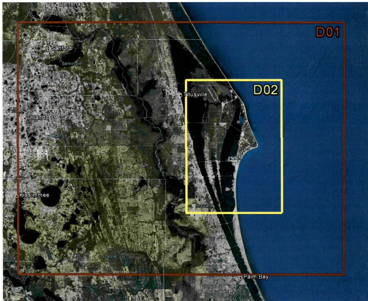
Figure 1. Map of east-central Florida showing the model domain boundaries. The red rectangle shows the outer domain and the yellow rectangle the inner domain for all configurations regardless of horizontal resolution or domain core.
