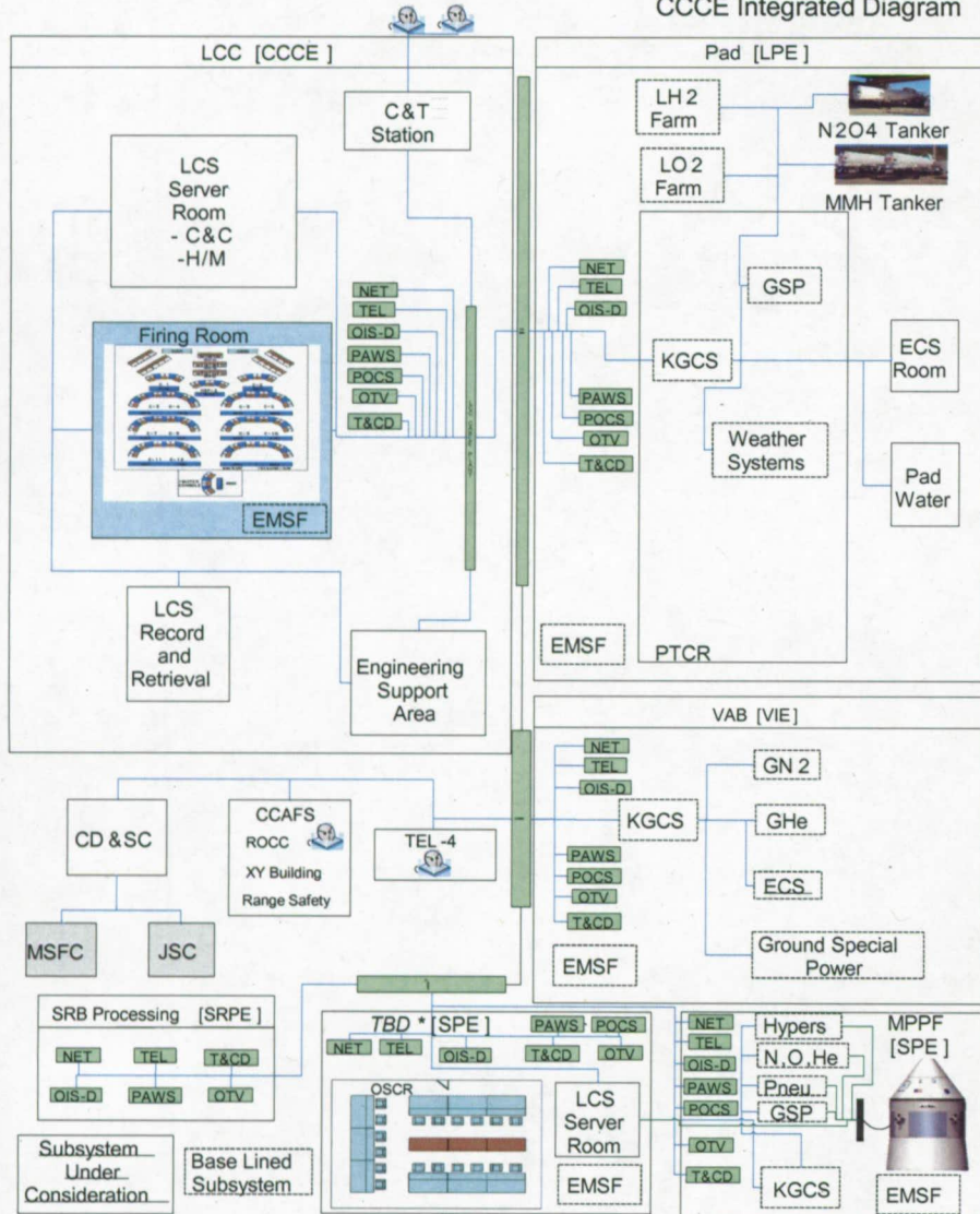
CCCE Integrated Diagram
