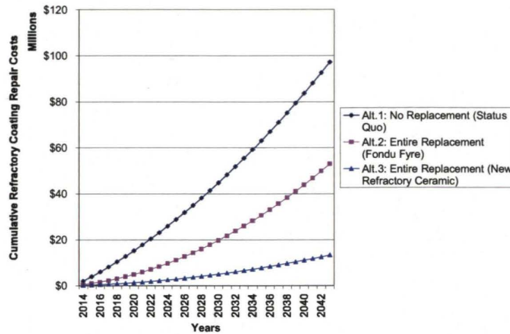
Figure 29. Comparison of Refractory Alternative Repair Costs
