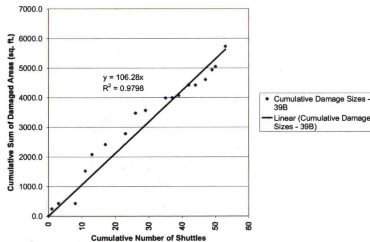
Figure 22. Cumulative Damages vs. Cumulative No. of Launches – LC 39B
