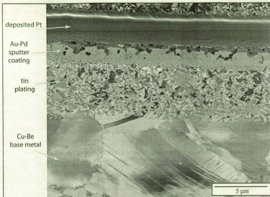
Figure 5-19 FIB ion channeling image of a card guide 16 (ATVC S/N 31) cross section showing the distinct layers studied: the expected Cu-Be substrate with larger grains, the Sn plating with nm-sized grains, the Au-Pd sputter coating and finally the deposited Pt used to protect the region during FIB (NASA/UCF). Magnification: 15,000X.
