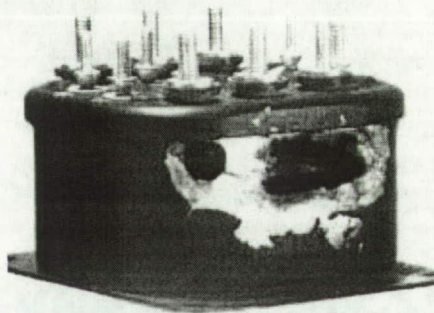
Figure 2-5 Failed relay from tin whisker induced metal vapor arc (Photo courtesy of NASA EEE Parts and Packaging (NEPP) Program)
