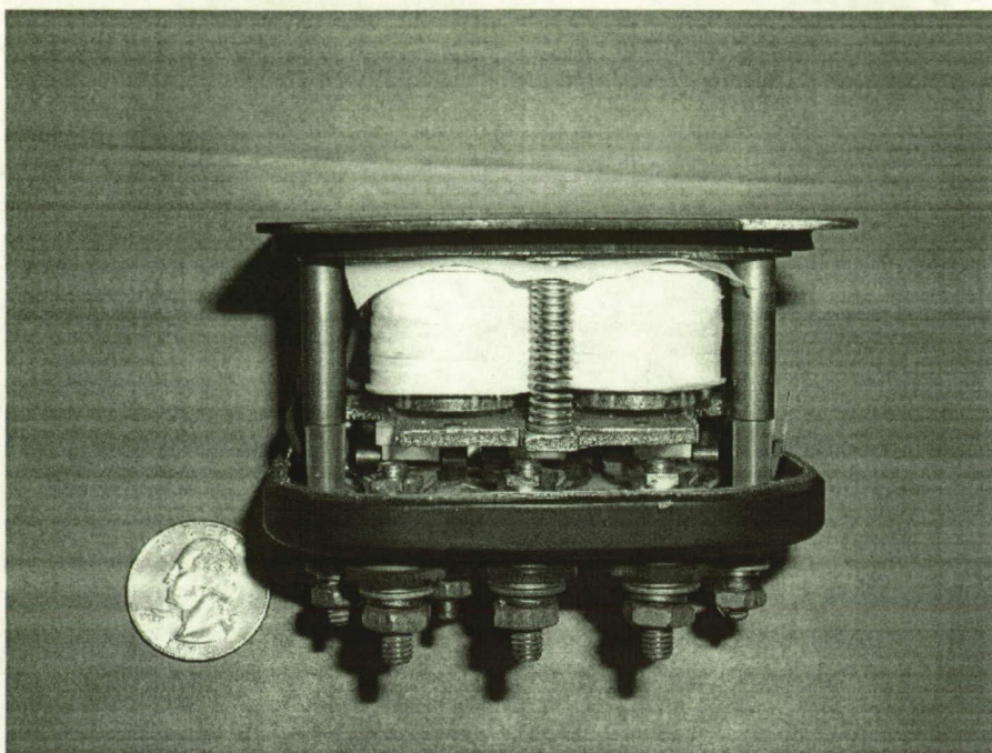
Figure 2-1 Relay with cover removed (Photo courtesy of NASA EEE Parts and Packaging (NEPP) Program)
