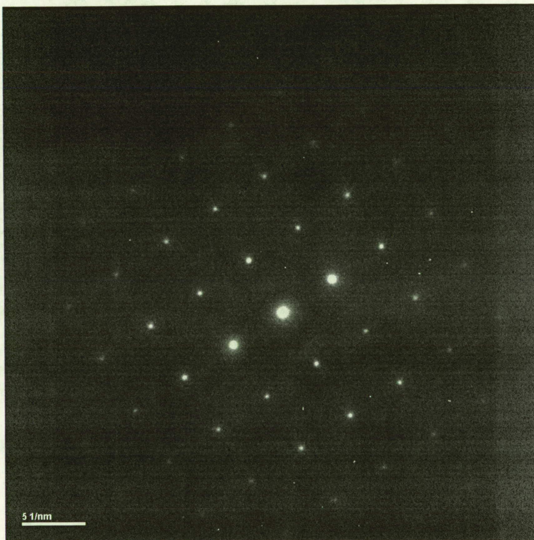
Diffraction Pattern for Polycrystalline Whisker Section A
