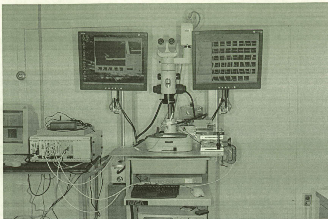
Figure 4-1 Tin whisker test station - full experiment
