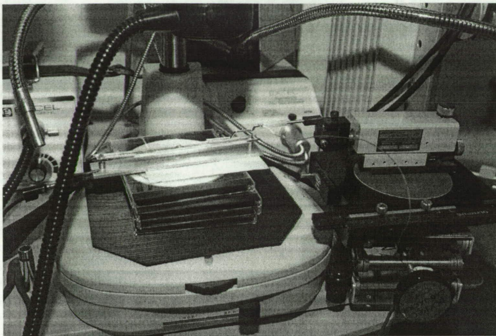
Figure 3-2 Micromaniputlator and card guide
