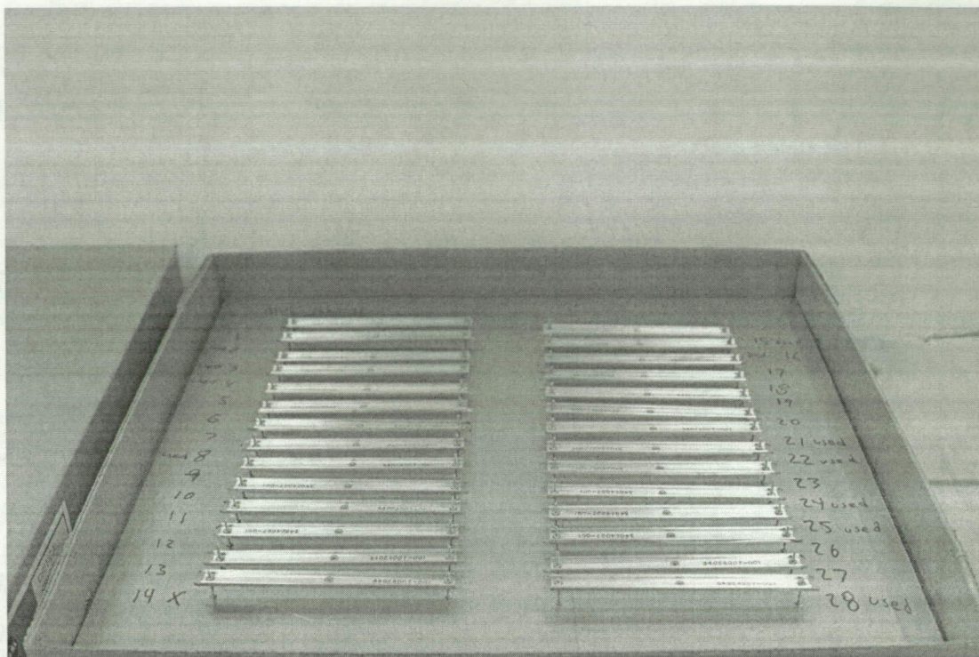
Figure 4-4 ATVC 31 card guides
