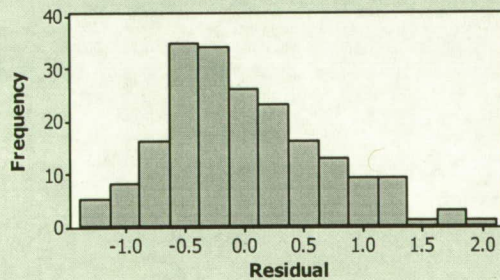
Histogram of the Residuals
