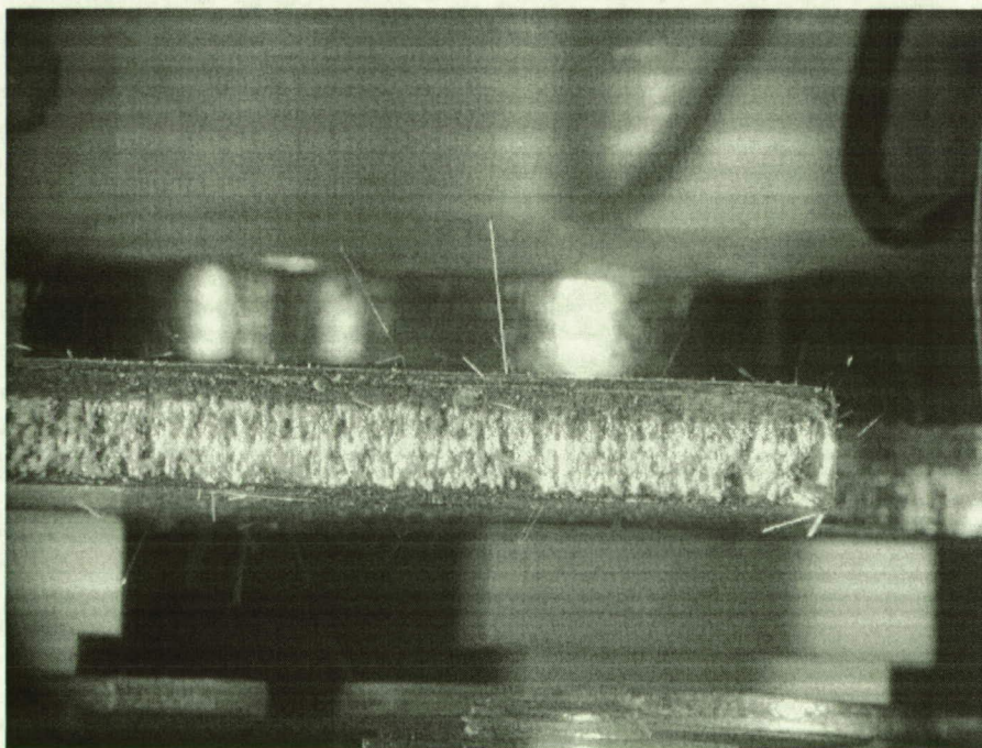
Figure 2-2 Tin whiskers growing on armature of a hermetically seals relay (Photo courtesy of NASA EEE Parts and Packaging (NEPP) Program)
