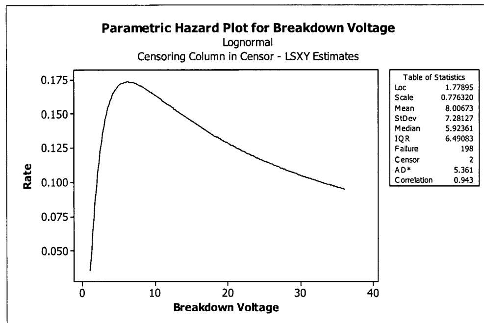
Figure 5-9 Hazard plot for breakdown voltage
