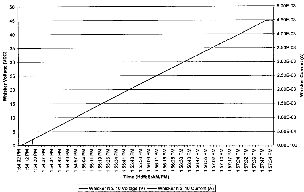
Whisker Breakdown Voltage POC Test Data
