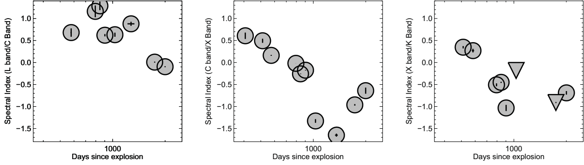
Fig. 3.— Spectral index ( \alpha ) evolution for SN 2006jd between various radio frequencies. The evolution is from positive index towards negative, typical in core-collapse SNe.
