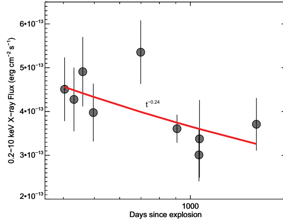
Fig. 7.— X-ray light curve of SN 2006jd. The light curve is best fit with a power law of index -0.24 \pm 0.12 .
