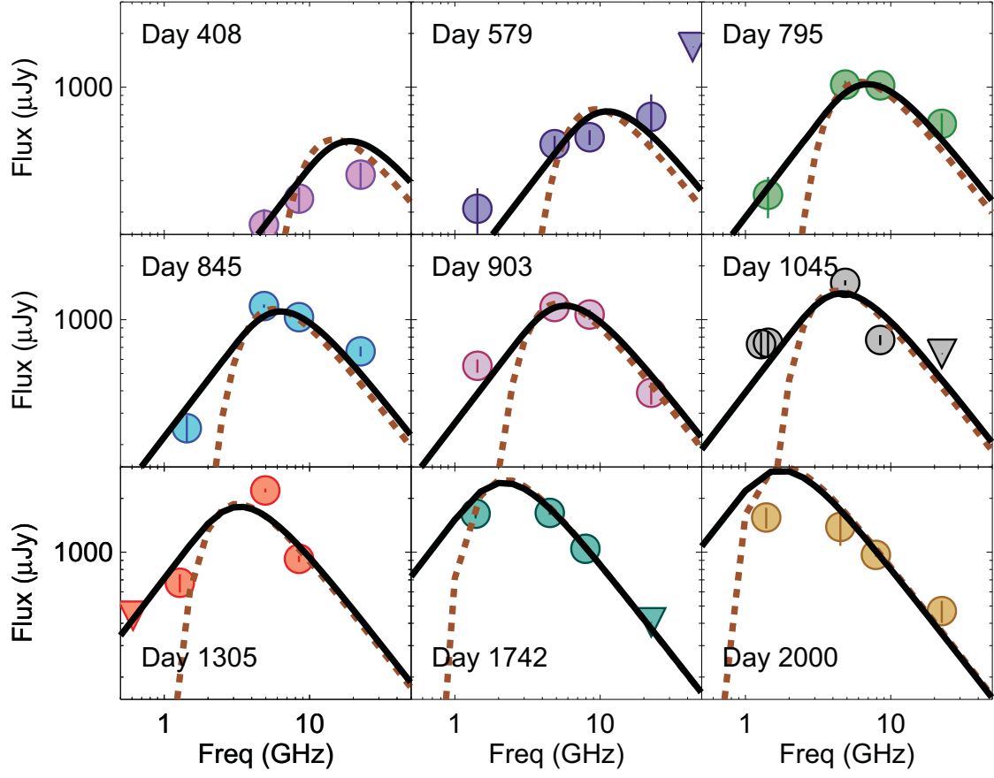
Fig. 2.— Radio spectra of SN 2006jd at 9 epochs. Even though the spectral evolution is slow, a transition from optically thick to an optically thin is clearly seen in the progression of the spectra from early to late epochs. Dashed lines show the best fit external absorption model for s = 1.77 . Black solid lines are the best fit internal absorption model.
