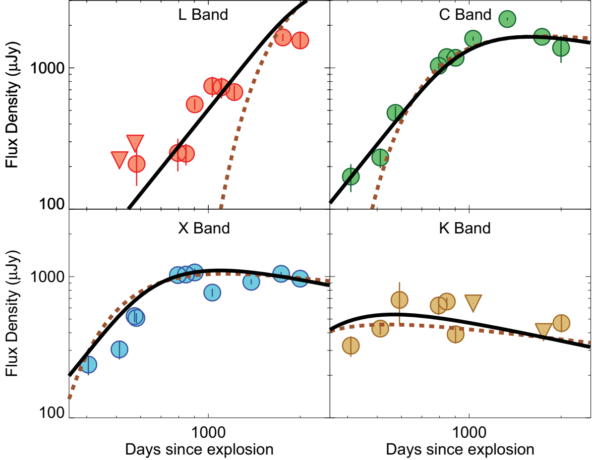
Fig. 1.— Radio light curves of SN 2006 in the 1.4 GHz (L), 5 GHz (C), 8.5 GHz (X) and 22.5 GHz (K) bands. The radio emission in the L band is still rising and the K band emission appears to be in the optically thin phase at late times. The radio emission is making a transition from optically thick to thin in the X and C bands. Here dashed lines show the best fit external absorption model for s = 1.77 . Black solid lines are the best fit internal absorption model.
