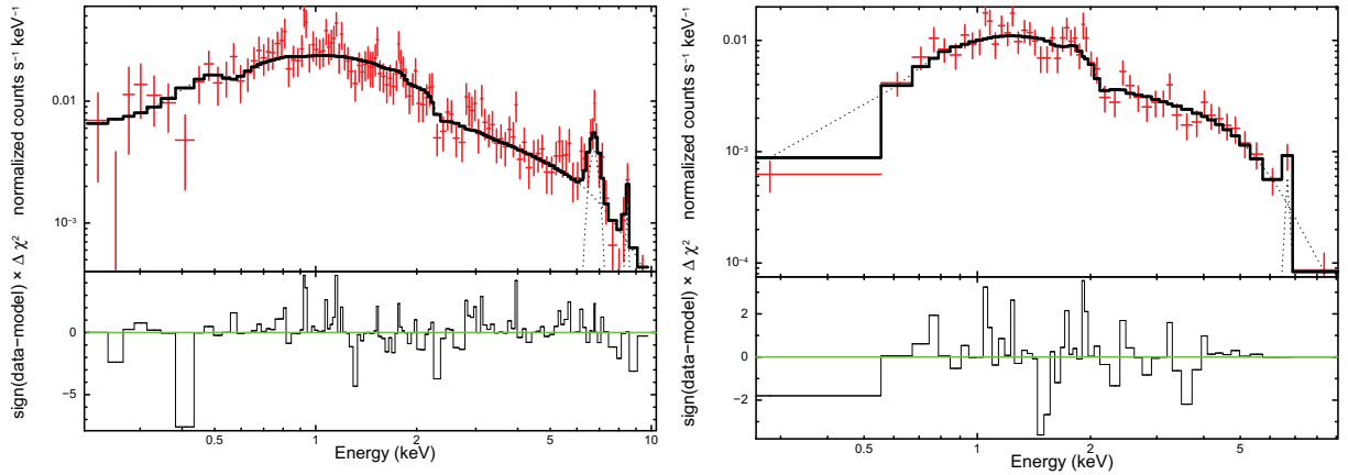
Fig. 6.— The left panel shows the XMM-Newton spectrum of SN 2006jd and the right panel shows the Chandra spectrum of SN 2006jd. Note that the 6.9 keV Fe line is detected in both spectra and has 10% of the total continuum flux (estimated from the XMM-Newton spectra).
