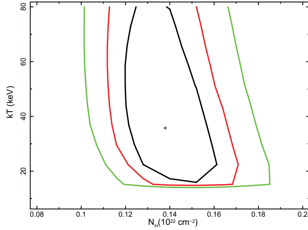
Fig. 4.— Confidence contours of column density versus the X-ray emitting plasma temperature. The column density is well constrained whereas the temperature is not constrained at the higher end.
