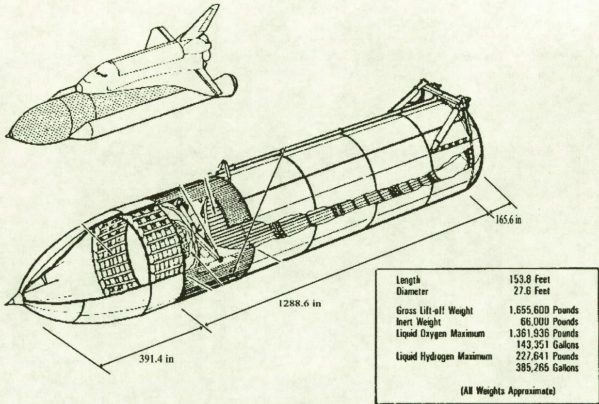
Lightweight External Tank
