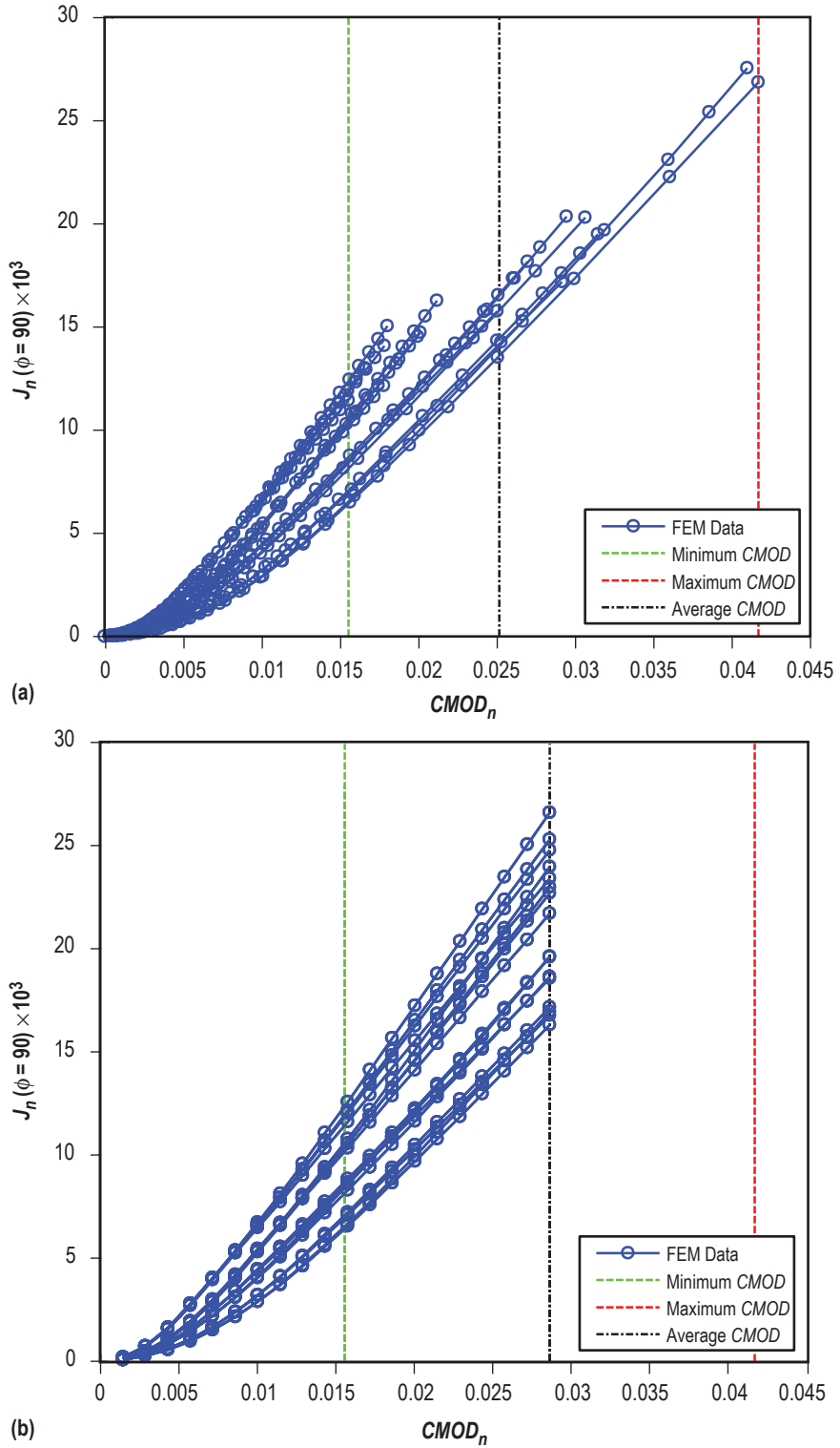
Figure 15. Illustration of (a) effect of truncating the solution space based on the average of the maximum CMOD_n values on the J_n versus CMOD_n results, and (b) dividing the CMOD_n into even increments for J_n versus CMOD_n interpolation.
