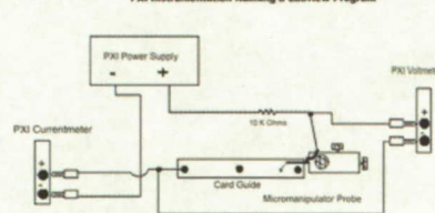
Fig. 3. Schematic diagram for the tin whisker test station instrumentation. Reproduced from [4].
