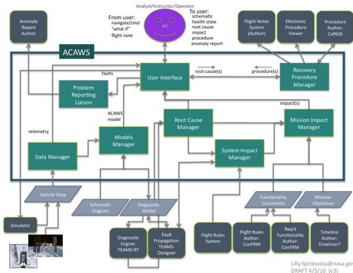
Figure 8: ACAWS high-level architecture.
