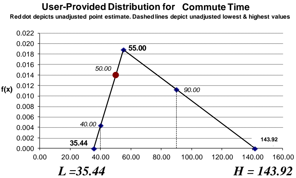
Triangular PDF from Iteration 2
