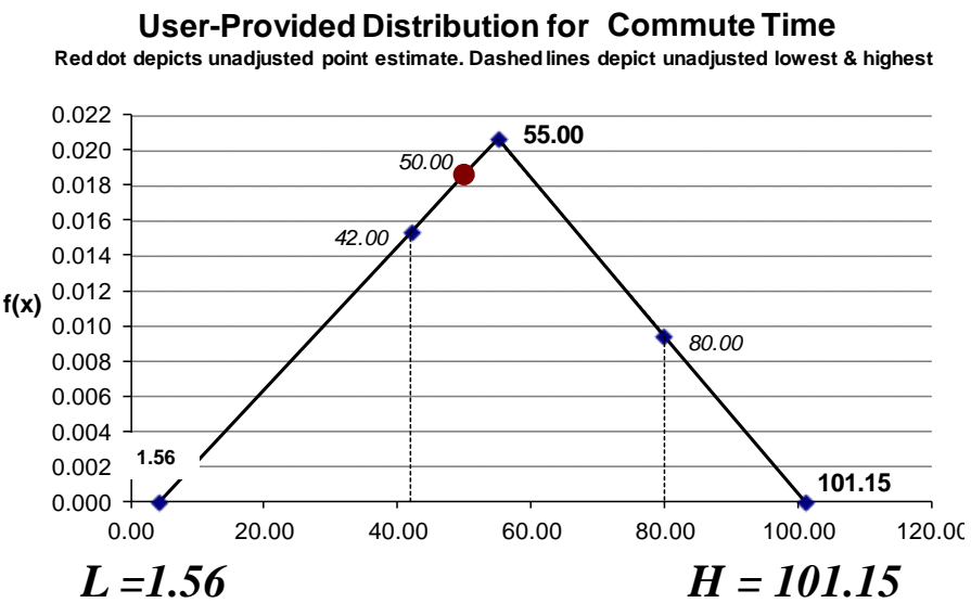
Triangular PDF from Iteration 1
