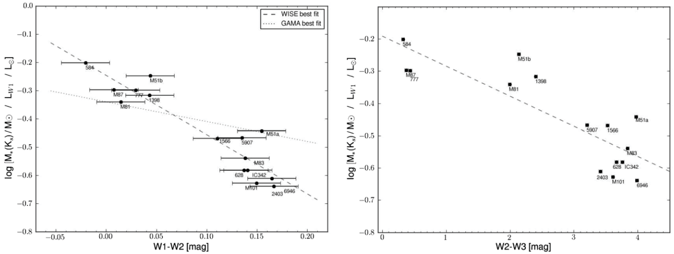
Figure 17. Empirical mass-to-light relation, (M_{\odot}/L_{\odot}) , derived from WISE 3.4 \mu\text{m} in-band luminosity ( W1 - W2 color (left panel), W2 - W3 color (right panel)) and K_s -derived stellar masses using the Zhu et al. (2010) relation (see also Figure 18). The color error bars represent the formal uncertainties (Table 2) and a 1.5% photometric calibration uncertainty. The linear trend (dashed line) is described by Equations (9) and (10). The dotted line (left panel) represents the (M_{\odot}/L_{\odot}) derived for nearby galaxies in the GAMA survey (see the text for details).
