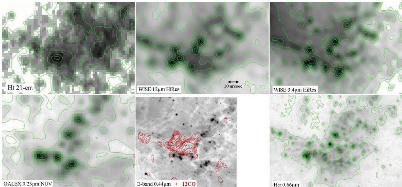
Figure 13. Close-up view of the southwestern bar cusp of M 83, centered on J2000 coordinate 13^{\text{h}}36^{\text{m}}52^{\text{s}}.86 , -29^{\text{d}}52^{\text{m}}55^{\text{s}}.3 . Clockwise starting from left: high spatial resolution 21 cm image (ranging from 0.01 to 0.60 \text{Jy km s}^{-1} ), WISE HiRes 12 \mu\text{m} , WISE HiRes 3.4 \mu\text{m} , \text{H}\alpha , B band (with 12CO contours), and GALEX NUV. The green contours emphasize the gray-scale contrast. Overlaying the B -band image, the red contours are 12CO(1–0) with levels 2, 3, 4, 5, 6, 7, 8, 9 \times 2.3 \text{ Jy km s}^{-1} (Kenney & Lord 1991). At the distance of M 83, the physical scale of 10'' is 213 pc.
