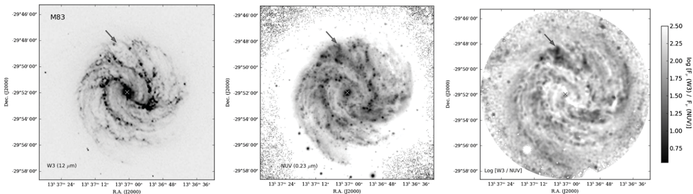
Figure 10. WISE W3 comparison with GALEX NUV of M 83 (NGC 5236). The left panel shows a log-stretch of the WISE W3 image, the middle panel shows a log-stretch of the GALEX NUV image, and the right panel is the flux ratio between the two bands. Dark gray-scale values indicate strong NUV , while light values indicate relatively strong W3 ; e.g., the arrow points to high NUV and low W3 . The nucleus is denoted with a \times symbol.
