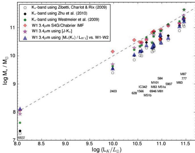
Figure 18. Stellar mass compared to the K_s -band luminosity. The masses are estimated from the K_s , W1 , and W2 luminosities and the M/L relations of Zibetti et al. (2009), Zhu et al. (2010), the S4G/Chabrier IMF relation (Equation (7)), and the M/L relations from this work (Equations (4) and (9); Figure 17). For comparison, the dashed line represents a M/L fraction of unity. (A color version of this figure is available in the online journal.)
