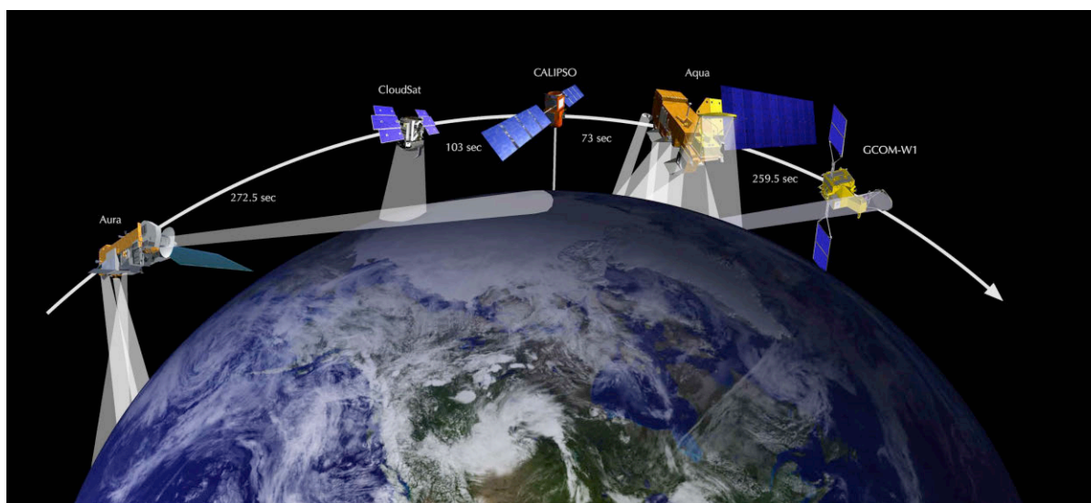
Figure 8. Configuration of the A-Train constellation of satellites as of mid-2012, with GCOM-W in the lead, followed by Aqua, CALIPSO, CloudSat, and Aura. Image credit: Ed Hanka, Angie Kelly, and the A-Train Mission Operations Working Group.
