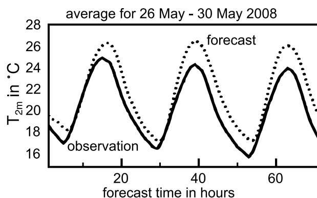
Fig. 1. Predicted T_{2m} as a function of forecast hour compared with measurements for the area of SW-Germany (see area \Omega in Fig. 2). Each day a forecast for three days was simulated; afterwards the results and the corresponding observations were averaged as a function of forecast hour to identify systematic differences between forecast and observation (U. Damrath, DWD, personal communication, 2010).
