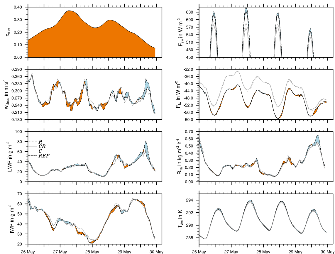
Fig. 13. Time series of dust optical thickness ( \tau_{\text{dust}} ), cloud properties ( w_{\text{cloud}} , LWP, and IWP), precipitation rate ( R_{1h} ), net surface radiation fluxes ( F_{\text{sw}} and F_{\text{lw}} ), and temperature ( T_{2m} ) averaged for domain D1. Solid lines are results from simulation C, dashed lines are results from simulation REF, solid gray lines are results from simulation CR, and dotted gray lines from simulation R.
