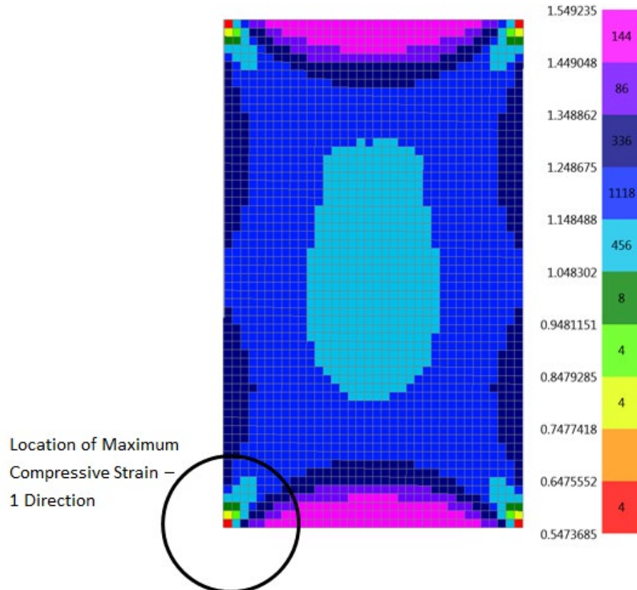
Figure 38.—HyperSizer margin of safety plot for core crimping, core crushing, facesheet wrinkling, and facesheet dimpling.
