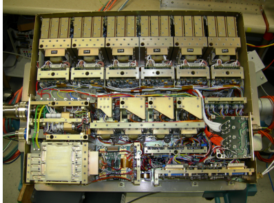
Figure 2 – NEXT PPU developmental unit
