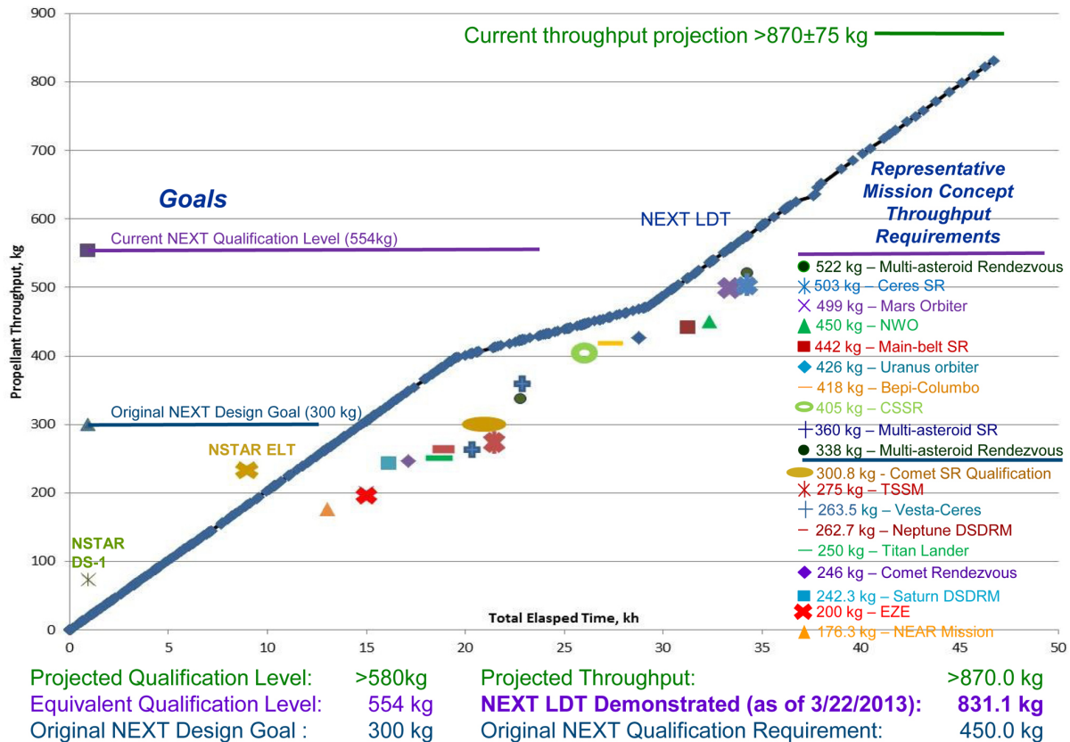
Figure 1 – Next Thruster Total Throughput versus Representative Mission Requirements
