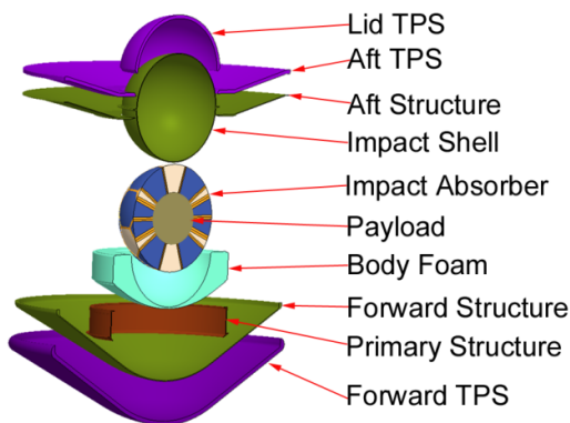
Figure 7 – Basic MMEEV architecture
