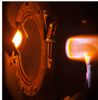
Figure 11 – Space Environmental Effects Testing – simulated micrometeoroid impact followed by arc jet testing
