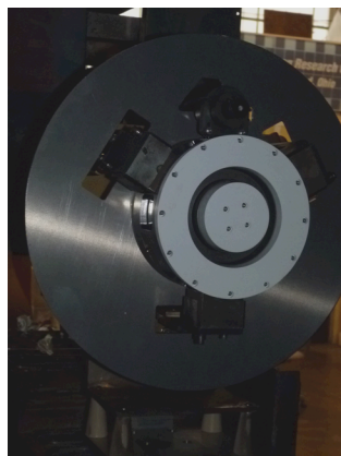
Figure 4 – HIVHAC thruster Engineering Development Unit (EDU)
