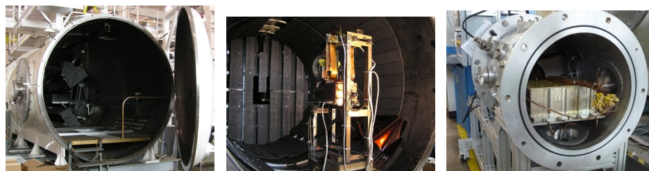
Figure 5 – HIVHAC EDU Thruster and Colorado Power SBIR PPU undergoing performance testing.
