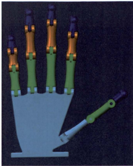
Figure 3. Skeleton of robotic hand
