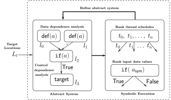
Figure 1: Overview of the abstraction-guided symbolic execution technique
