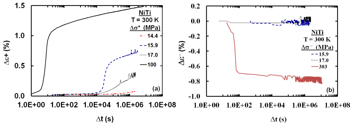
Figure 4.—The nature of the creep curves immediately after (a) a stress increase and (b) a stress decrease. The values of \Delta\varepsilon and \Delta t are defined with respect to the point at which the stress change was performed. The + and – superscripts indicate increase and decrease, respectively. The curves for \Delta\sigma^+ = 14.4, 15.9 and 17.0 MPa do not start at \Delta t = 0 since the first data acquisition was acquired 10 s after the stress increase.
