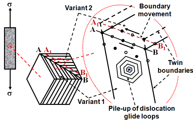
Figure 13.—Phenomenological model showing the possible role of dislocation pile-ups in martensitic variant 1, which results in the development of shear stresses in the boundary regions so that the boundary between variants 1 and 2 moves from AB to A_1B_1 , and the corresponding detwinning of variant 2.
