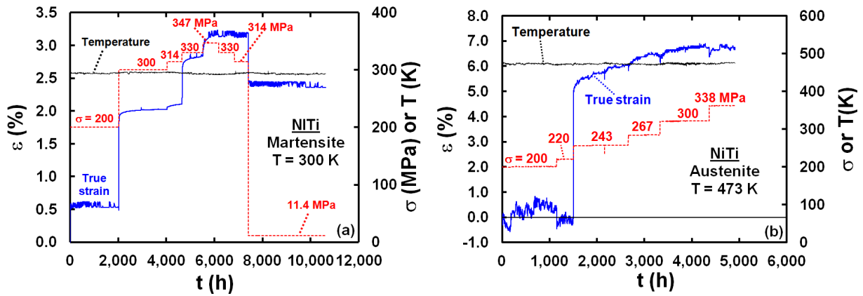
Figure 3.—Creep strain versus time plots for (a) NiTi martensite deformed at 300 K and (b) NiTi austenite deformed at 473 K showing the effect of stress changes on the nature of the creep curves. Insignificant creep was observed below 200 and 220 MPa for martensite and austenite, respectively.
