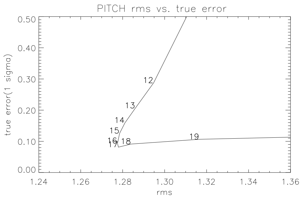
Figure 5.8: True errors versus rms values of EKF estimation (arcsecond)
