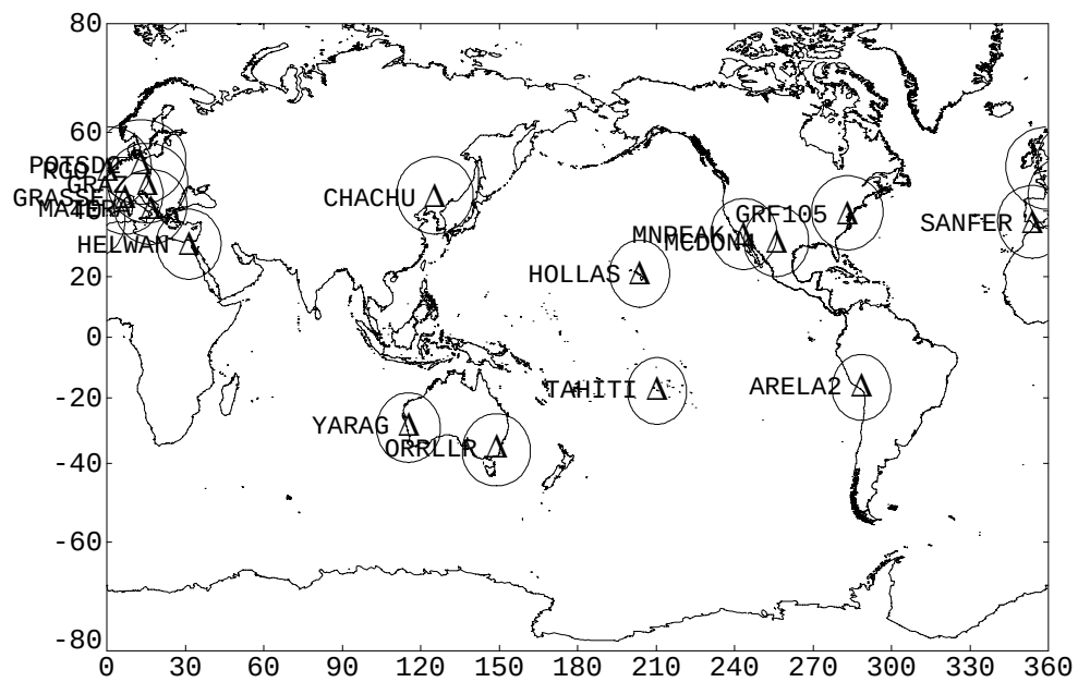
Figure 3. SLR Stations Tracking ICESat/GLAS (20 degree Elevation Masks)
