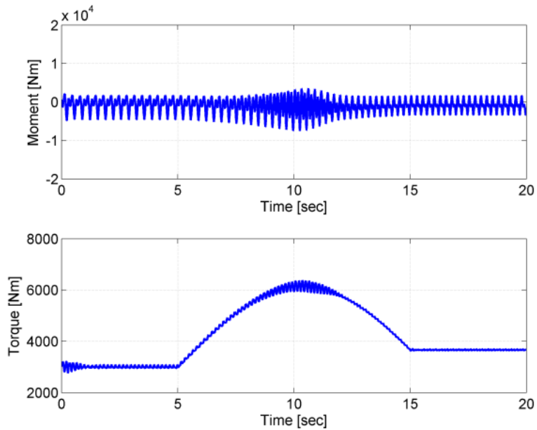
Figure 2.27.—Lagwise root bending moment and rotor torque with 5 percent critical damping.
