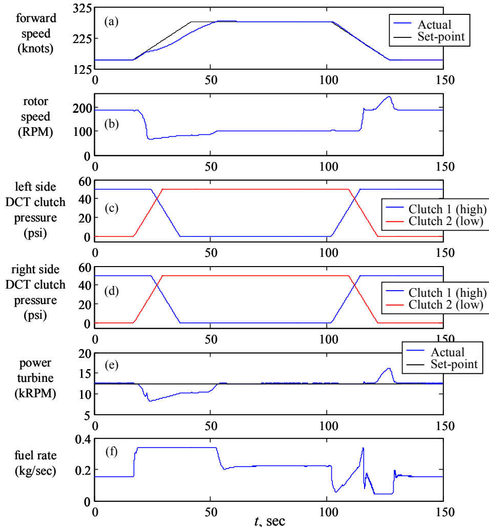
Figure 7.24.—Variable forward cruise PSC downshift/upshift; (a) forward speed, (b) rotor speed, (c) left DCT shift commands, (d) right DCT shift commands, (e) power turbine speeds, (f) fuel rates.
