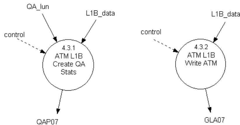
Figure 11-8 ATM L1B QA Statistics and WriteATM Subprocesses
