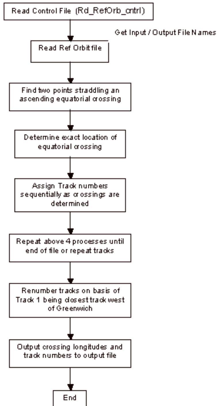
Figure 14-1 Process Flow Diagram
