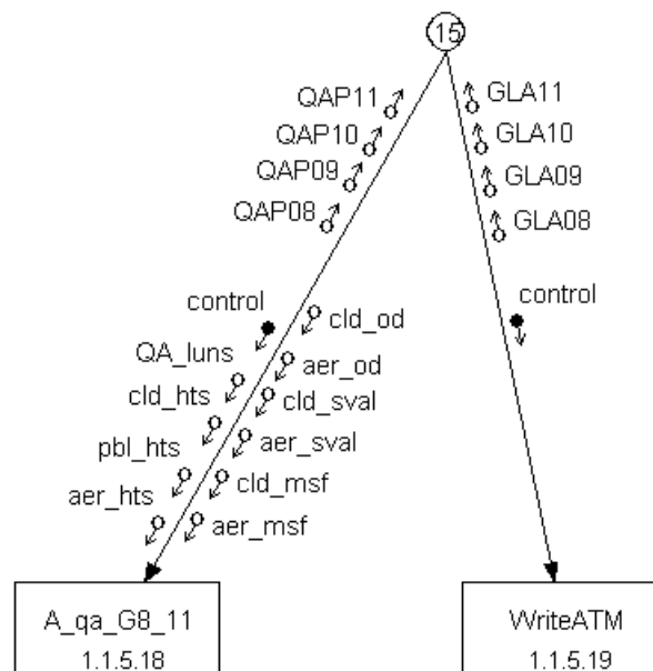
Figure 11-19 L2 QA Statistics / Write ATM Modules
