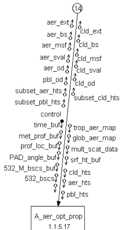
Figure 11-18 ATM Optical Properties Module
