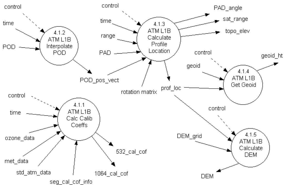
Figure 11-6 ATM L1B Calculate Calibration Coefficients, Profile Locations, and DEM Subprocesses
