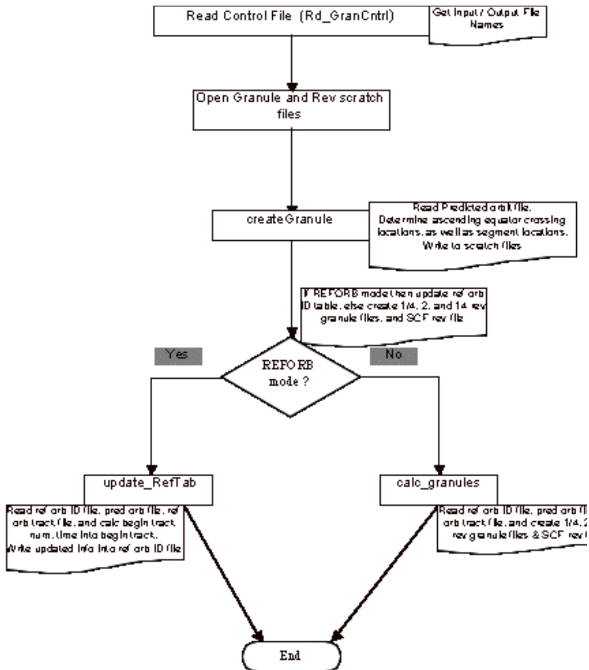
Figure 15-1 Process Flow Diagram
