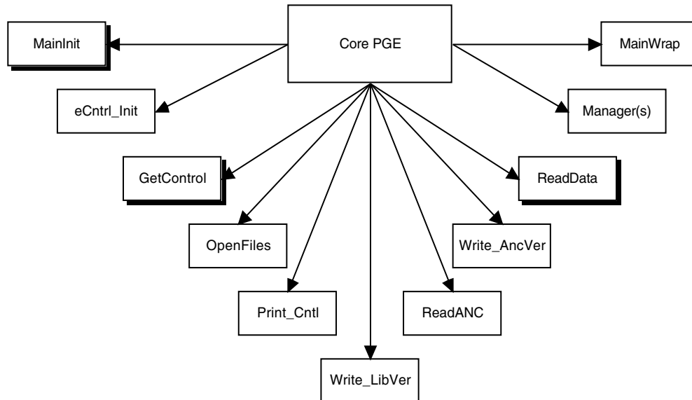
Figure 6-1 Top-Level Structure Chart
