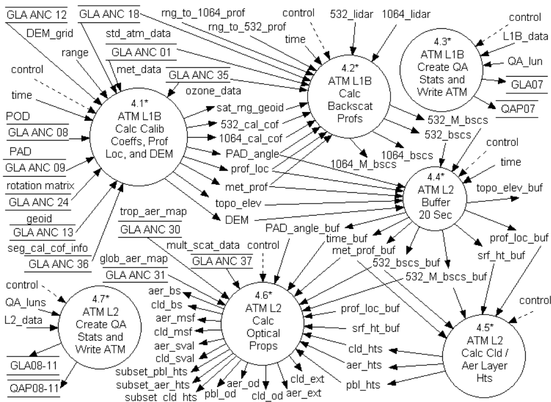
Figure 11-5 Atmosphere Subsystem Processes
