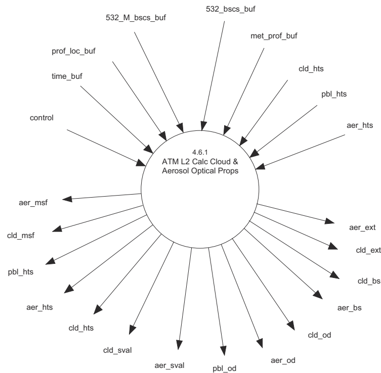
Figure 11-11 Atmosphere Subsystem: Optical Properties Subprocesses
