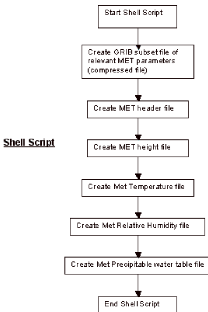
Figure 13-2 Process Flow Diagram: Shell Script
