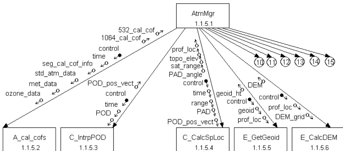
Figure 11-13 ATM Calibration Coefficient / Profile Location / DEM Modules
