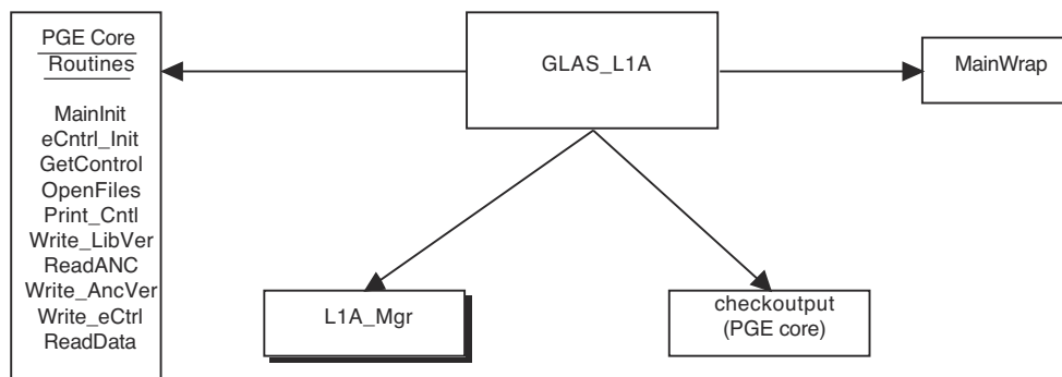
Figure 9-1 GLAS_L1A Structure Chart
