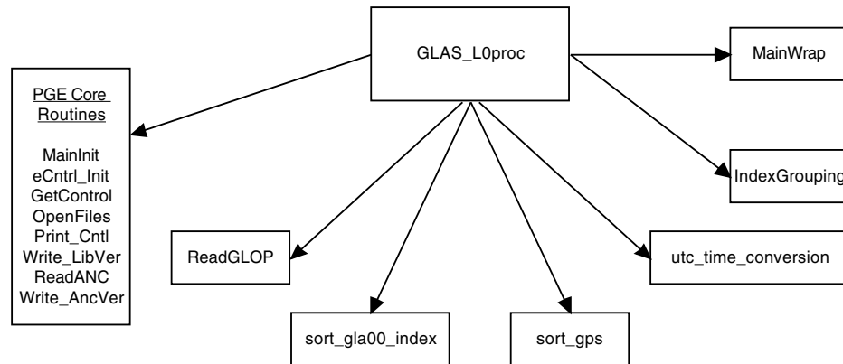
Figure 8-1 GLAS_L0proc Structure Chart
