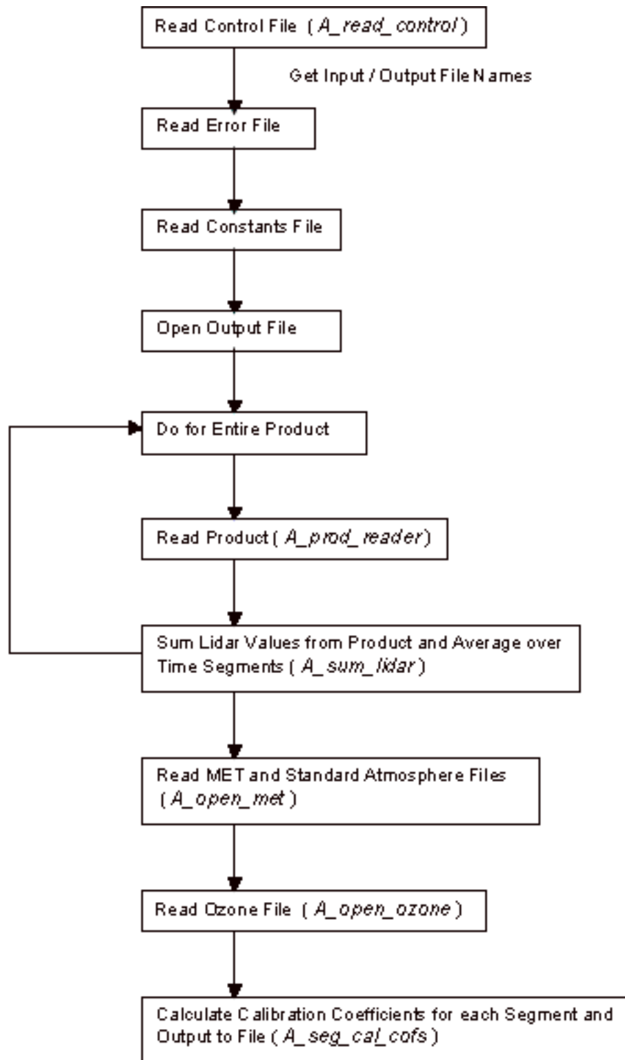
Figure 16-1 Process Flow Diagram
