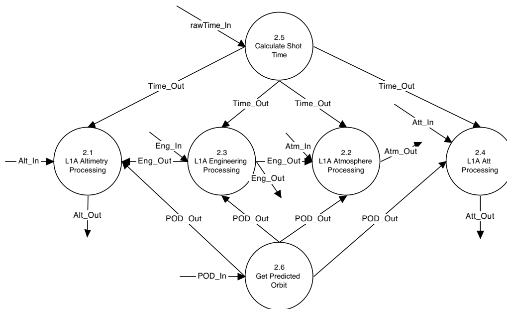
Figure 9-4 Level 1A Computations
