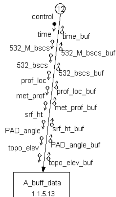
Figure 11-16 ATM 20 sec Buffering Module
