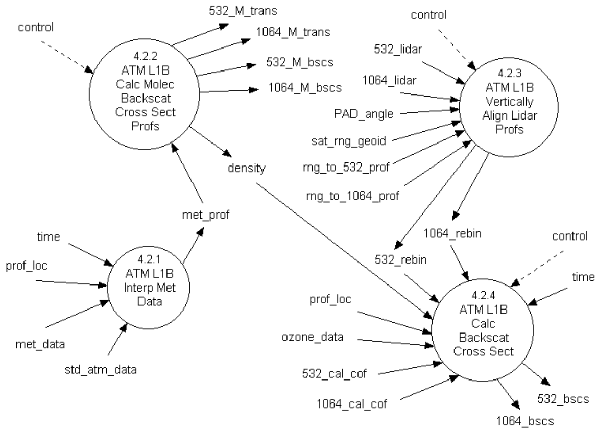
Figure 11-7 ATM L1B Backscatter Subprocesses
