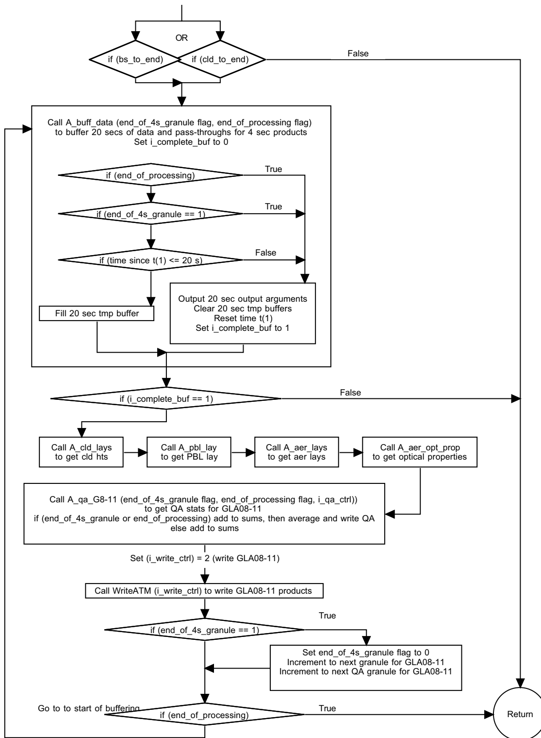
Figure 11-4 ATM Manager - Part 2
