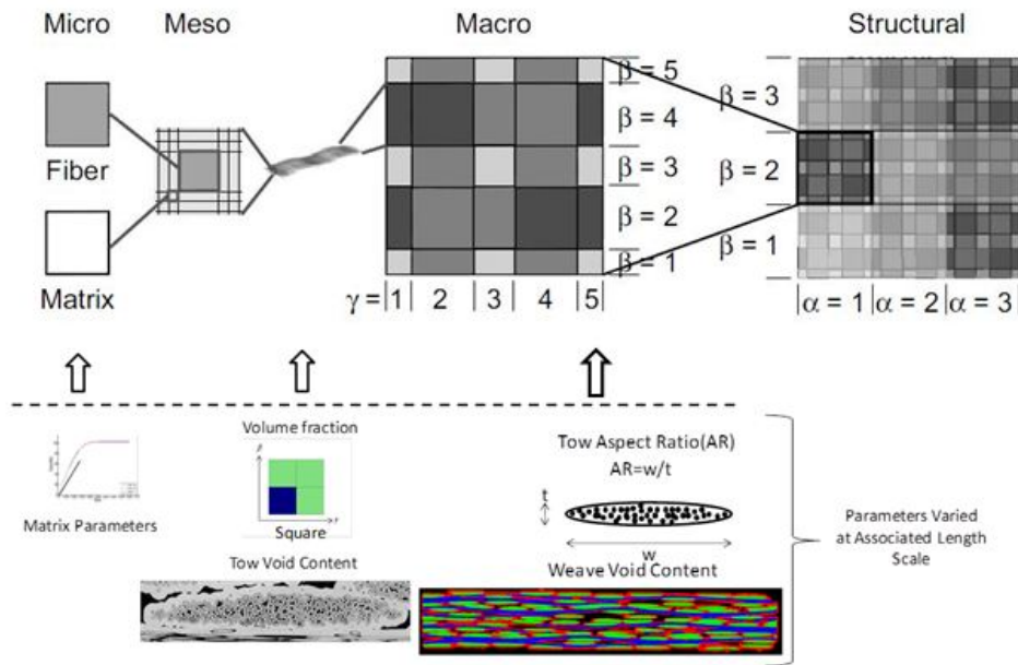
Figure 4.—Multiscale methodology with architectural effects being varied shown at three length scales considered. Actual micrographs are complements of P. Bonacuse, NASA GRC, 2010.
