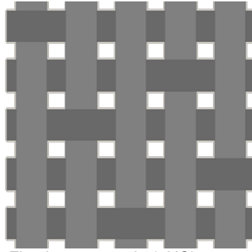
Figure 3.—Five harness satin (5HS) macroscale RUC.
