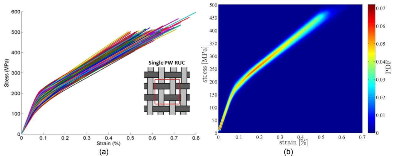
Figure 17.—Stochastic simulation of a PW composite at the macroscale; (a) 638 individual cases; and (b) multivariate probability density function tensile curve.
