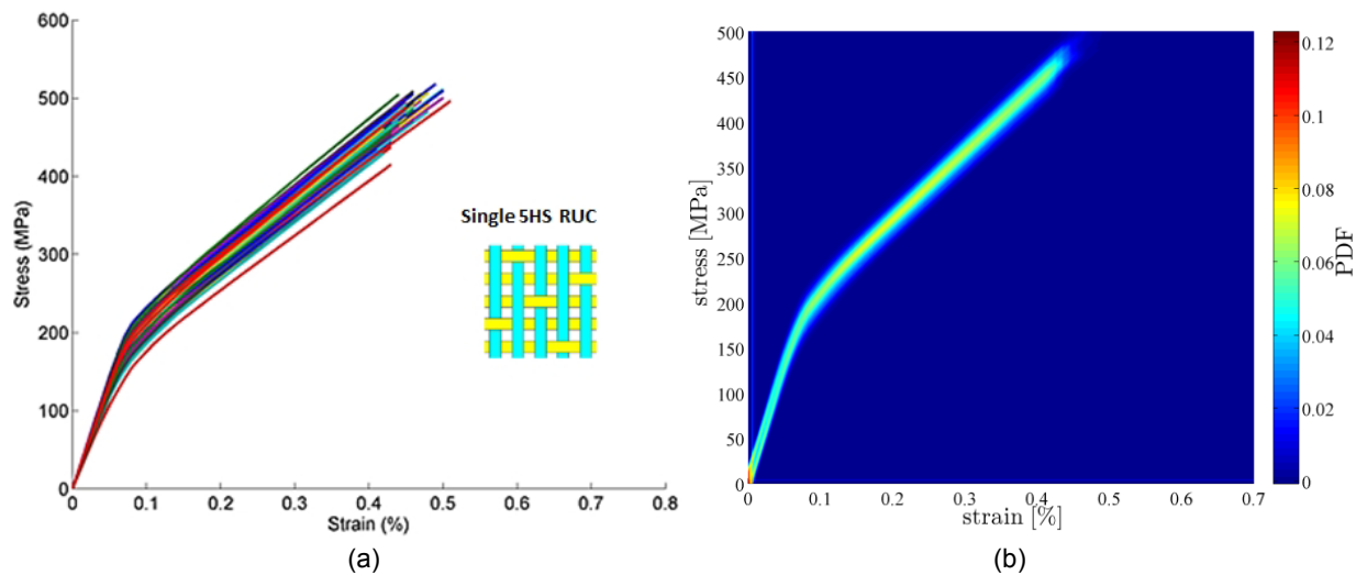
Figure 16.—Stochastic simulation of a 5HS weave composite at the macroscale; (a) 150 individual cases; and (b) multivariate probability density function tensile curve.
