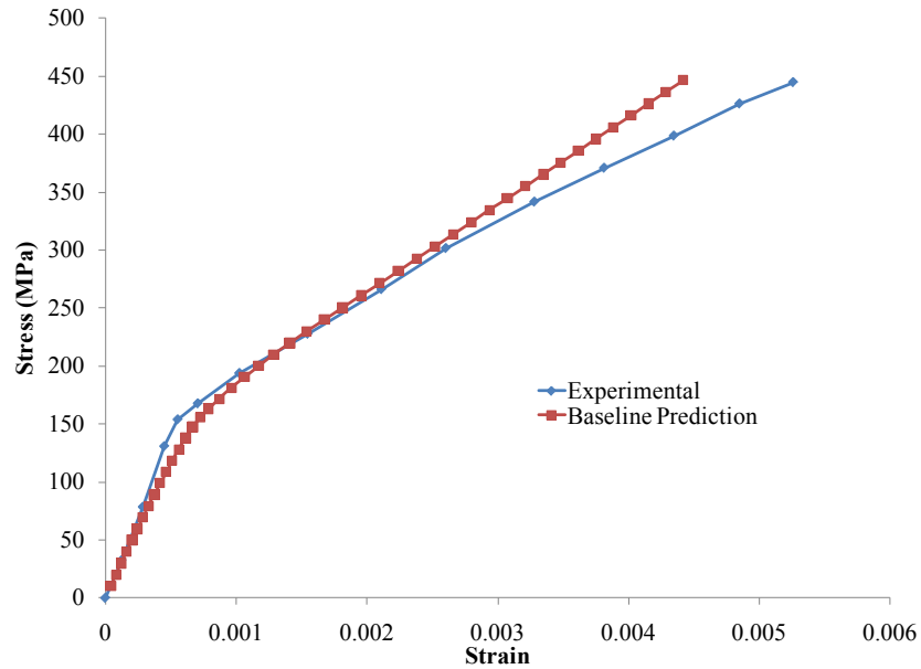
Figure 11.—Typical experimental response curve (Refs. 10 and 11).
