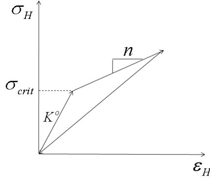
Figure 5.—Schematic showing bulk moduli change as function of triaxial strain. Note K^0 represents the initial bulk modulus.
