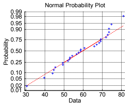
Figure 18.—Normal probability plot of out-of-plane modulus for 5HS composite.
