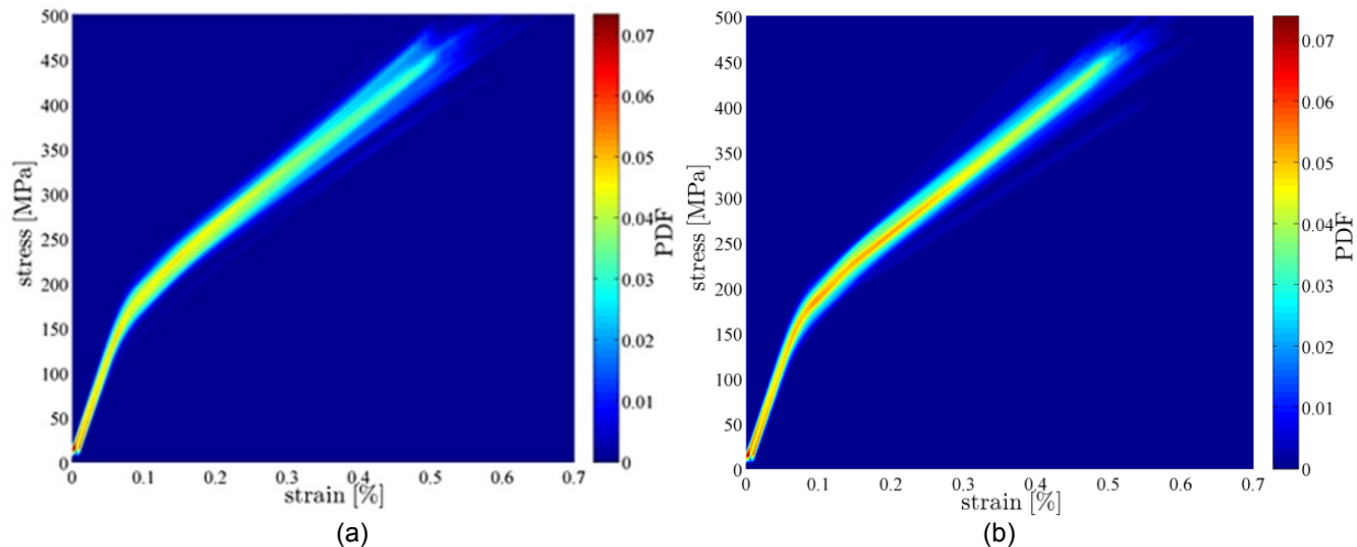
Figure 19.—Monte Carlo simulations at the structural scale for a plain weave composite using, (a) 2x2 and (b) 3x3.
