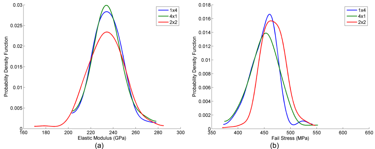
Figure 21.—Distributions of (a) elastic modulus (b) failure stress; given the same number of random variables but analyzed using a 4x1 (parallel), 1x4 (series) and combination plain weave idealization.
