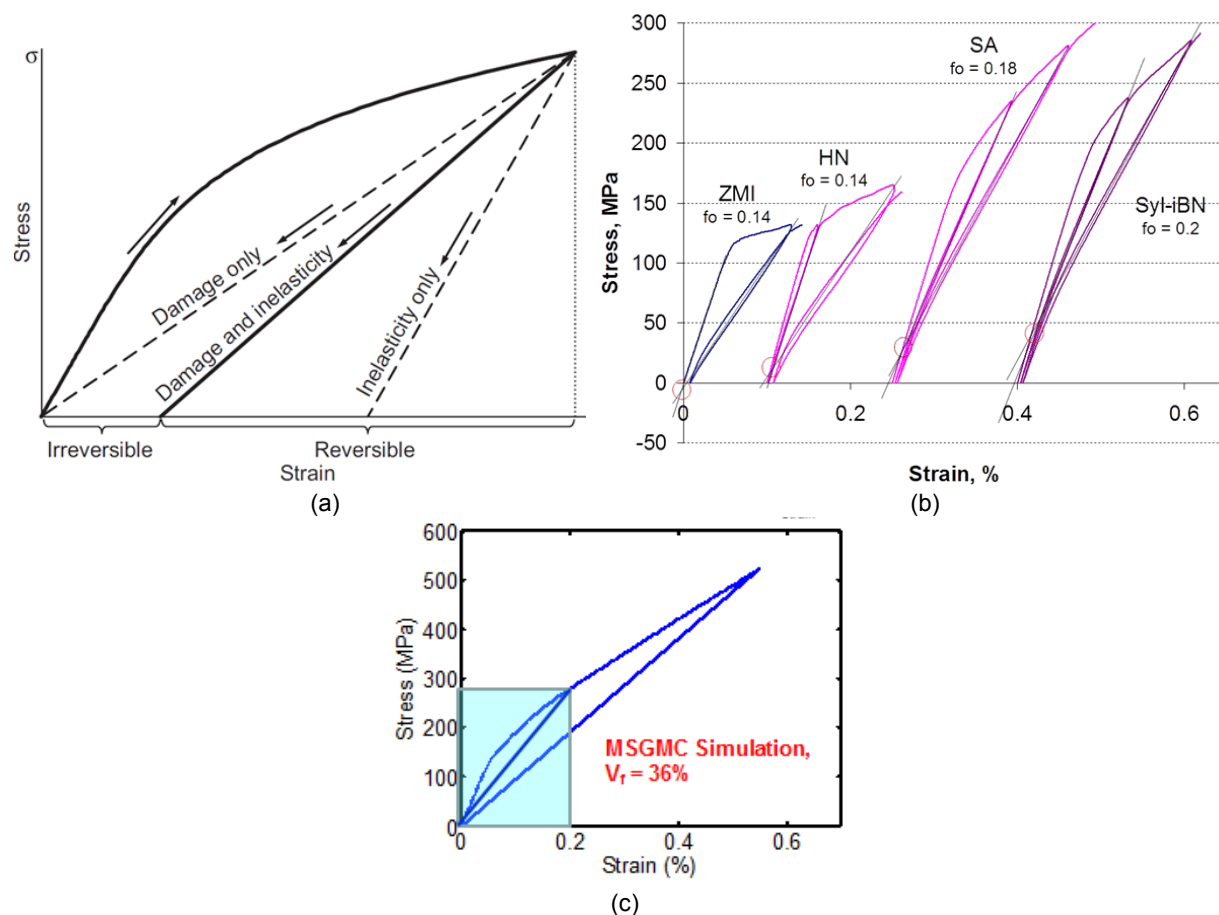
Figure 14.—(a) Schematic of loading/unloading of a given material; (b) Experimental results (Ref. 12); and (c) Simulated tensile loading and unloading response for the localized void model of a 5HS weave.
