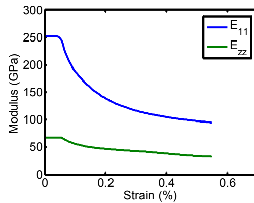
Figure 12.—Concurrent degradation of in plane and out of plane modulus as a function of tensile strain.
