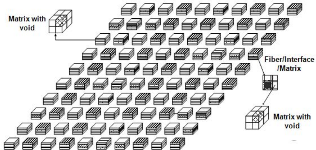
Figure 7.—Discretized five-harness satin subcell configuration, with each block representing a given group.
