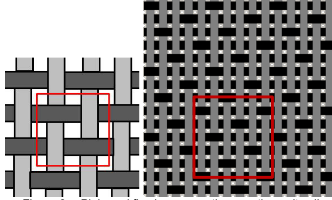
Figure 6.—Plain and five harness satin repeating unit cell.
