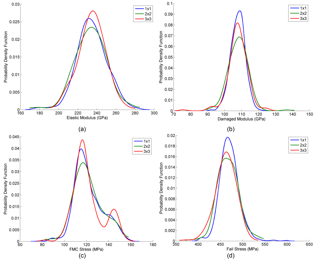
Figure 20.—Distributions of salient stress-strain curve parameters; (a) elastic modulus; (b) damaged modulus; (c) first matrix cracking stress; and (d) failure stress.
