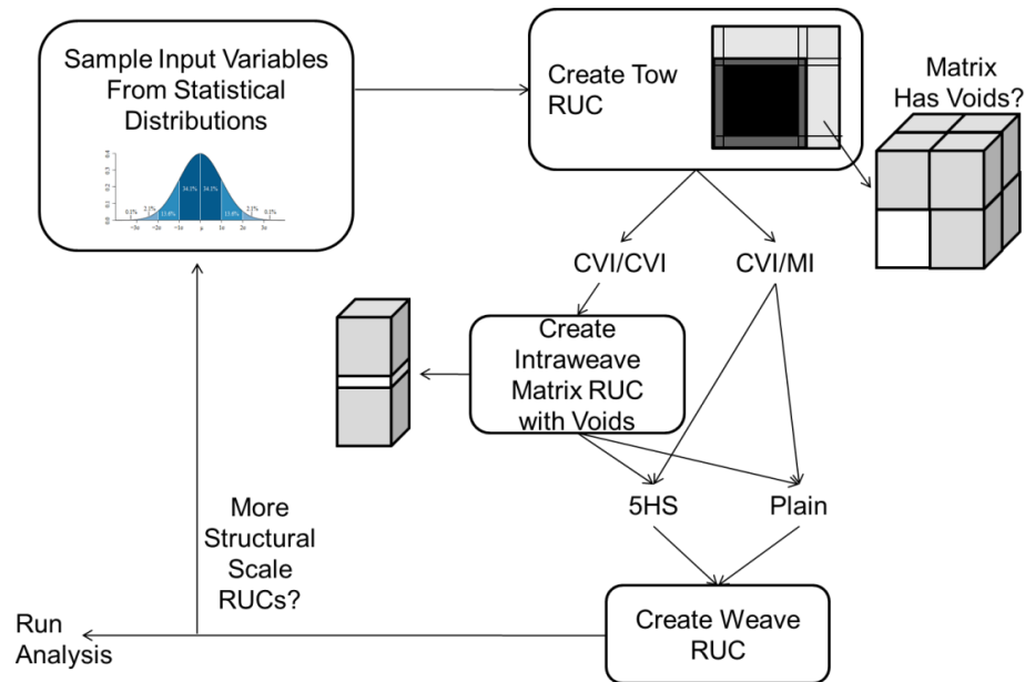
Figure 15.—Statistical procedure.
