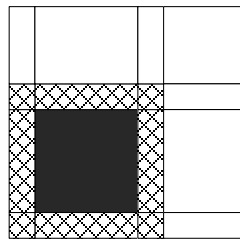
Figure 9.—Fiber tow bundle RUC.
