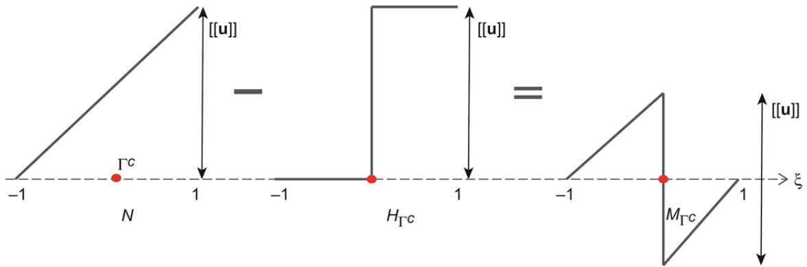
Figure 18.—Construction of discontinuous multiscale shape function M_{\Gamma^c} in one dimension from continuous basis function N and Heaviside function H_{\Gamma^c} . [[\mathbf{u}]] is displacement discontinuity and \Gamma^c is crack surface (in red).
