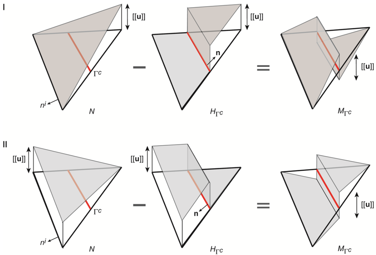
Figure 19.—Two possible constructions of discontinuous multiscale shape function M_{\Gamma^c} in two dimensions from continuous basis function N and Heaviside function H_{\Gamma^c} . [[\mathbf{u}]] is displacement discontinuity, \Gamma^c is crack surface (in red), and \mathbf{n} is normal to crack path in direction of desired jump in displacement.
