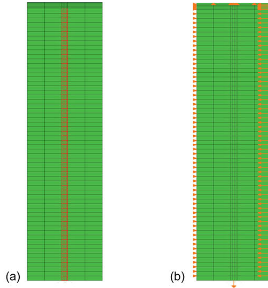
Figure 45.—Finite element model geometry. (a) Quadrilateral elements mesh. (b) Boundary conditions.
