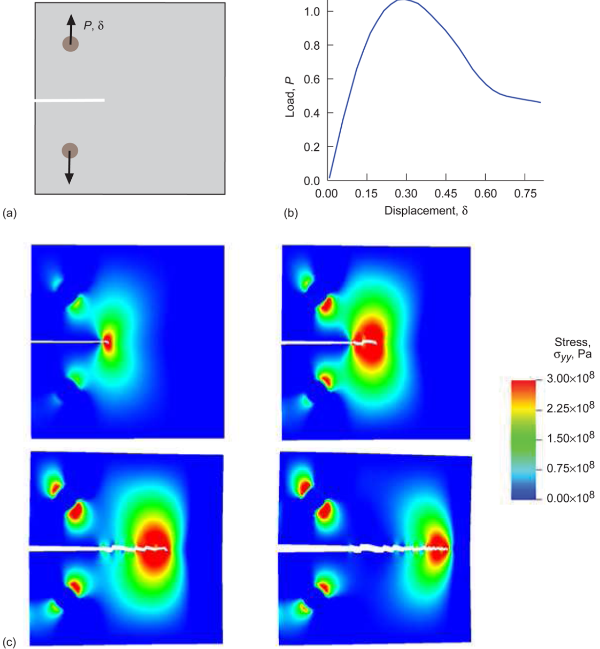
Figure 26.—Mixed-mode crack propagation in symmetrically loaded compact tension specimen (CTS) (with load P and displacement \delta ). (a) CTS. (b) Corresponding load-displacement response; P and \delta values have been normalized with fixed reference values. (c) Evolving opening stress \sigma_{yy} magnitude with crack growth.
