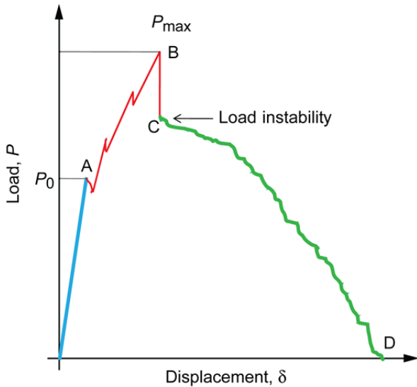
Figure 43.—Fiber-pullout load-displacement response. A: Crack initiation, A–B: Crack propagation and contact friction, B–C: Load instability, and C–D: Fiber pullout.
