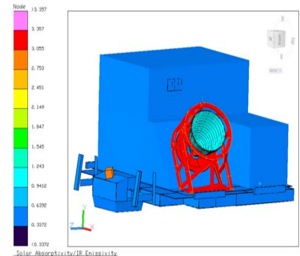
Solar Absorptivity/ IR Emissivity
