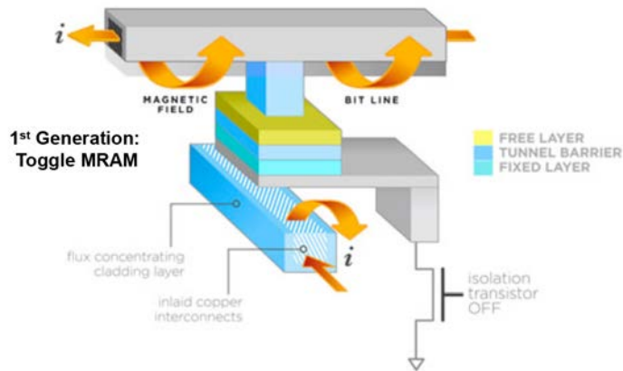
Figure 3.2-5. "Toggle" MRAM 1T/1MTJ memory cell [15].
