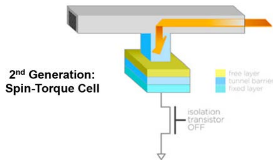
Figure 3.2-6. ST-MRAM 1T/1MTJ memory cell [17].
