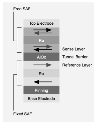
Figure 3.2-1. The Everspin proprietary 10-layer MTJ [12].
