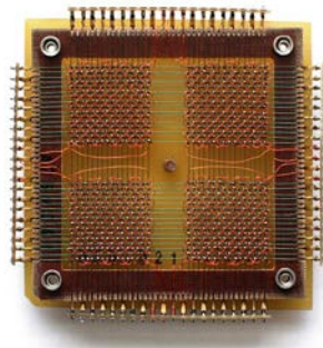
Figure 2.1-1. Magnetic core memory used in the 1950s, the first magnetic memory. The memory shown here stored 32x32 (1024) bits of data [1].
