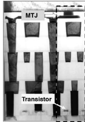
Figure 3.2-2. Cross sectional view of Everspin MTJ [13].
