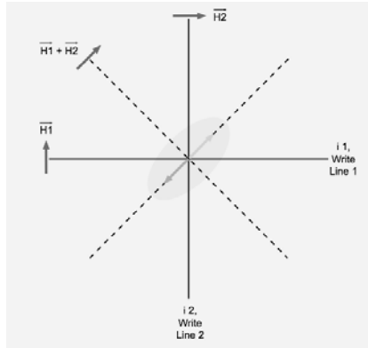
Figure 3.2-3. Schematic of toggle MRAM bit [12].
