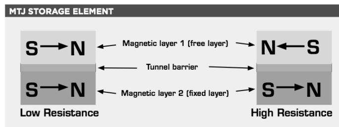
Figure 2.43-1. The MTJ has low electrical resistance when the magnetic moments of the ferromagnetic layers are parallel, and high electrical resistance when they are antiparallel [8].
