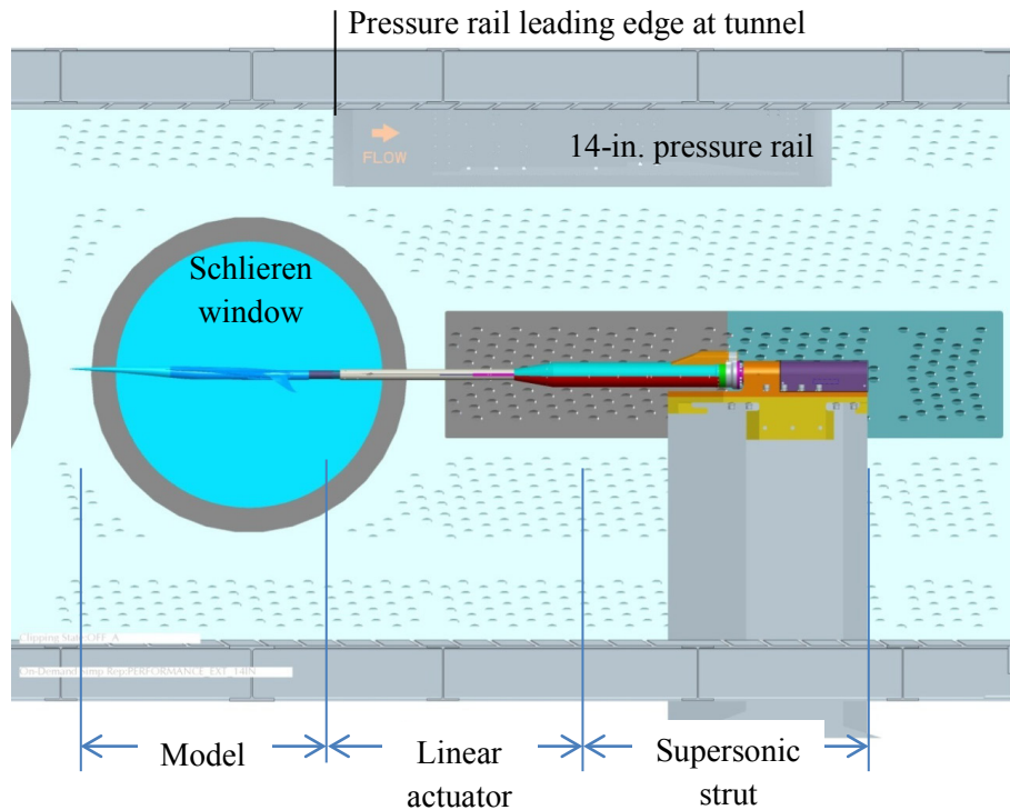
Figure 1.—Wind tunnel layout for the sonic boom model in the 8×6 SWT.
