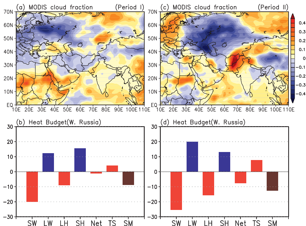
FIG. 6. (top) Distribution of MODIS cloud fraction anomalies for periods (a) I and (c) II. Anomalies were computed based on the climatology of March 2000–February 2010. (bottom) Area mean MERRA shortwave (SW) and longwave (LW) radiation, latent heat (LH) and sensible heat (SH) flux, net flux (Net) at the surface, and soil moisture (SM) averaged over western Russia (45–65°N, 30–60°E) for periods (b) I and (d) II. Units are \text{W m}^{-2} for fluxes and fraction ( \times 100 ) for soil moisture. Red (blue) color denotes warming (cooling) of the land surface.
