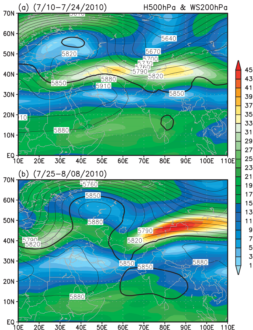
FIG. 3. Spatial patterns of 500-hPa geopotential height (contours) and 200-hPa wind speeds (colors) during periods (a) I and (b) II.
