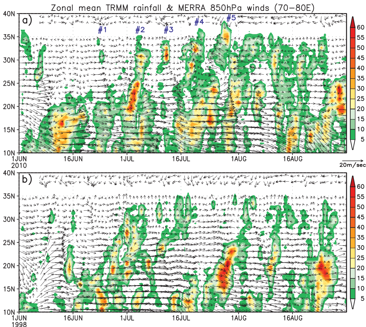
FIG. 8. Latitude–time cross section of TRMM daily rainfall ( \text{mm day}^{-1} ) and MERRA winds at 850 hPa averaged between 70° and 80°E for (a) 2010 and (b) 1998.
