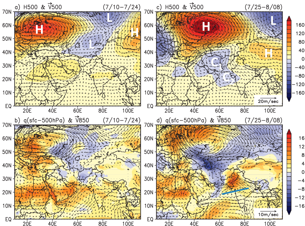
FIG. 4. Spatial patterns of (a) 500-hPa geopotential height (m) and wind anomalies during period I, (b) 850-hPa wind and precipitable water (mm) below 500 hPa during period I, (c) 500-hPa geopotential height and wind anomalies ( \text{m s}^{-1} ) during period II, and (d) anomalous 850-hPa wind and precipitable water during period II. Centers of the blocking high (H) and low (L) and the midtropospheric cyclones ( C_1 and C_2 ) are marked. Thick line in Fig. 4d indicates the location of monsoon front. Anomalies were computed based on the climatology of 1979–2009.
