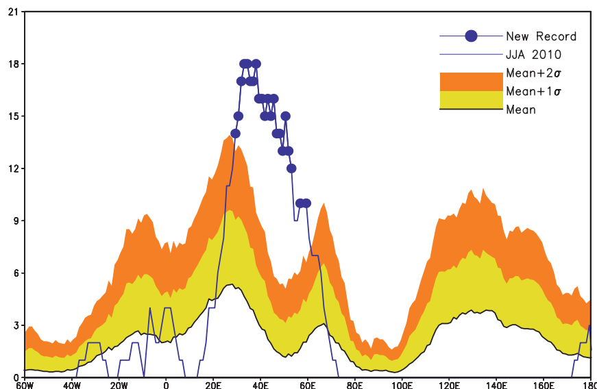
FIG. 2. Number of blocking events at each longitude during boreal summer (JJA) for 2010 (blue) and climatological mean distribution of atmospheric blocking from 1979 to 2009. Yellow and orange layers indicate 1 and 2 std dev from mean, respectively. Blue dots indicate longitudinal locations where the blocks in 2010 were at an all-time high since 1979.
