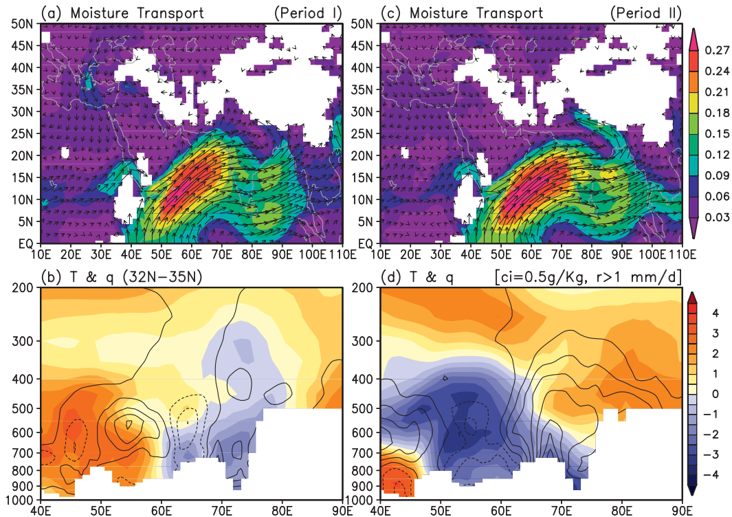
FIG. 7. (top) Distribution of vertically integrated moisture transport between surface to 850 hPa for periods (a) I and (c) II. Amplitude is shown in shading. (bottom) Composite longitude–height cross section of temperature (shading) and moisture (contour) anomalies averaged between 32° and 35°N during rainy days (rain rate > 1 mm day -1 ) in northern Pakistan (see Fig. 1) for periods (b) I and (d) II.
