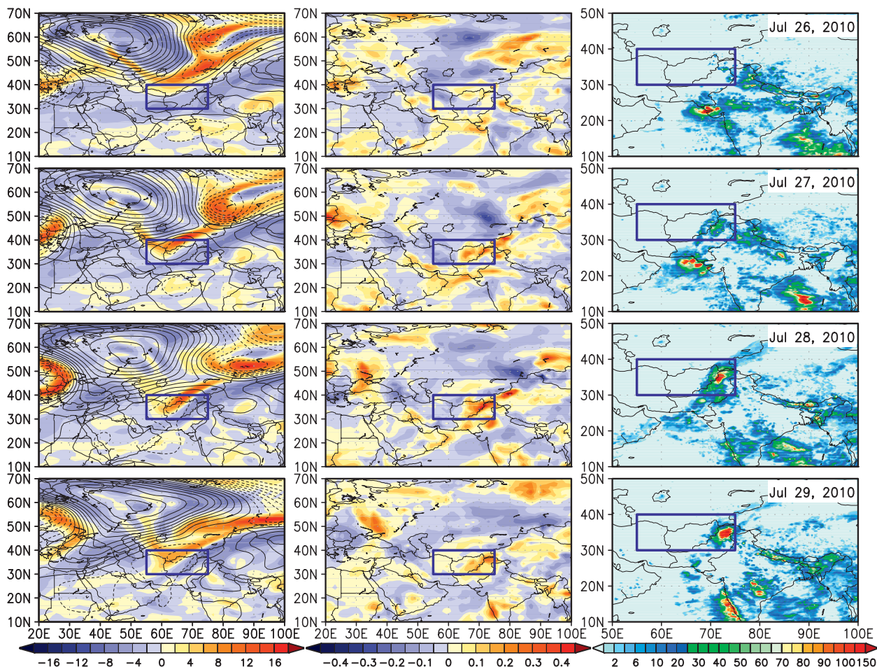
FIG. 5. Daily sequence during 26–29 Jul of MERRA (left) 300-hPa vorticity ( 10^{-5} \text{ s}^{-1} ) and 500-hPa height (m) anomalies, (middle) 500-hPa vertical velocity ( \text{Pa s}^{-1} ), and (right) TRMM rainfall (mm). The target region of northern Pakistan and vicinity to the west is indicated by the rectangle. The sign of the vertical velocity (middle) is reversed so that positive value (red) indicates ascending motion.
