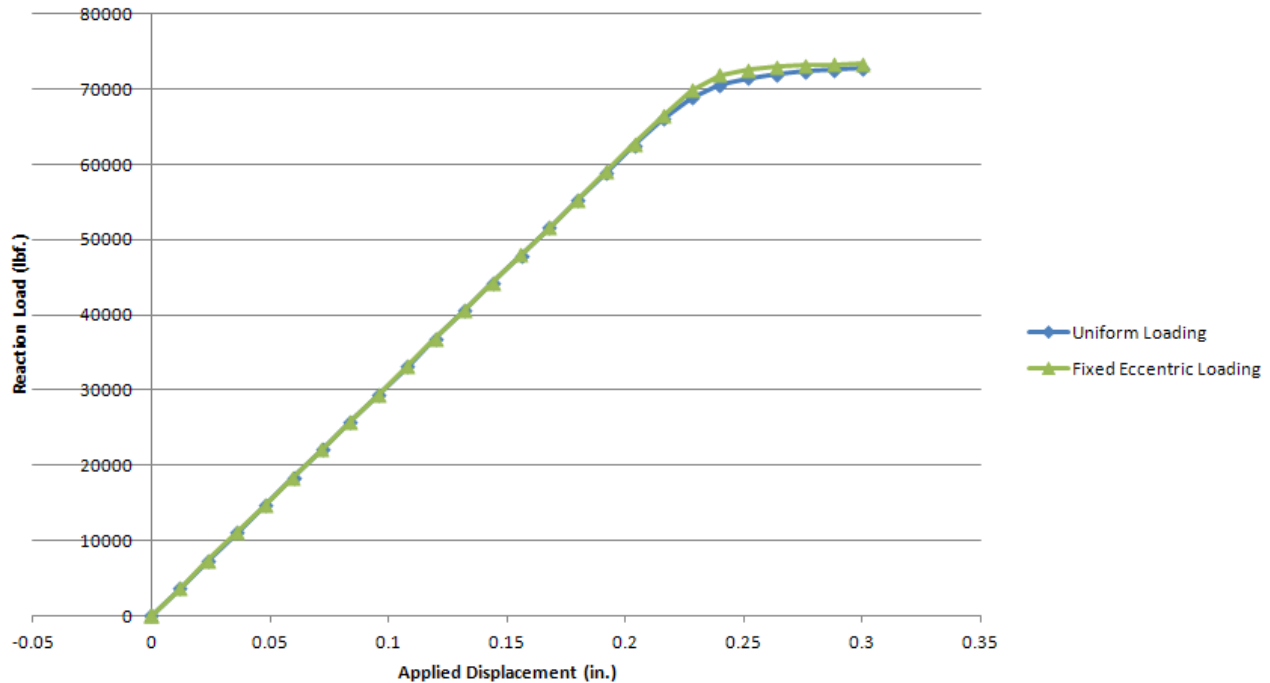
Figure 50.—Reaction load versus applied displacement with uniform applied displacement and simulated eccentric applied displacement. (Fix legend/scale lines on left side of plot.)
