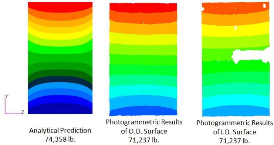
Figure 29.—Post-buckling Y (in-plane) displacement comparison.
