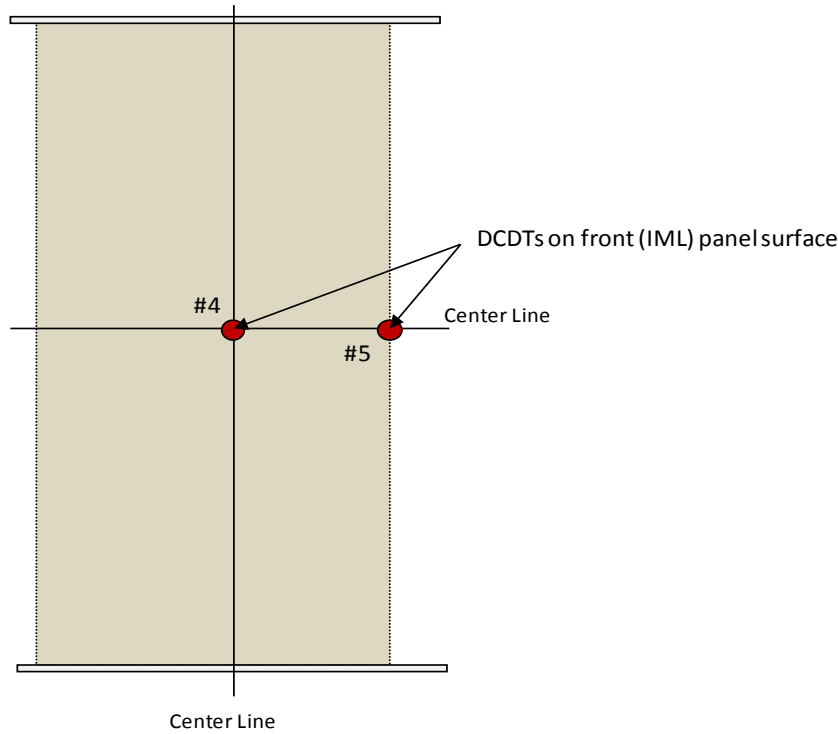
Figure 7.—Location of DCDT's on front (IML) surface of Panel B-1 and back (OML) surface of Panel B-2.
