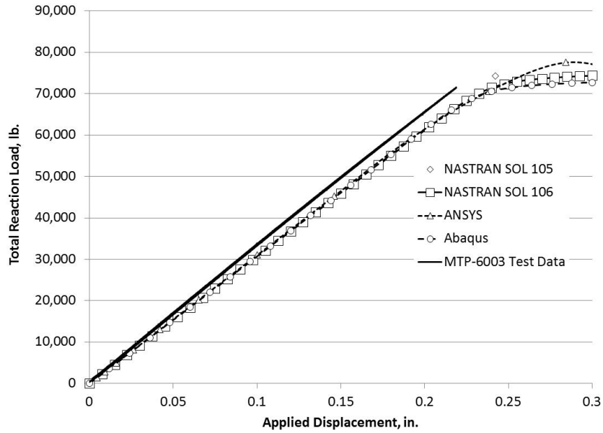
Figure 12.—Total Panel B-1 reaction load versus end shortening for all analyses.
