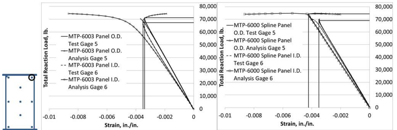
Figure 21.—Load/strain plot for MTP-6003 and MTP-6000 Approximated Spline Gages 5 and 6, upper, right side, even numbers on I.D. Analysis obtained from MSC/NASTRAN, Sol 106.
