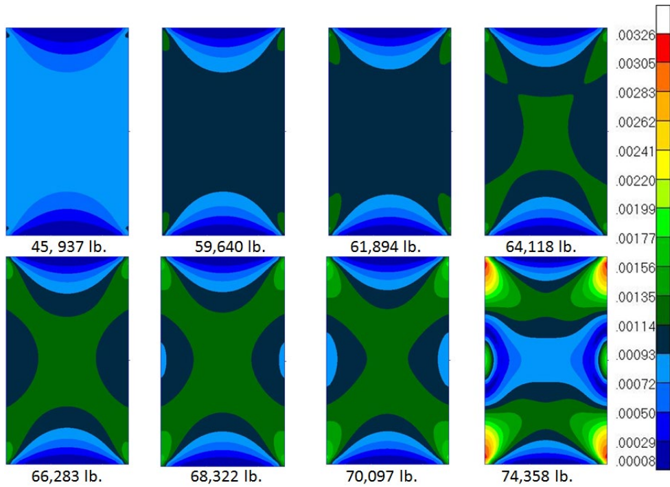
Figure 40.—Analytical maximum principal strain (Z) strain I.D.
