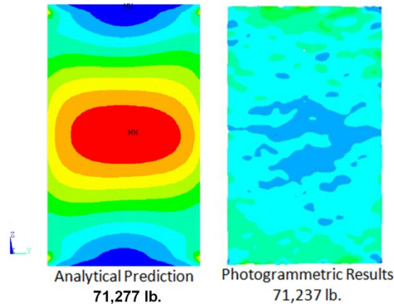
Figure 78.—Post-buckling O.D. minimum principal (Z-axis or longitudinal) strain comparison for Panel B-1.
