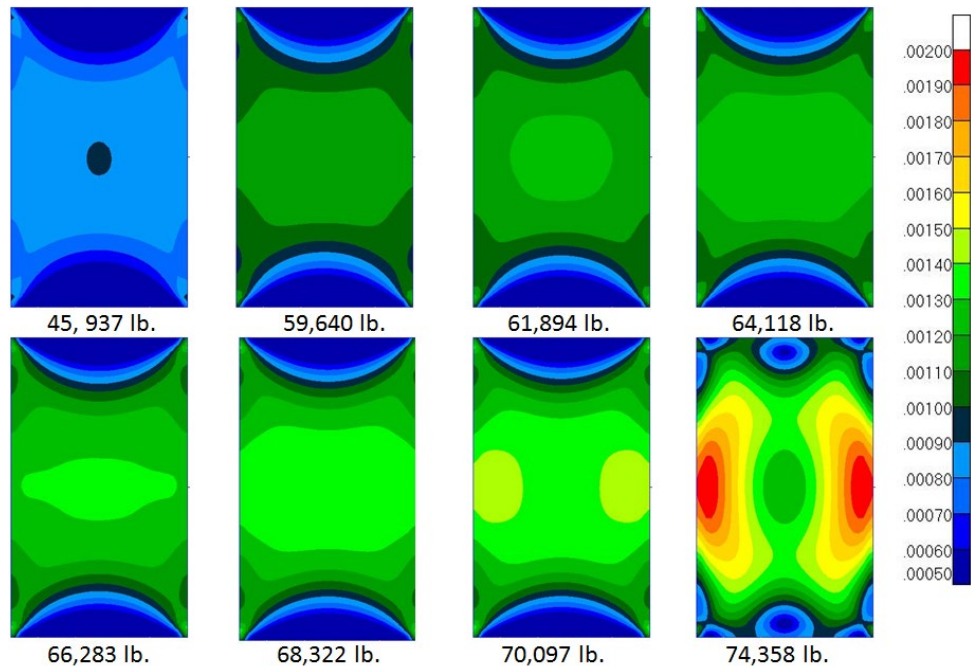
Figure 38.—Analytical maximum principal strain (Z) strain O.D.
