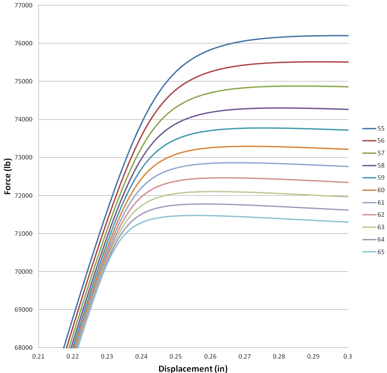
Figure 47.—Nonlinear static analysis results for altered 60° ply angle (magnified view).
