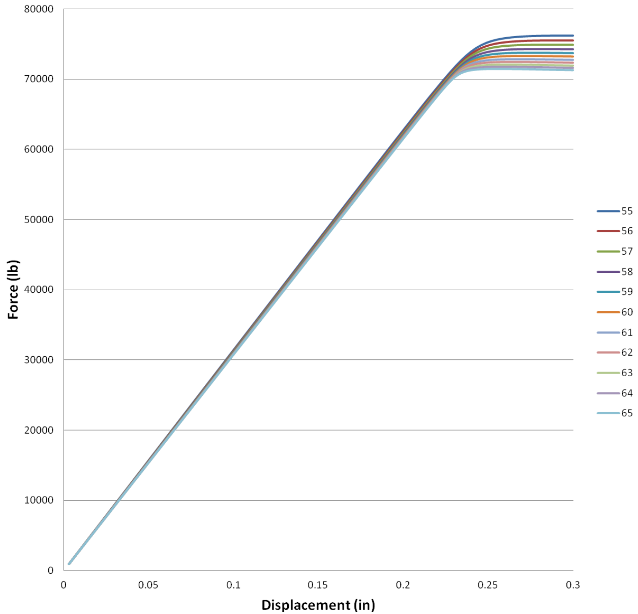
Figure 46.—Nonlinear static analysis results for altered 60° ply angle.
