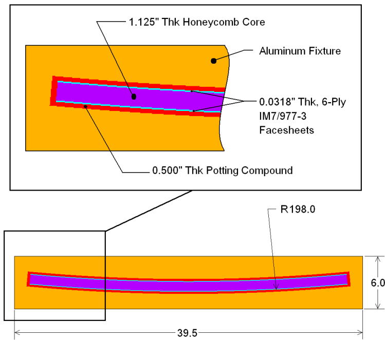
Figure 2.—The 3- by 5-ft arc segment test panel and test fixture end view.
