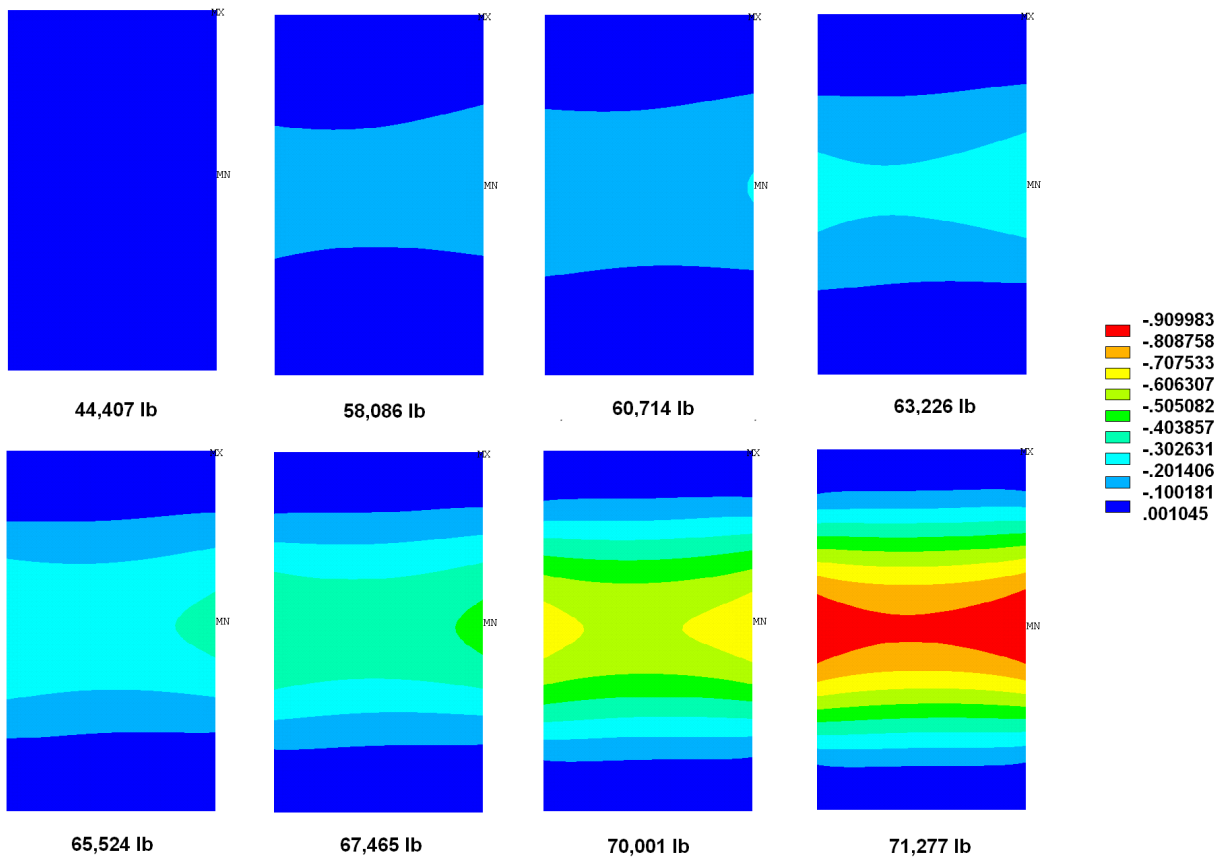
Figure 77.—ANSYS solid FEM out-of-plane (X-axis or radial) displacement contour plots versus load for Panel B-1.
