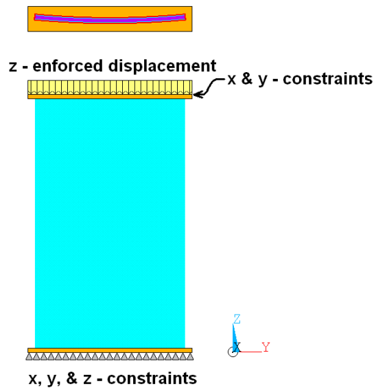
Figure 55.—ANSYS solid model boundary conditions.
