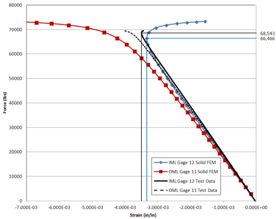
Figure 69.—Load versus minimum principal strain plot for gages 11 and 12, Panels B-1 and B-2.
