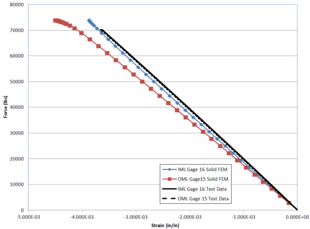
Figure 71.—Load versus minimum principal strain plot for gages 15 and 16, Panels B-1 and B-2.
