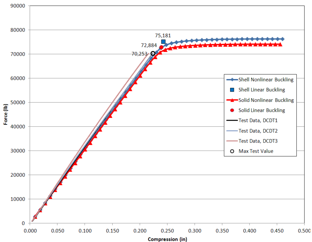
Figure 61.—Total reaction load versus end shortening for ANSYS solid and shell FEM's of Panel B-2.
