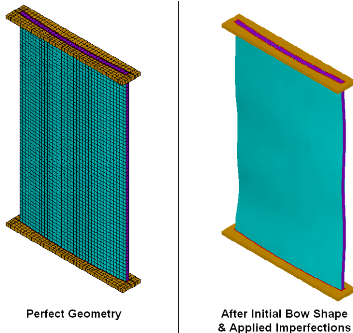
Figure 57.—Panel B-1 model with the applied initial bowed shape and geometric imperfections (exaggerated).
