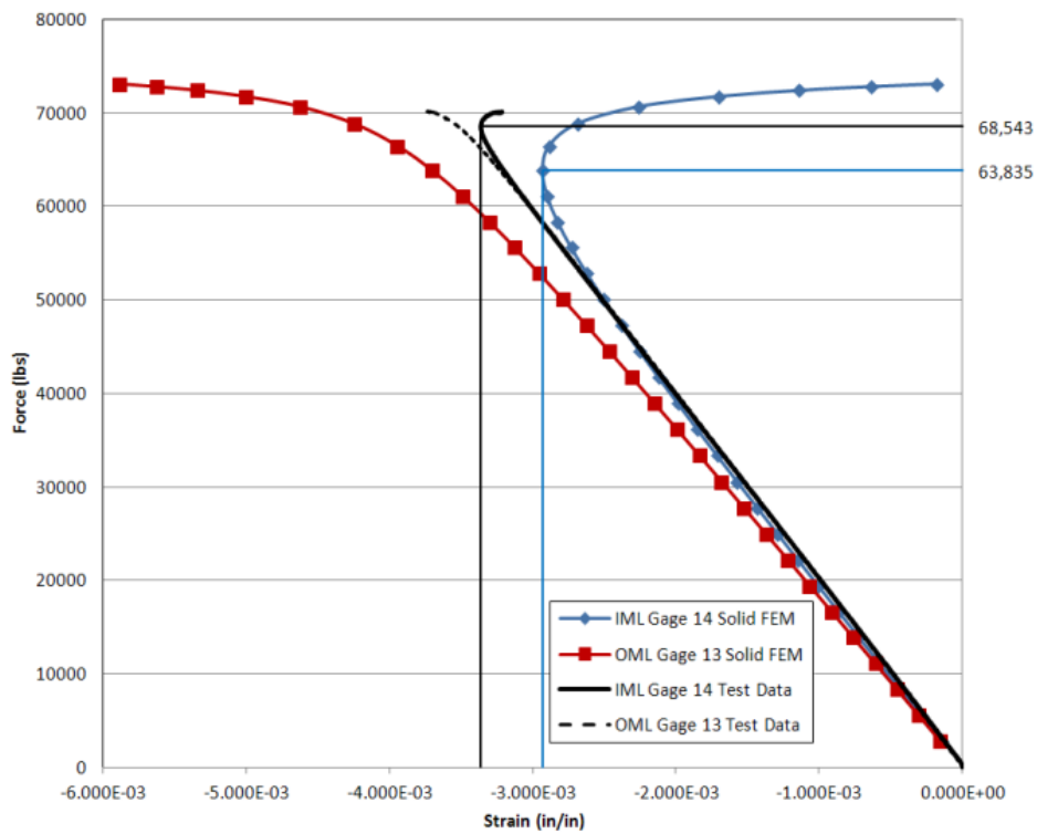
Figure 70.—Load versus minimum principal strain plot for gages 13 and 14, Panels B-1 and B-2.
