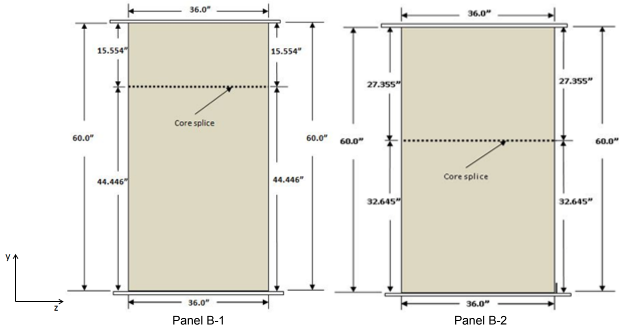
Figure 4.—Potted specimen dimensions for Panels B-1 and B-2. Note that the outside surfaces of the aluminum end plates were machined flat and parallel. The position of the core splices are also shown relative to the inside surface of the aluminum end plates.
