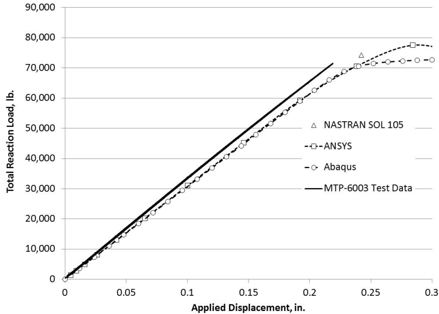
Figure 14.—Total Panel B-1 reaction load versus end shortening for Sols 105, ANSYS, Abaqus, and test.
