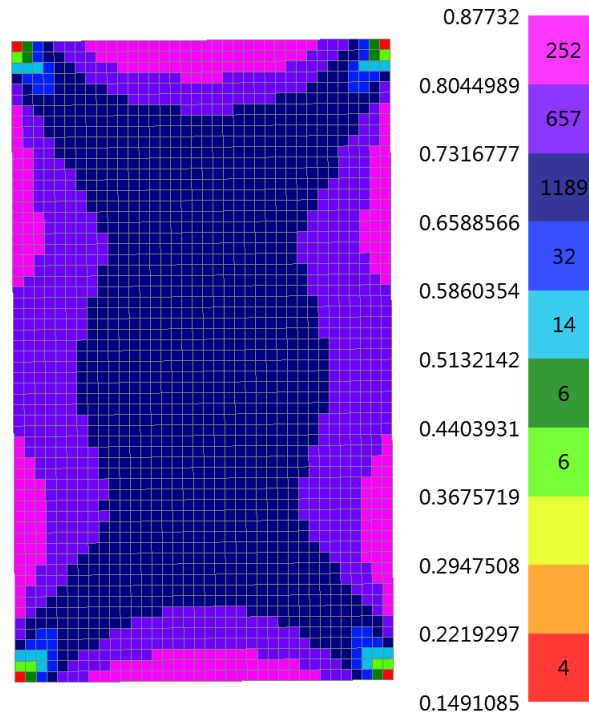
Figure 44.—HyperSizer margin of safety plot for core crimping, core crushing, facesheet wrinkling, and facesheet dimpling.
