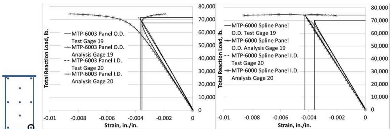
Figure 28.—Load/strain plot for MTP-6003 and MTP-6000 Approximated Spline Gages 19 and 20 lower, right side, even numbers on I.D. Analysis obtained from MSC/NASTRAN, Sol 106.
