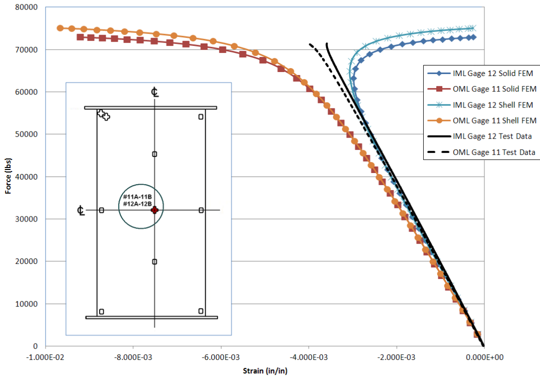
Figure 60.—Load versus minimum principal strain plots for Panel B-1 at gages 11 and 12.
