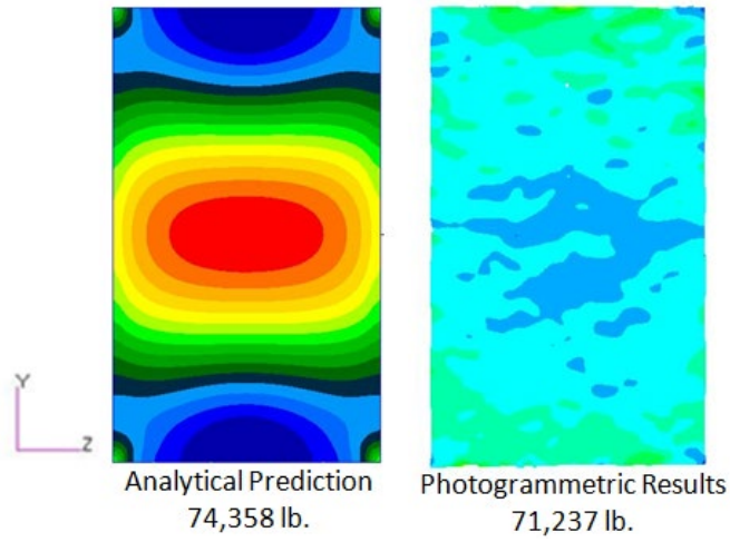
Figure 33.—Post-buckling O.D. minimum principal (Y) strain comparison.
