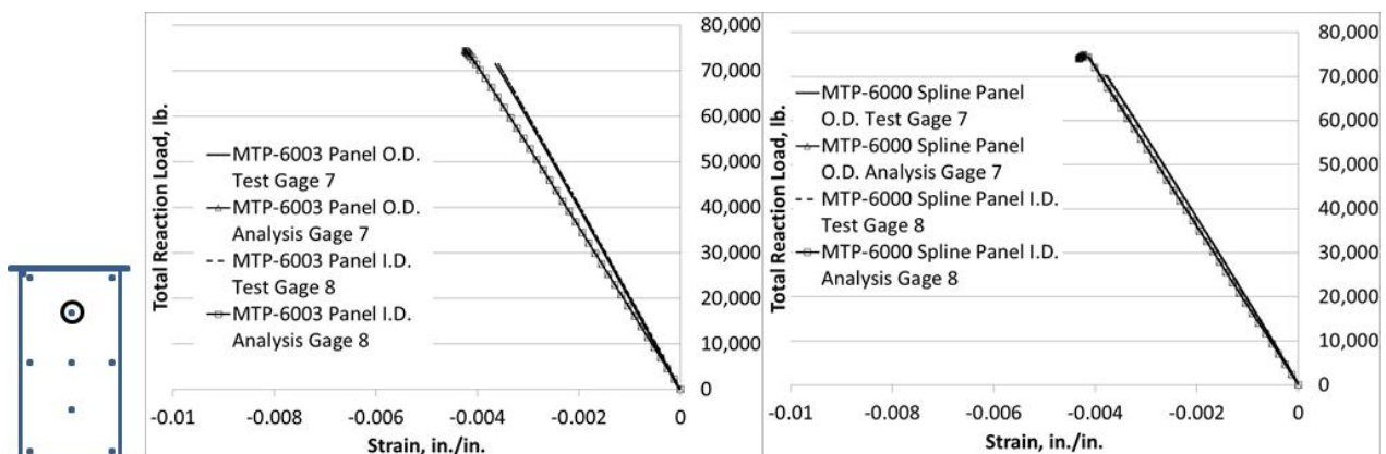
Figure 22.—Load/strain plot for MTP-6003 and MTP-6000 Approximated Spline Gages 7 and 8, upper ¼ length, center, even numbers on I.D. Analysis obtained from MSC/NASTRAN, Sol 106.
