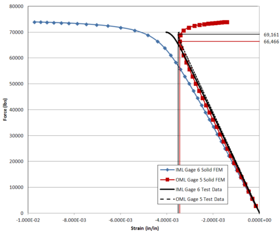
Figure 66.—Load versus minimum principal strain plot for gages 5 and 6, Panels B-1 and B-2.
