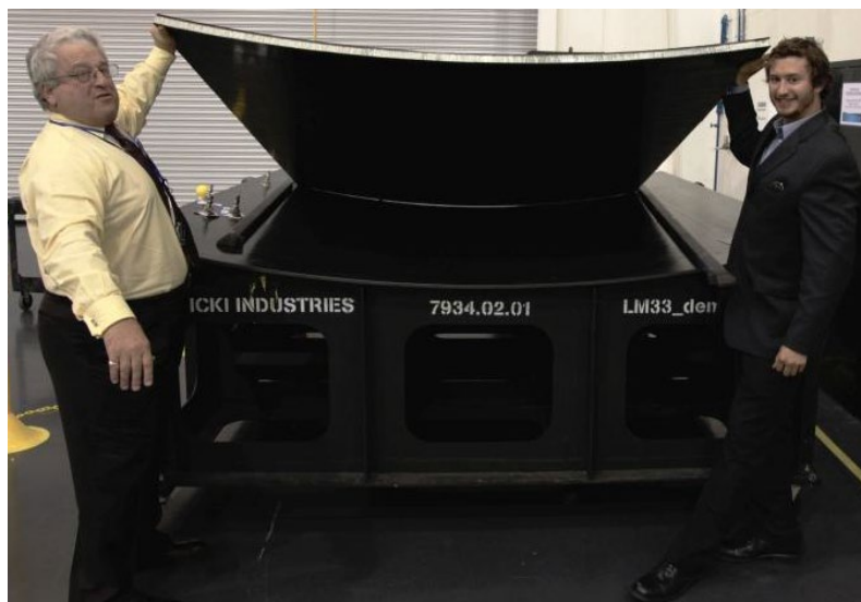
Figure 1.—Cured 1/16 th arc segment panel and the tool it was molded on.
