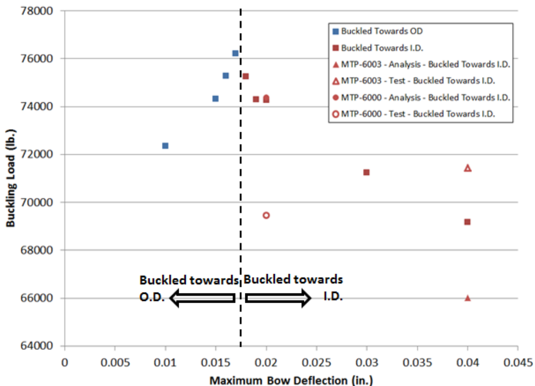
Figure 45.—Impact of initial panel bow geometry on panel buckling loads.
