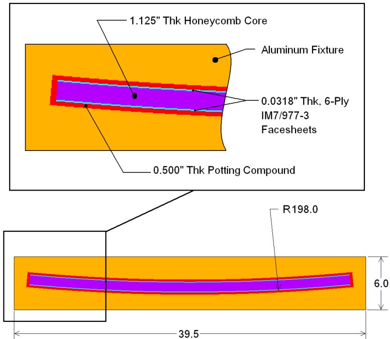
Figure 53.—The 3- by 5-ft arc segment test panel and test fixture end view.
