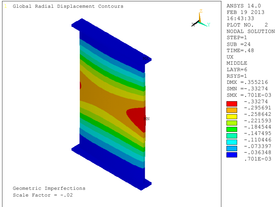
Figure 59.—ANSYS solid FEM, radial displacement contour plot for Panel B-1 at 0.219-in. end shortening.
