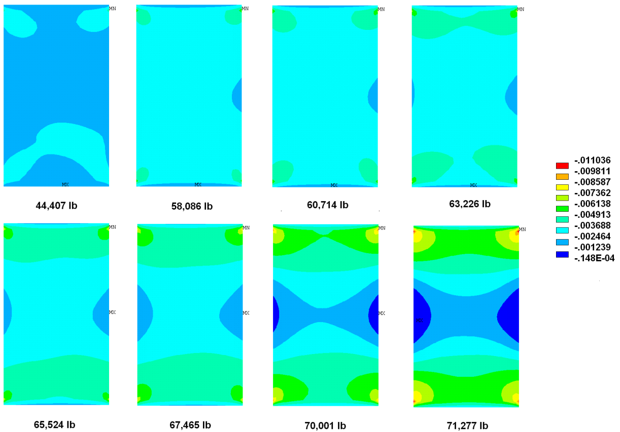
Figure 81.—ANSYS solid FEM, I.D. minimum principal strain (z-axis or longitudinal) for Panel B-1.
