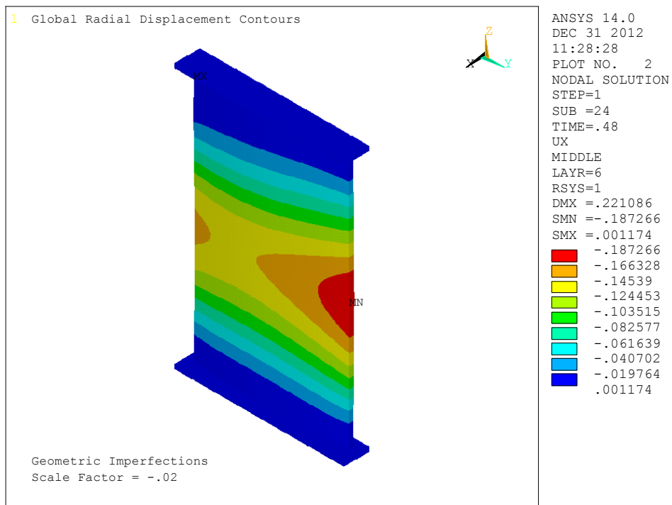
Figure 62.—ANSYS solid FEM, radial displacement contour plot for Panel B-2 at 0.219-in. end shortening.
