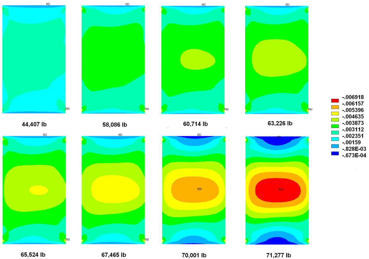
Figure 79.—ANSYS solid FEM, O.D. minimum principal strain (z-axis or longitudinal) for Panel B-1.
