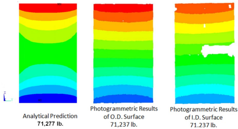
Figure 74.—Post-buckling Z (in-plane or longitudinal) displacement comparison for Panel B-1.
