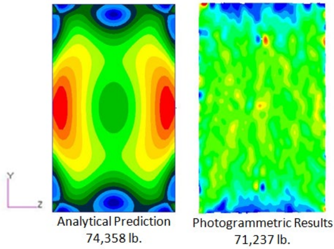
Figure 37.—Post-buckling O.D. maximum principal (Z) strain comparison.
