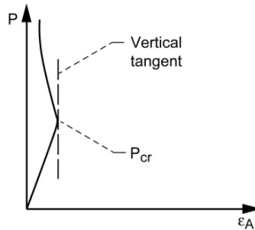
Figure 10.—Method for determining buckling load (Singer et al.,1998).
