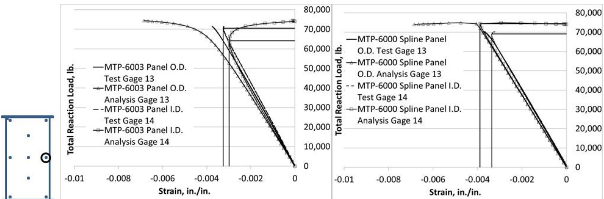
Figure 25.—Load/strain plot for MTP-6003 and MTP-6000 Approximated Spline Gages 13 and 14 center, left side, even numbers on I.D. Analysis obtained from MSC/NASTRAN, Sol 106.
