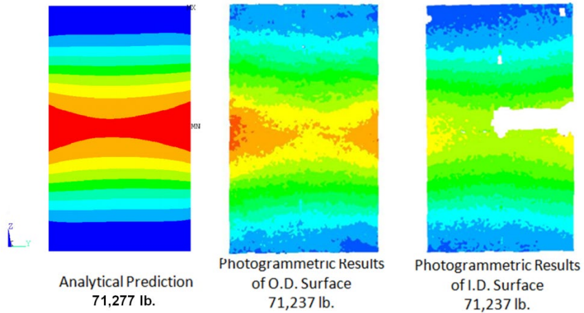
Figure 76.—Post-buckling X (out-of-plane or radial) displacement comparison for Panel B-1.
