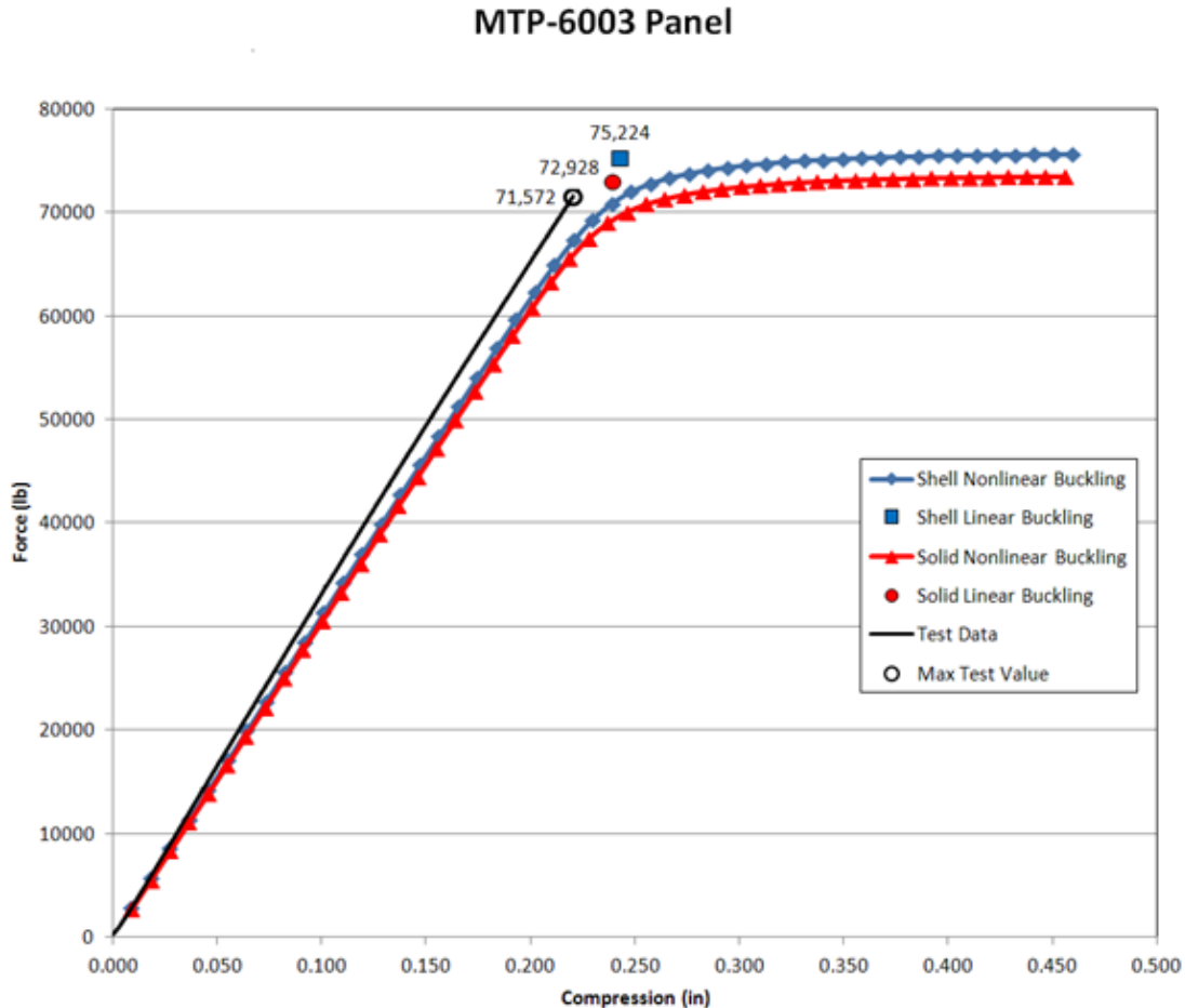
Figure 58.—Total reaction load versus end shortening for ANSYS solid and shell FEMs of panel B-1.
