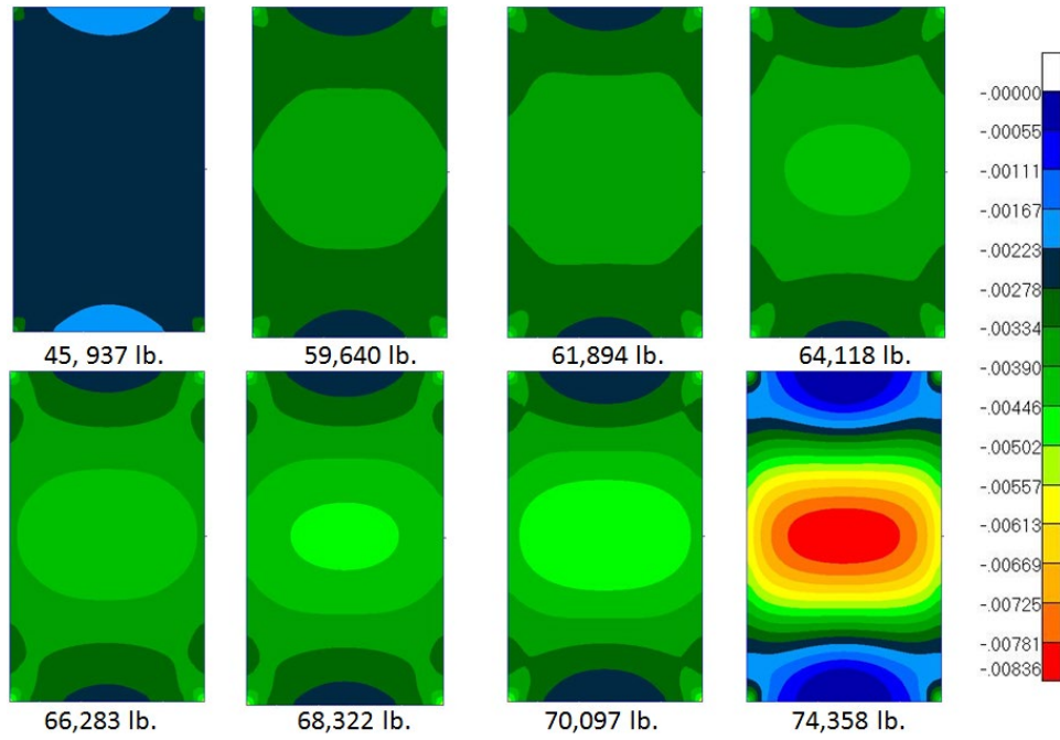
Figure 34.—Analytical minimum principal strain (Y) strain O.D.
