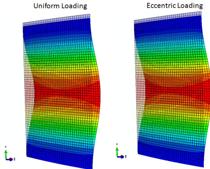
Figure 49.—Post-buckled shape with uniform applied displacement and simulated eccentric applied displacement.
