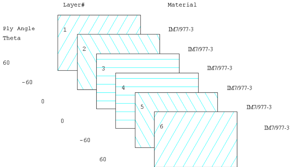
Figure 54.—Facesheet 6-Ply stacking sequence.
