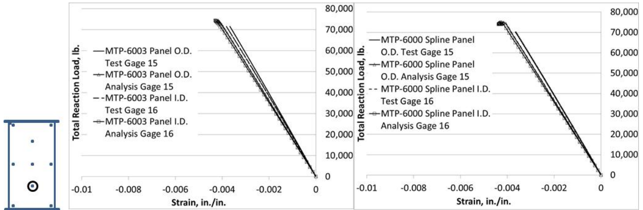
Figure 26.—Load/strain plot for MTP-6003 and MTP-6000 Approximated Spline Gages 15 and 16, lower ¼ length, center, even numbers on I.D. Analysis obtained from MSC/NASTRAN, Sol 106.
