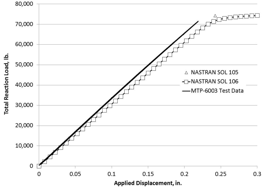
Figure 13.—Total Panel B-1 reaction load versus end shortening for Sols 105, 106 and test.
