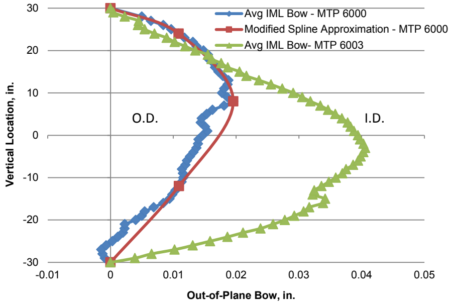
Figure 9.—Imperfection, or bow, data from the bag side (I.D.) of the panel. Data were taken vertically along the height of the panel, in the horizontal center of the panel.
