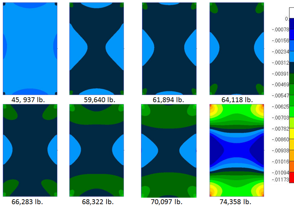
Figure 36.—Analytical minimum principal strain (Y) strain I.D.
