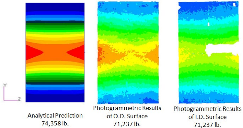
Figure 31. Post-buckling X (out-of-plane) displacement comparison.
