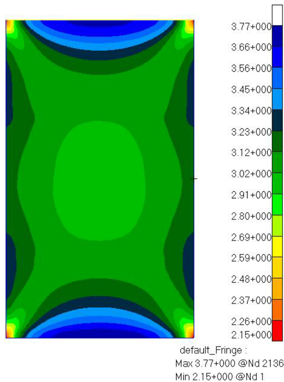
Figure 41.—Strength ratio plot at buckling load.
