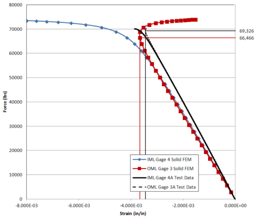
Figure 65.—Load versus minimum principal strain plot for gages 3 and 4, Panels B-1 and B-2.
