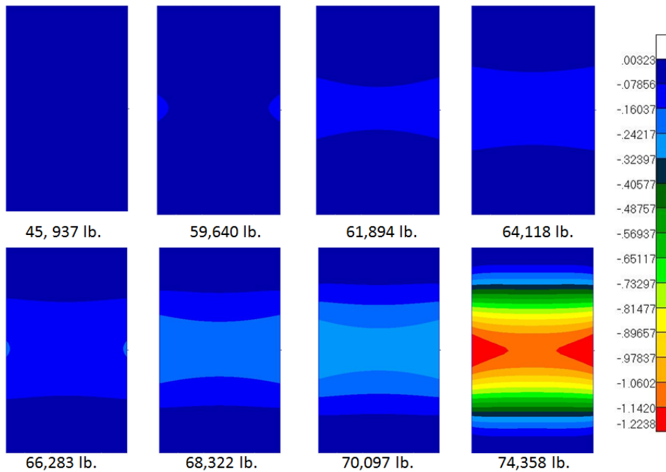
Figure 32.—Analytical X (out-of-plane) displacement.
