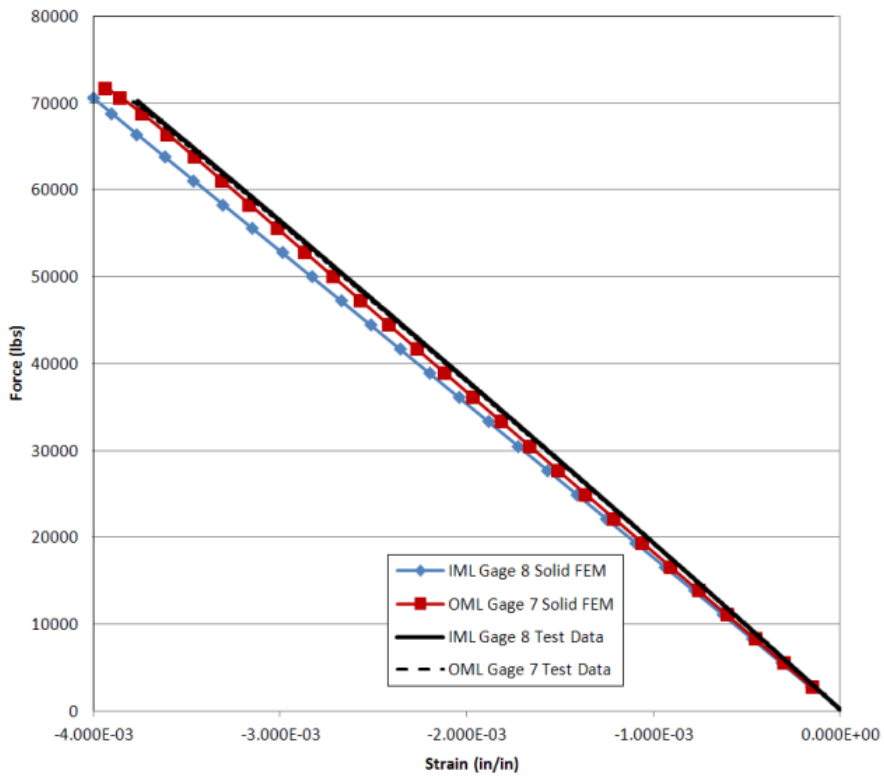
Figure 67.—Load versus minimum principal strain plot for gages 7 and 8, Panels B-1 and B-2.
