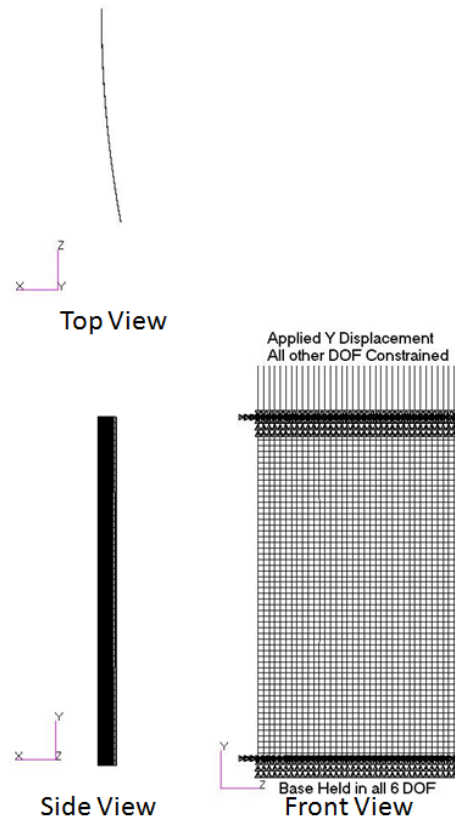
Figure 8.—Panel geometry with boundary conditions.
