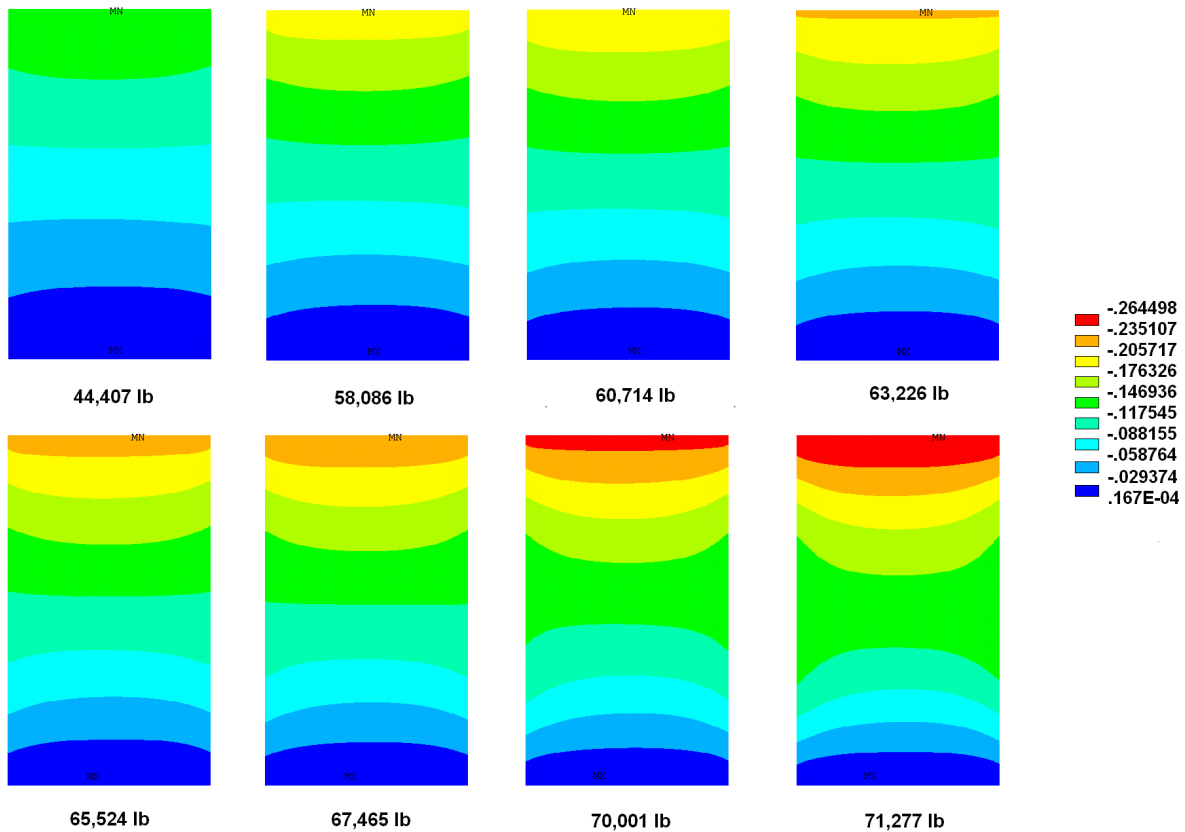
Figure 75.—ANSYS solid FEM axial (Z-axis or longitudinal) displacement contour plots versus load for Panel B-1.
