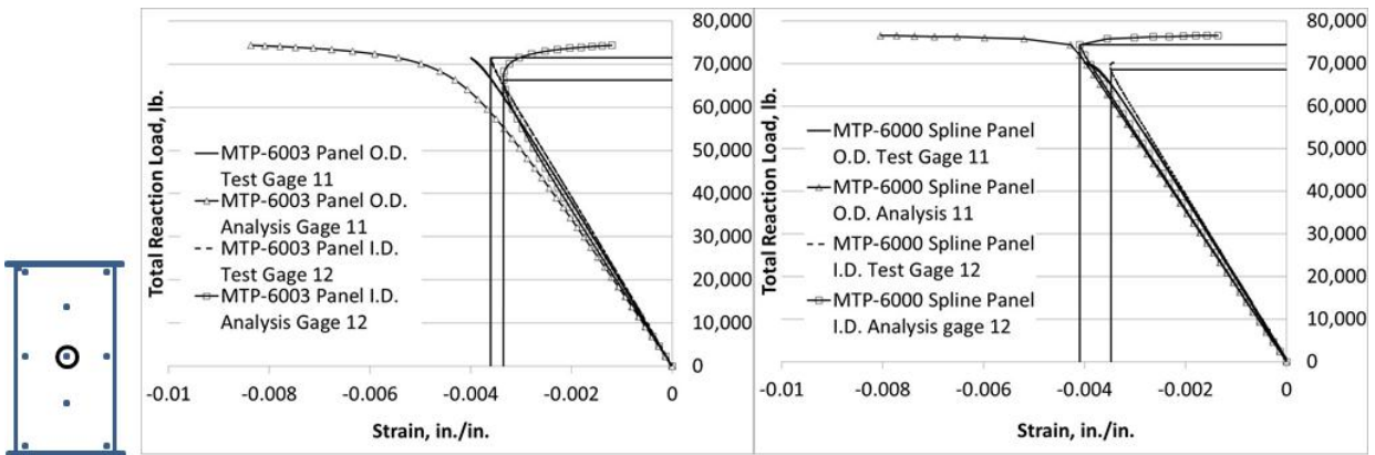
Figure 24.—Load/strain plot for MTP-6003 and MTP-6000 Approximated Spline Gages 11 and 12,center of panel, even numbers on I.D. Analysis obtained from MSC/NASTRAN, Sol 106.
