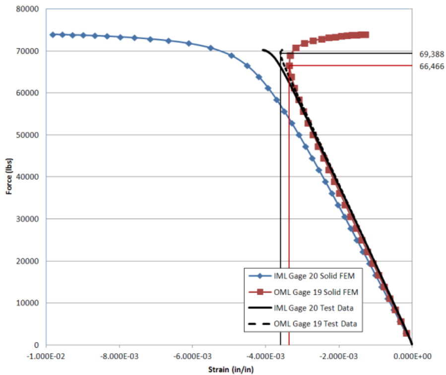
Figure 73.—Load versus minimum principal strain plot for gages 19 and 20, Panels B-1 and B-2.
