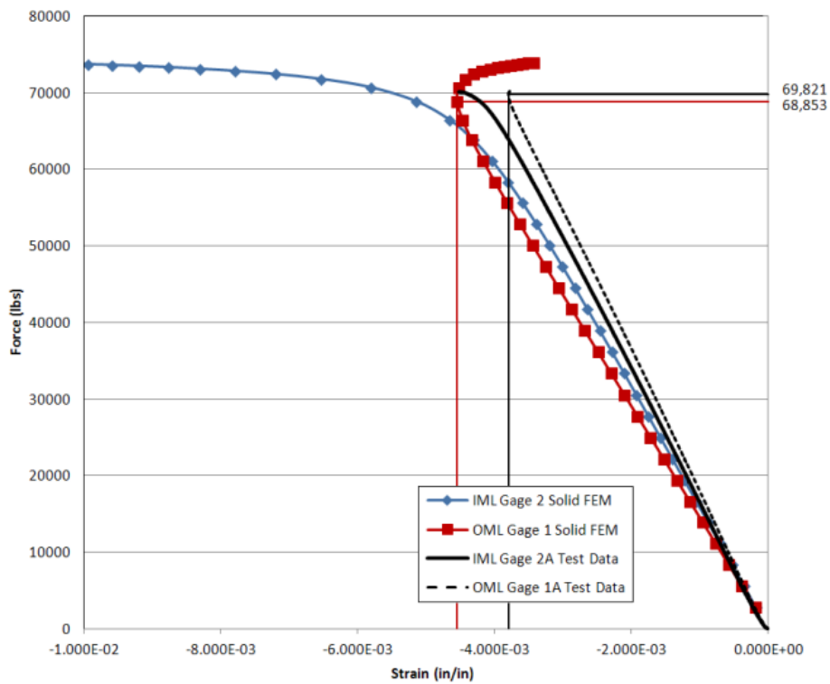
Figure 64.—Load versus minimum principal strain plot for gages 1 and 2, Panels B-1 and B-2.
