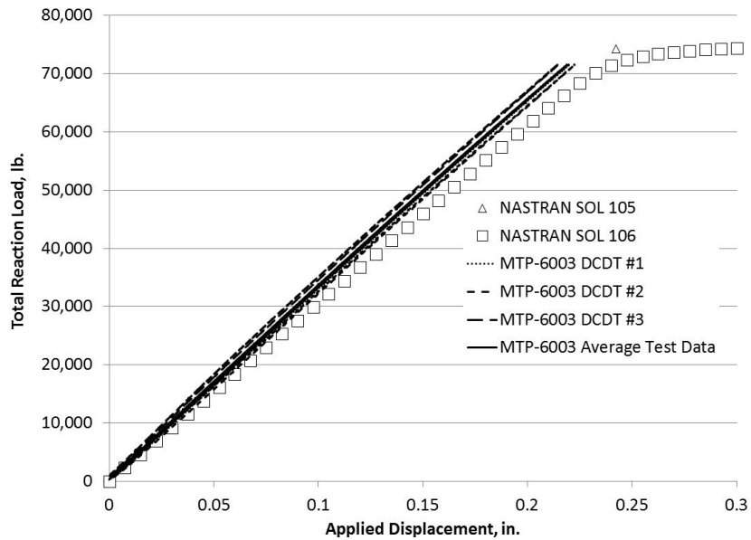
Figure 15.—DCDT end shortening versus total reaction load (Panel B-1).
