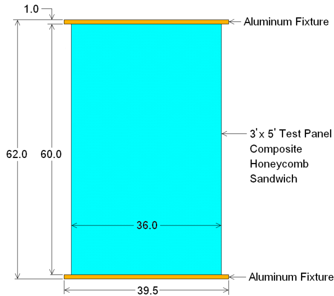
Figure 52.—The 3- by 5-ft arc segment test panel configuration.
