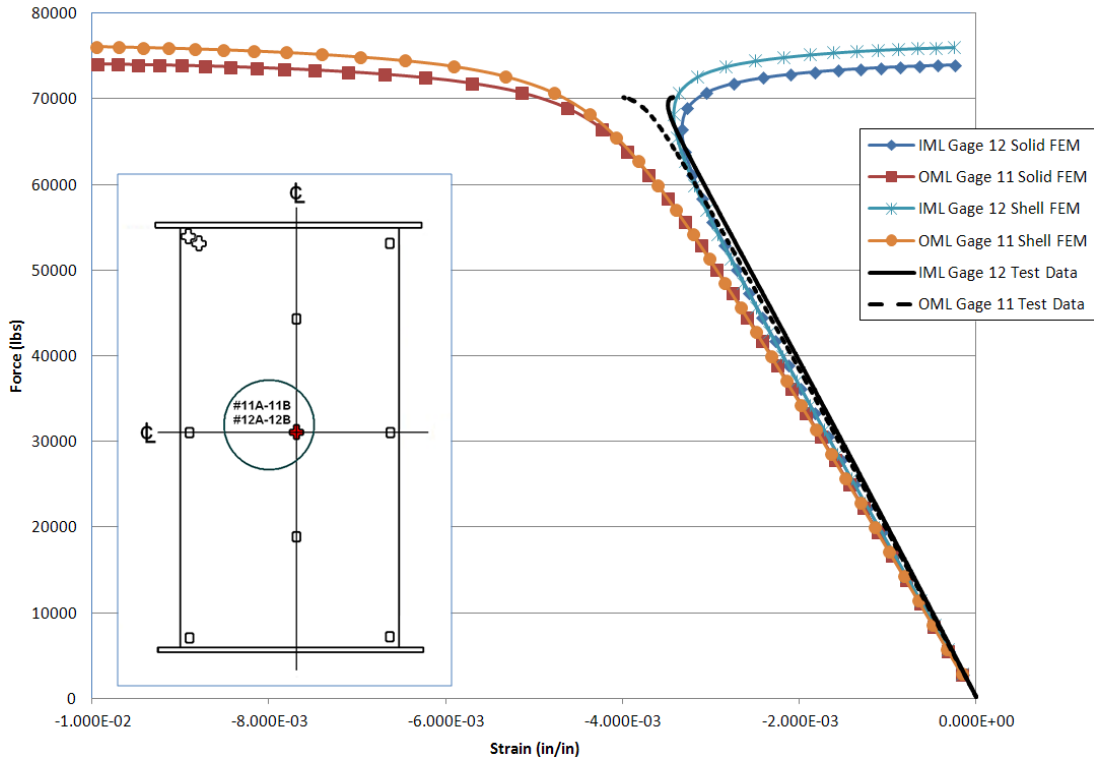
Figure 63.—Load versus minimum principal strain plot for Panel B-2 at gages 11 and 12.
