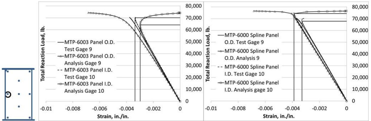
Figure 23.—Load/strain plot for MTP-6003 and MTP-6000 Approximated Spline Gages 9 and 10,center, left side, even numbers on I.D.. Analysis obtained from MSC/NASTRAN, Sol 106.
