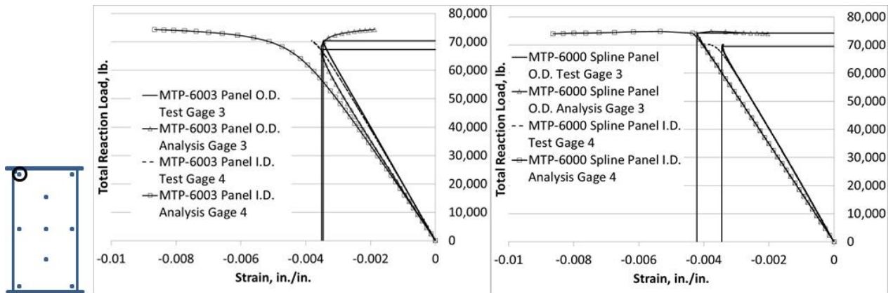
Figure 20.—Load/strain plot for MTP-6003 and MTP-6000 Approximated Spline Gages 3 and 4, upper, left side, even numbers on I.D. Analysis obtained from MSC/NASTRAN, Sol 106.
