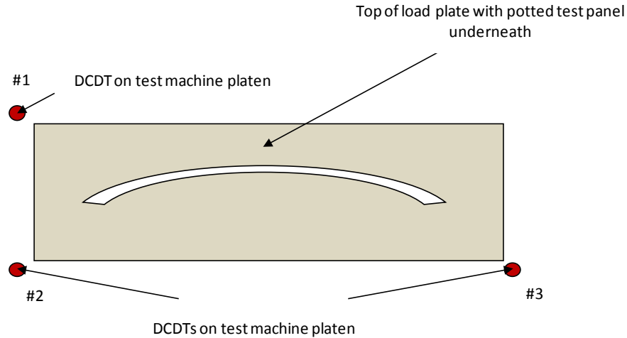
Figure 6.—Location of DCDT's on test machine platen.
