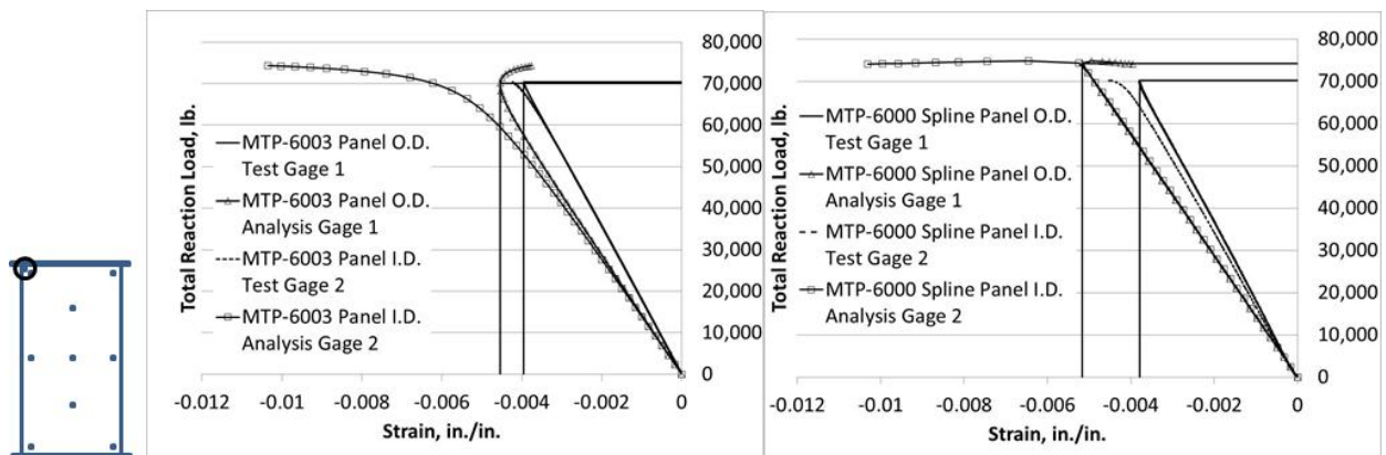
Figure 19.—Load/strain plot for MTP-6003 and MTP-6000 Approximated Spline Gages 1 and 2 upper, left side, even numbers on I.D. Analysis obtained from MSC/NASTRAN, Sol 106.
