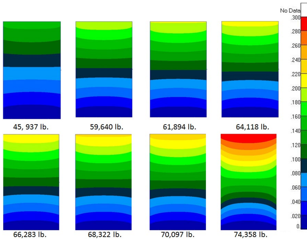
Figure 30.—Analytical Y (in-plane) displacement.
