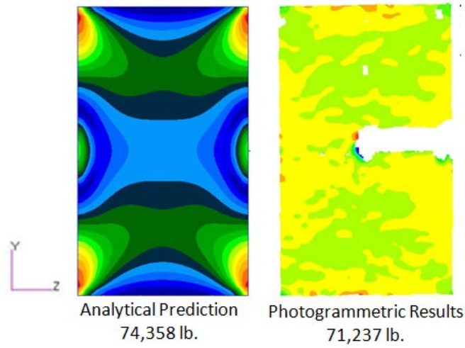
Figure 39.—Post-buckling I.D. maximum principal (Z) strain comparison.
