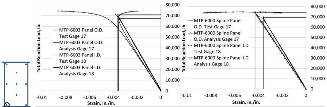
Figure 27.—Load/strain plot for MTP-6003 and MTP-6000 Approximated Spline Gages 17 and 18 lower, left side, even numbers on I.D. Analysis obtained from MSC/NASTRAN, Sol 106.
