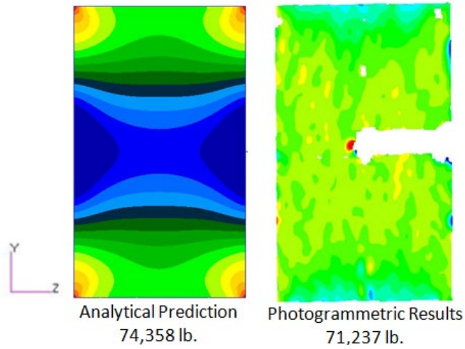
Figure 35.—Post-buckling I.D. minimum principal (Y) strain comparison
