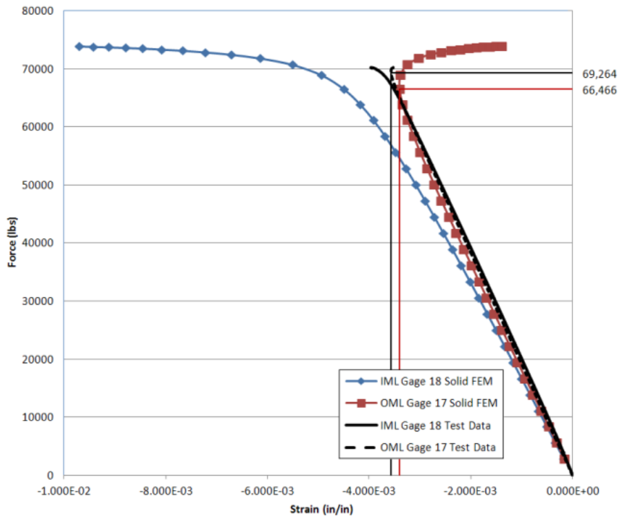
Figure 72.—Load versus minimum principal strain plot for gages 17 and 18, Panels B-1 and B-2.
