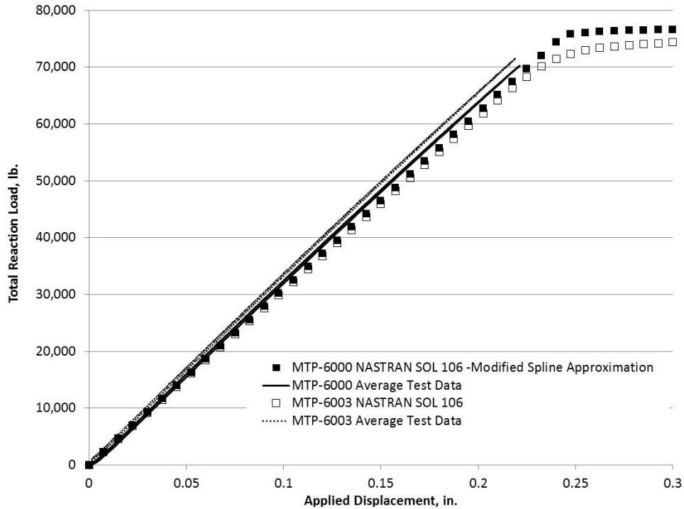
Figure 17.—DCDT end shortening versus total reaction load comparison of Panel B-1 with Panel B-2.
