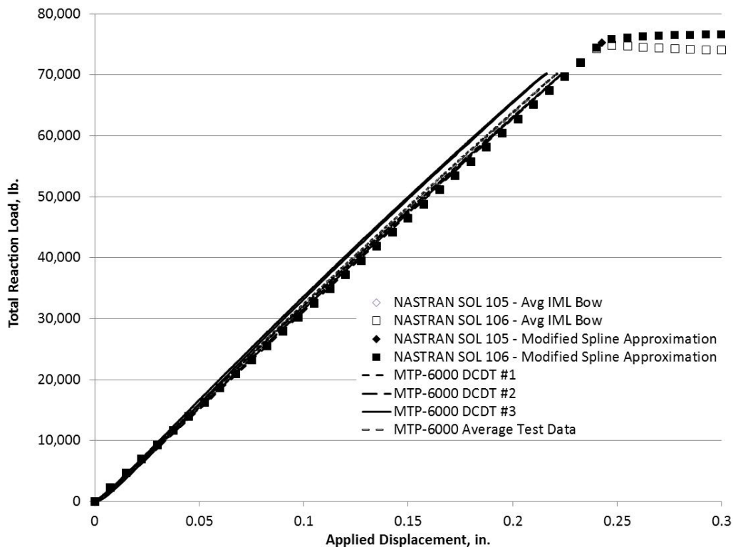
Figure 16.—DCDT end shortening versus total reaction load (Panel B-2).
