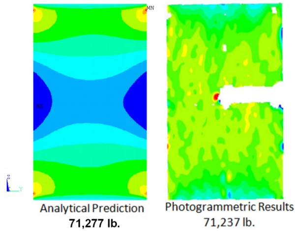
Figure 80.—Post-buckling I.D. minimum principal (Z-axis or longitudinal) strain comparison for Panel B-1.
