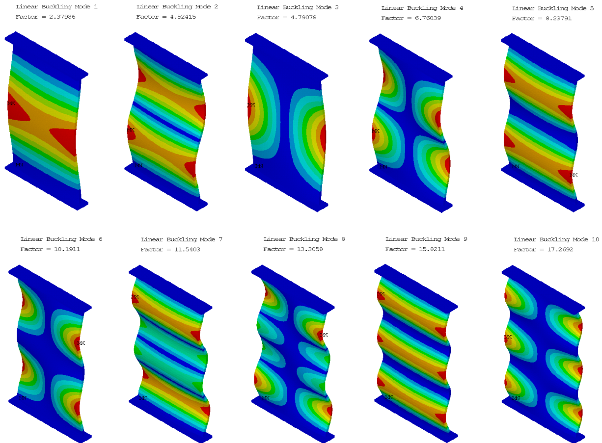
Figure 56.—The first 10 linear buckling mode shapes for the 3 by 5 panel with 6-ply facesheets.
