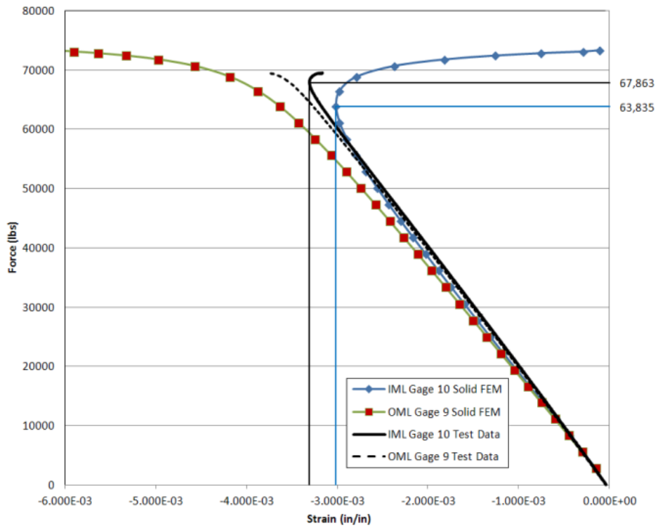
Figure 68.—Load versus minimum principal strain plot for gages 9 and 10, Panels B-1and B-2.
