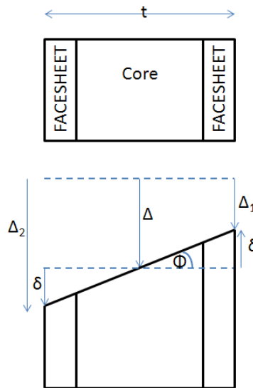
Figure 48.—Diagram showing eccentric loading applied through the thickness of the panel leading to rotation of the panel edge.
