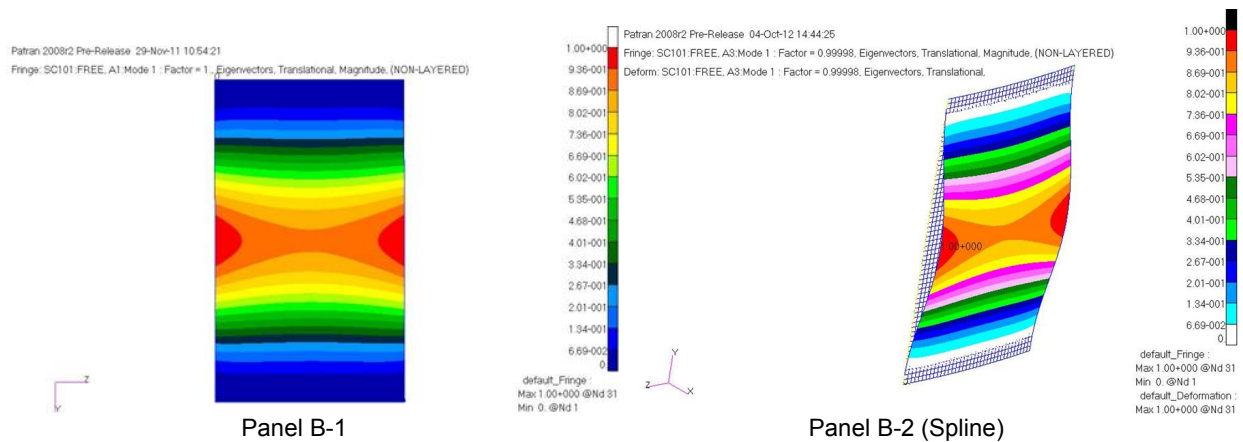
Figure 11.—Euler eigenvector buckling plot obtained from MSC/NASTRAN.
