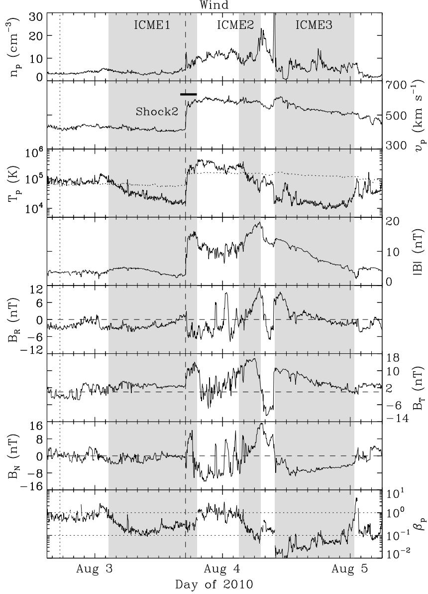
Fig. 4.— Solar wind plasma and magnetic field parameters observed at Wind. From top to bottom, the panels show the proton density, bulk speed, proton temperature, magnetic field strength and components, and proton \beta , respectively. The dotted curve in the third panel denotes the expected proton temperature from the observed speed. The shaded regions show the ICME intervals, and the vertical dashed line indicates the associated shock. The horizontal line in the second panel marks the predicted arrival time (with uncertainties) and speed of the merged front of CME2 and CME3 at the spacecraft. The predicted arrival time of CME1 is indicated by the vertical dotted line.
