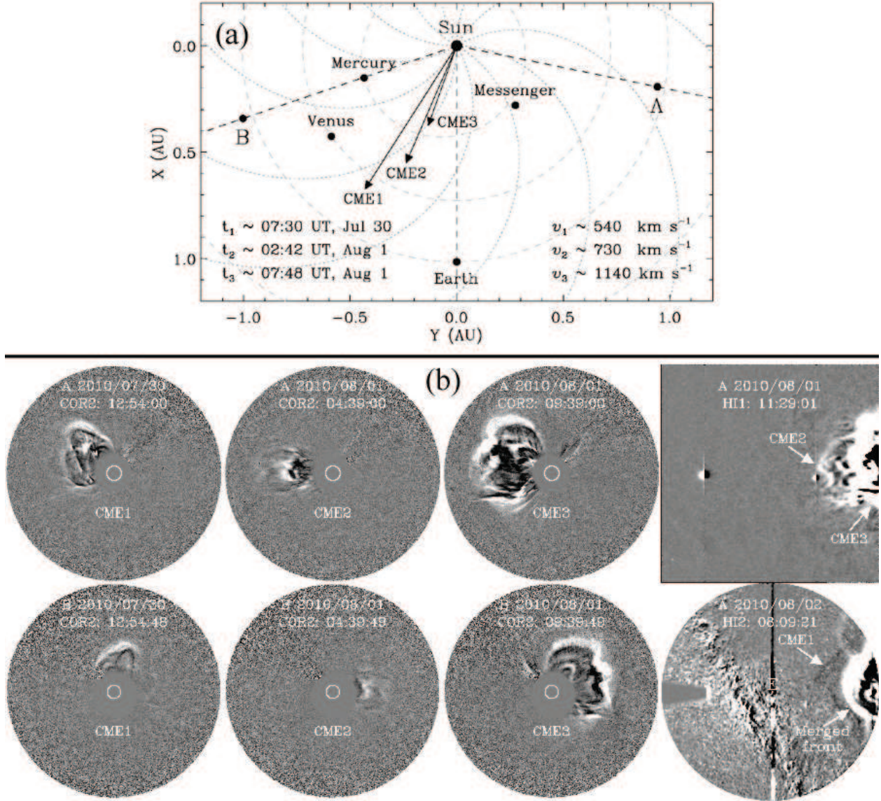
Fig. 1.— (a) Positions of the spacecraft and planets in the ecliptic plane on 2010 August 1. The gray dashed curves indicate the planetary orbits, and the dotted lines show Parker spiral magnetic fields. The arrows mark the propagation directions of the CMEs of interest obtained from a triangulation technique. The estimated CME speeds and launch times on the Sun are also given. (b) CME evolution observed by STEREO. The left three columns display COR2 images of the three CMEs viewed from STEREO A (upper) and B (lower) near simultaneously. The right column shows images from HI1 and HI2 of STEREO A, which indicate the scenario of CME-CME interactions. The position of the Earth is labeled as E. (Animations of this figure are available in the online journal.)
