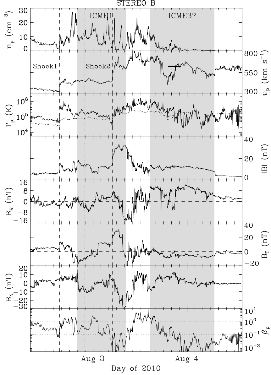
Fig. 5.— Similar format to Figure 4, but for the measurements at STEREO B. ICME1 has a forward shock at STEREO B, while only a discontinuity is observed at Wind.
