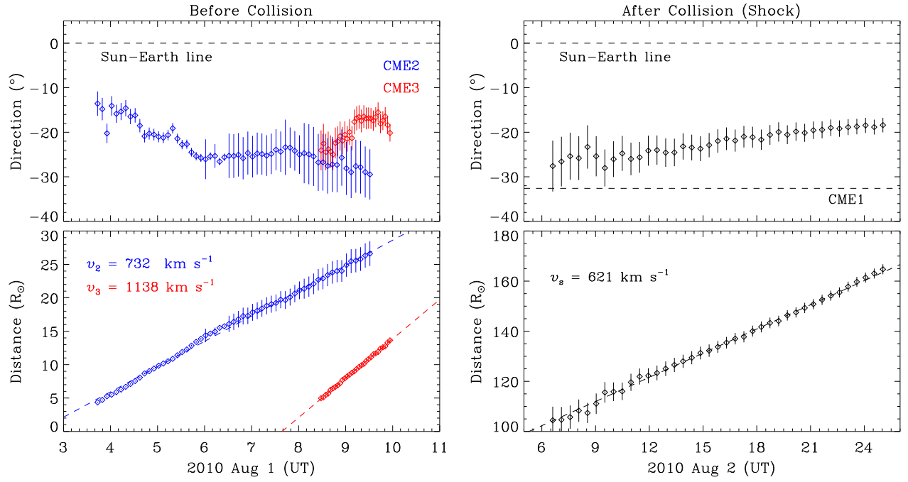
Fig. 3.— Propagation direction and radial distance derived from geometric triangulation before (left) and after (right) collision between CME2 and CME3. The lower dashed line in the top right panel indicates the propagation angle of CME1. Also shown are linear fits to the distances, together with the speeds obtained from the fits.
