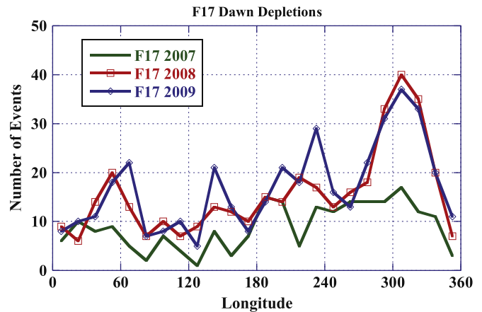
Fig. 8. Occurrences of dawn depletions from the DMSP F17 satellite are shown for three years, 2007 (green), 2008 (red) and 2009 (blue) (adapted from Gentile et al., 2011). (For interpretation of the references to color in this figure legend, the reader is referred to the web version of this article.)
