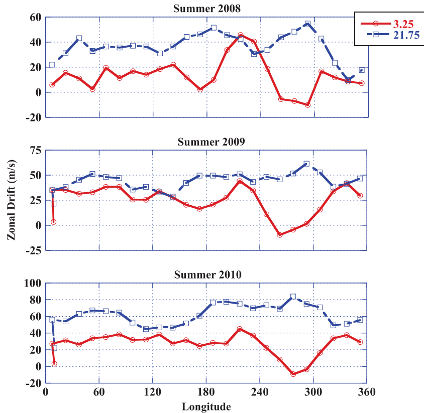
Fig. 5. VEFI zonal drifts for two local times on the nightside are shown for the same three summer solstice periods as in Fig. 4. The post-sunset LT (blue) and post-midnight LT (red) are plotted. (For interpretation of the references to color in this figure legend, the reader is referred to the web version of this article.)
