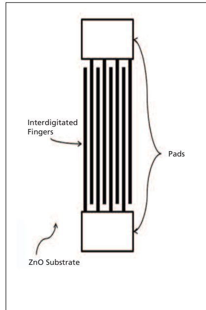
Schematic of the UV Photodetector.
