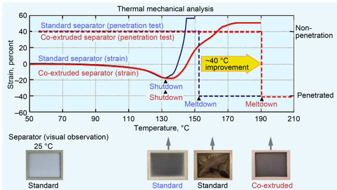
Figure 2.—Thermal mechanical properties of ExxonMobil/Tonen battery separator products (Ref. 10).
