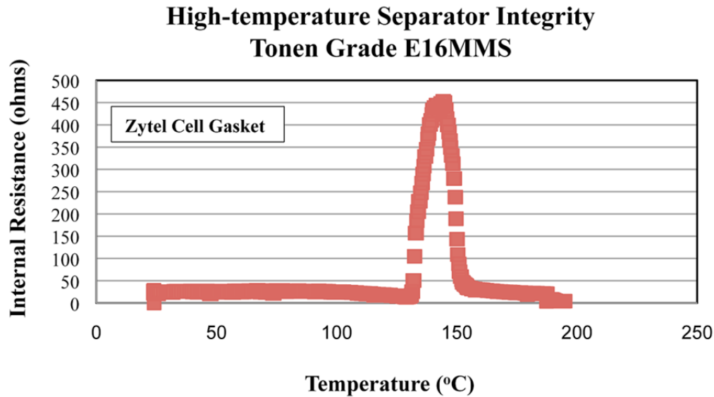
Figure 9.—Experimental high-temperature separator integrity data for Tonen E16MMS material with a Zytel cell gasket employed.
