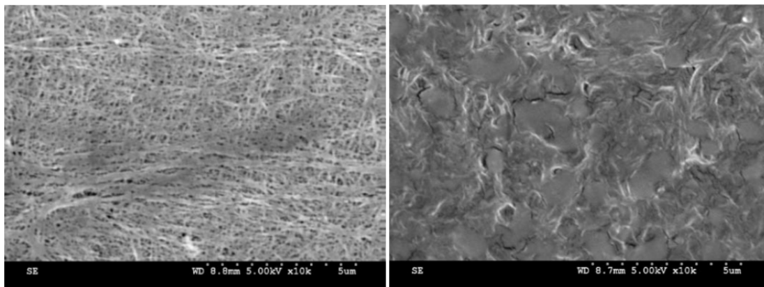
Figure 14.—SEM photos of Tonen E16MMS separator material before and after heating to >185^{\circ}\text{C} during the resistance measurement testing.
