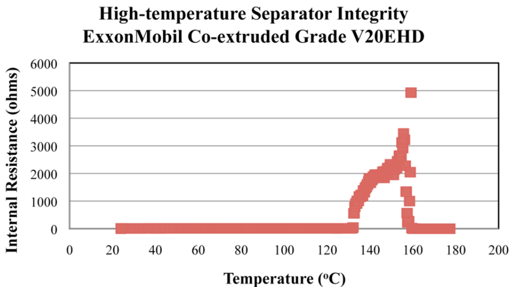
Figure 10.—Experimental high-temperature separator integrity data for ExxonMobil grade V20EHD material.
