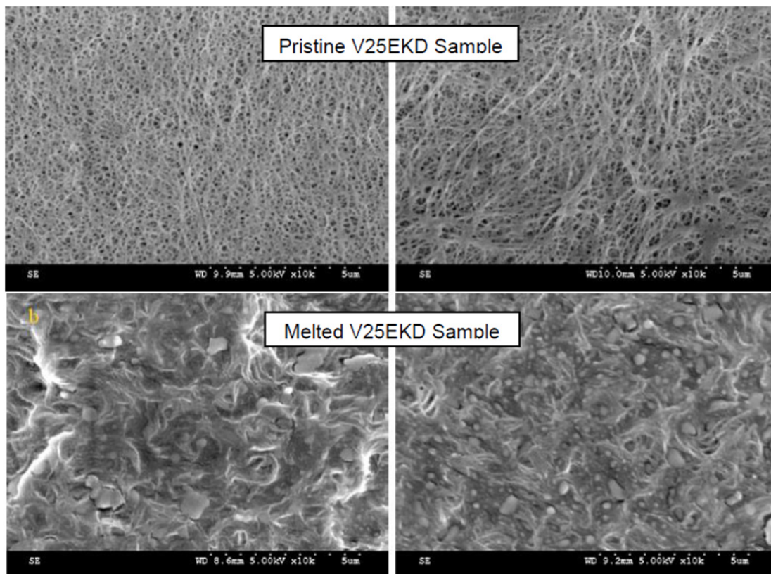
Figure 15.—SEM photos of ExxonMobil V25EKD separator material before and after heating to >185^{\circ}\text{C} during the resistance measurement testing.
