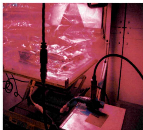
Figure 4: Pressure transducer test set up
