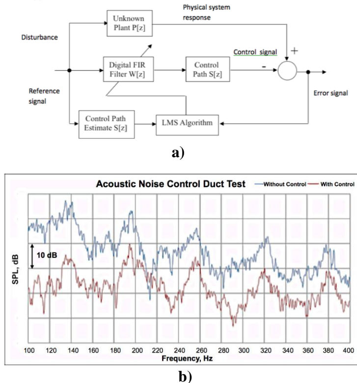
Figure 12. a) Block diagram of feedforward arrangement and b) example benchtop performance of active noise control system.
