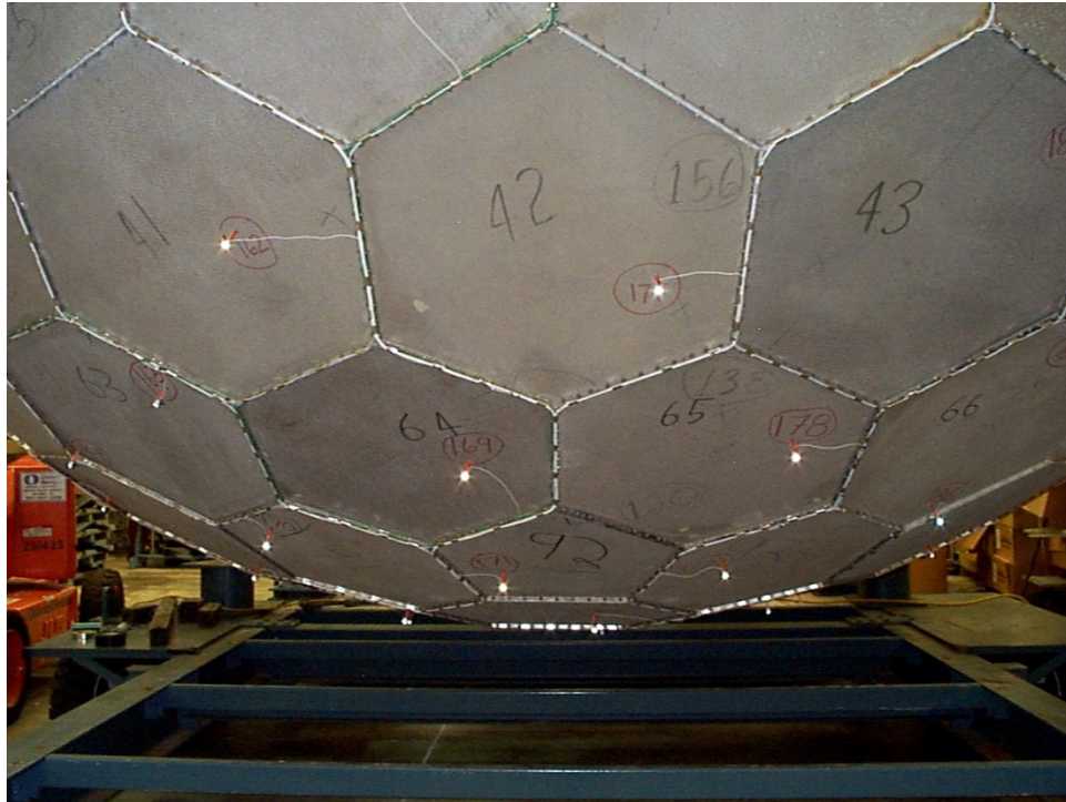
Figure 160.—Light from camera flash reflecting from photorefective targets.
