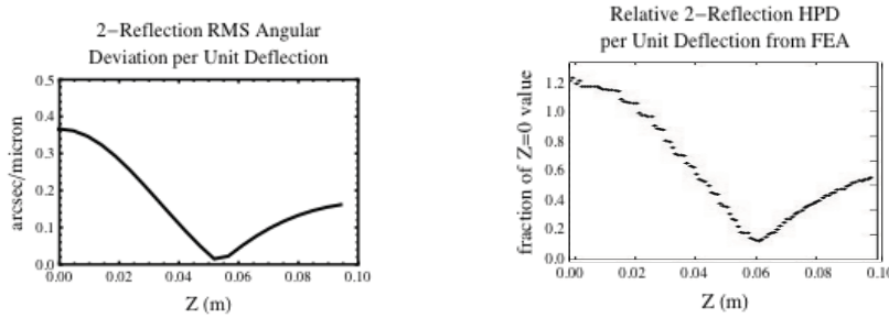
Figure 8: The analytical results are shown on the left; the FEA results on the right show the same trend.
