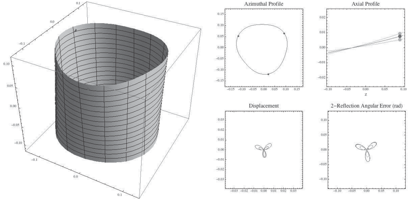
Figure 3: An example of using analytical modeling to gain insight through visualization. A deformed shell is shown on the left. The plots on the right show the azimuthal profile in the mounting plane (points are mounting locations), the axial profile of the mounting meridians, the mean displacement vs. azimuth, and the 2-reflection angular error vs. azimuth. The 2-reflection angular error is discussed in Section 3.3.
