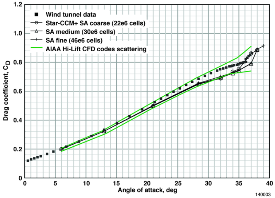
Figure 5. Star-CCM+ CFD code validation results for drag coefficient, Mach 0.2, Reynolds number based on mean aerodynamic chord of 4.3 million.
