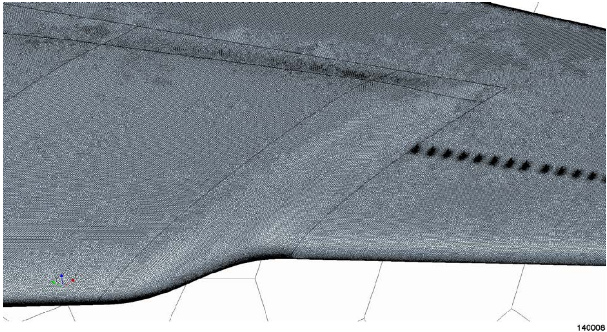
b) Gloved wing (4 vortex generators missing).
