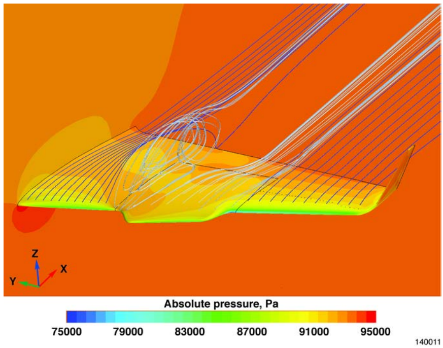
b) Stalled gloved wing.
