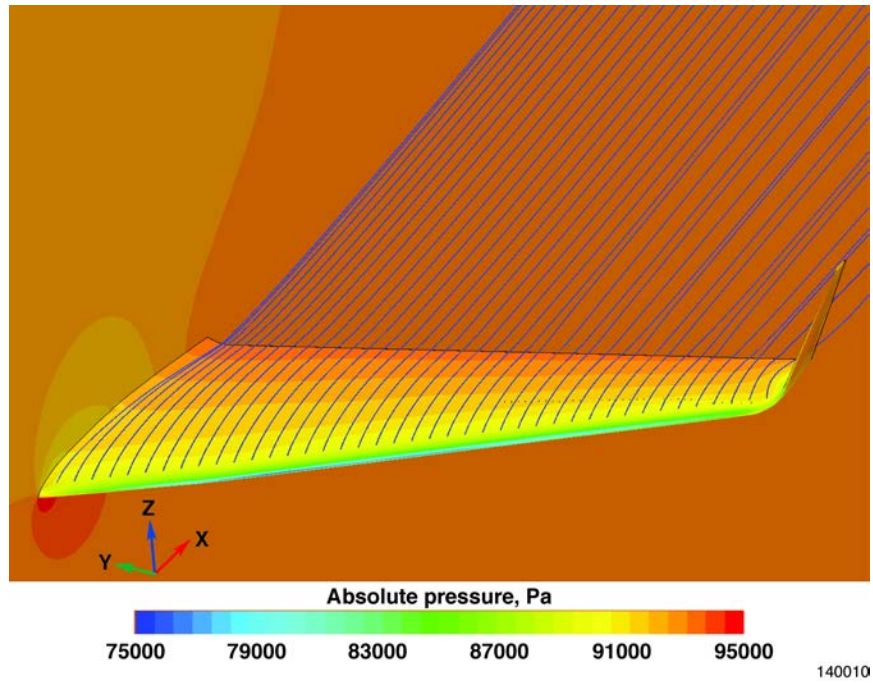
a) Unstalled clean wing.
