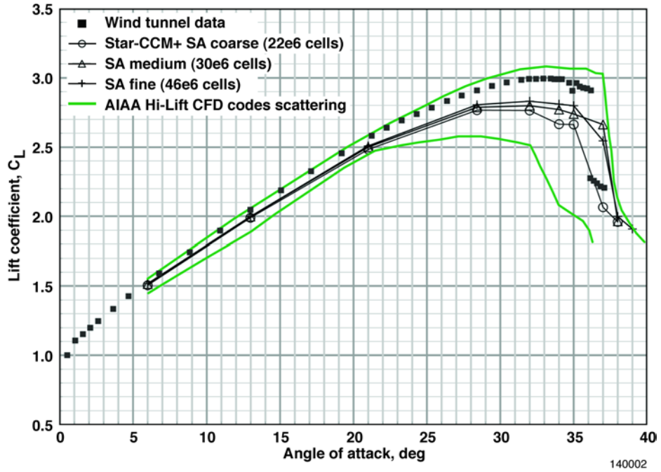
Figure 4. Star-CCM+ CFD code validation results for lift coefficient, Mach 0.2, Reynolds number based on mean aerodynamic chord of 4.3 million.
