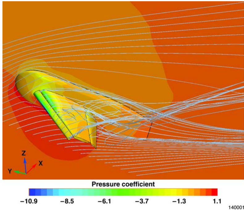
Figure 3. Geometry for the First AIAA CFD High Lift Prediction Workshop configuration 1.
