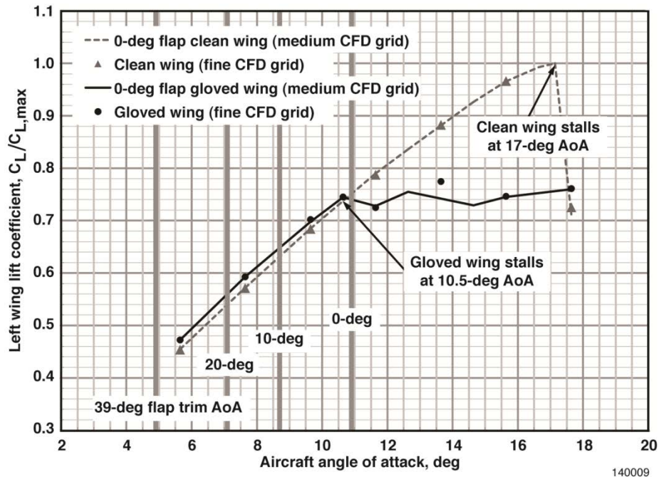
Figure 9. Star-CCM+ CFD wing lift coefficient stall results, 120 knots, 2300 ft above MSL.
