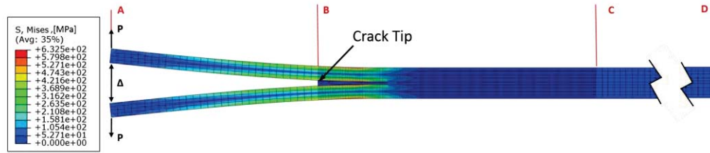
Figure 5. Von Mises stress, S , contour plot from the DCB numerical simulation.
