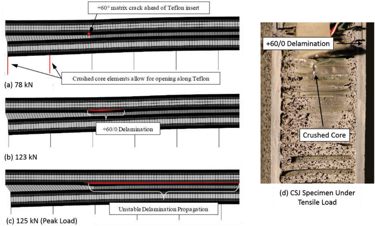
Figure 9. Failure process for conventional splice joint subjected to tensile loading, numerical and experimental.
