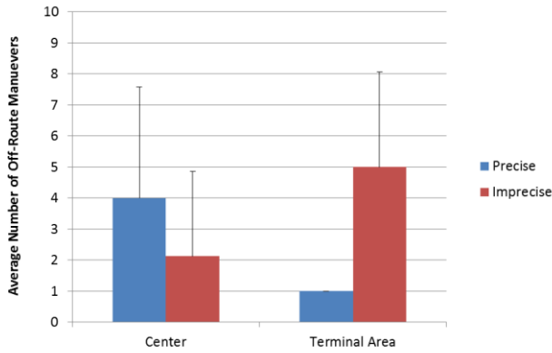
Figure 13. Preconditioning effects on lateral route conformance by control region.
