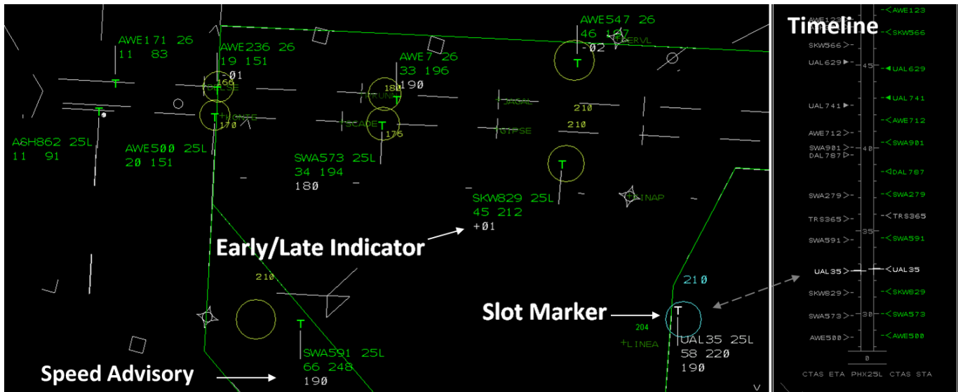
Figure 2. Controller-Managed Spacing (CMS) tools, illustrating synchronous highlighting of data block, slot marker, and timeline entries.
