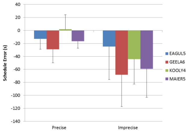
Figure 11. Meter-fix schedule conformance by preconditioning level and assigned RNAV OPD (negative values indicate aircraft arrived early).
