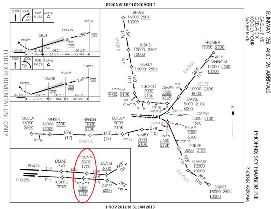
Figure 5. Experimental chart depicting PHX terminal-area RNAV OPDs, with final-approach fixes circled and artificial base-legs in red.
