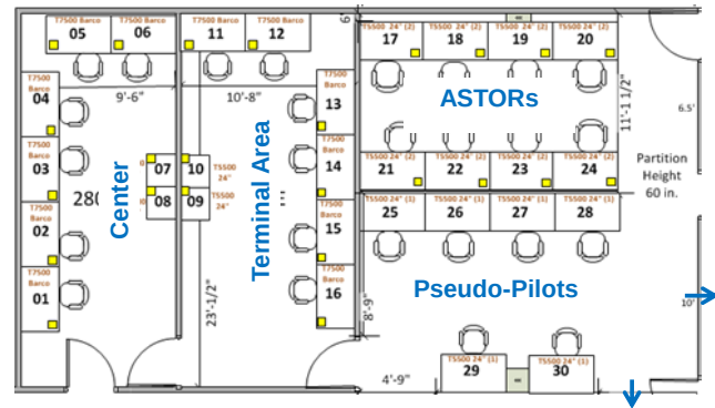
Figure 10. AOL laboratory layout for CA-4.
