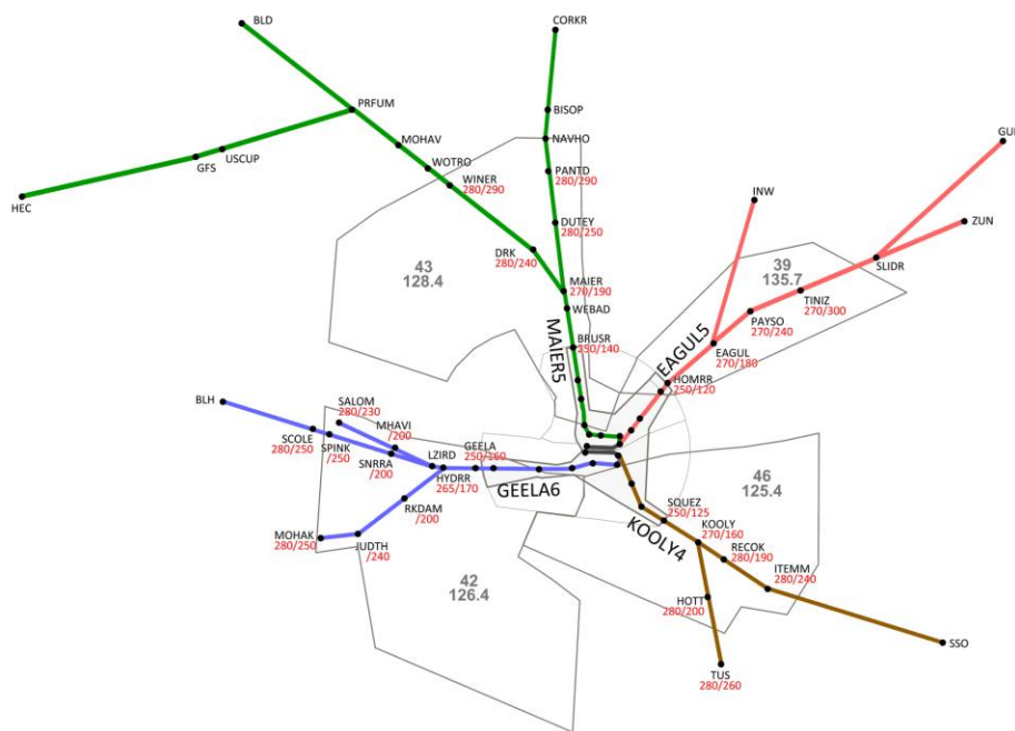
Figure 4. PHX west-flow RNAV OPDs and arrival transitions through low-altitude en-route sectors.
