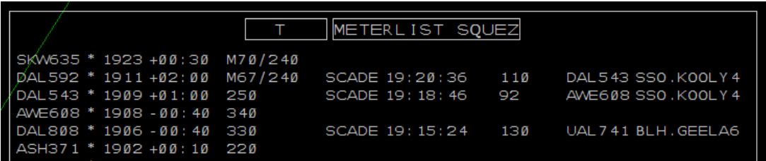
Figure 7. Meter list display on en-route controller workstation, showing FIM-clearance parameters for FIM-equipped aircraft; from left to right, the parameters are achieve-by point, STA at achieve-by-point, required spacing interval, lead aircraft, and lead aircraft’s assigned RNAV OPD.
