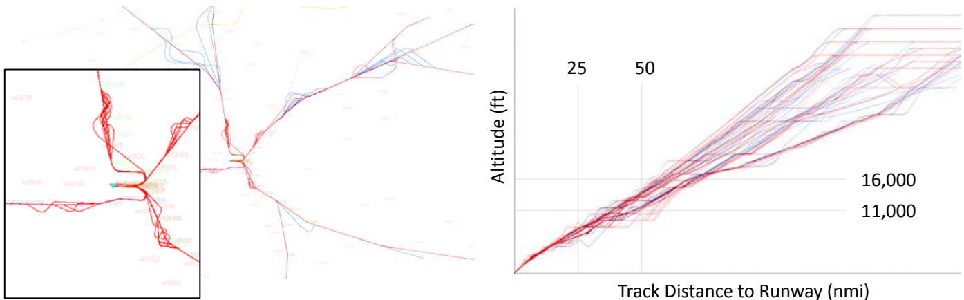
Figure 12. Comparison of lateral tracks and vertical profiles for one CA-4 trial with precise preconditioning (blue), and one without (red).
