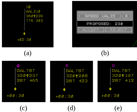
Figure 8. En-route speed advisories and FIM-status designators.
