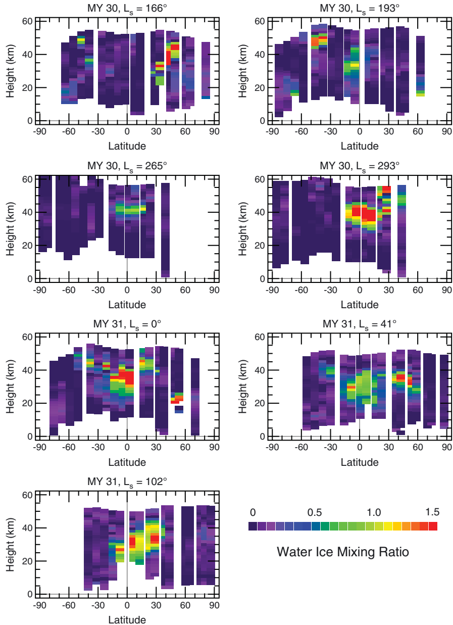
Figure 13. Cross sections showing the seasonal variation of water ice vertical and latitudinal distributions. All retrievals are from orbits near 290^\circ W longitude.
