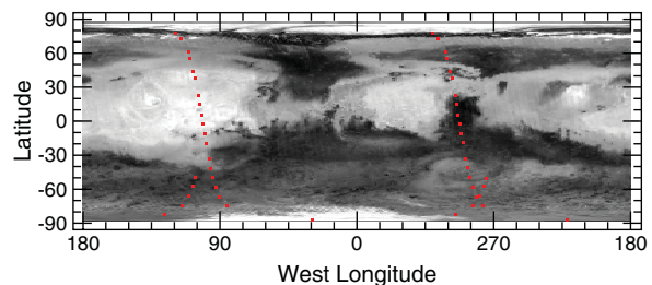
Figure 1. The latitude and longitude locations (small red squares) of CRISM limb scans for a limb set taken in July 2009 (MY 29, L s = 301°). A typical limb set contains pole-to-pole coverage at two longitudes at approximately 100° W and 290° W. Other CRISM limb sets have similar distribution.
