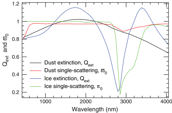
Figure 4. The extinction coefficient, Q_{\text{ext}} , and single-scattering albedo, \bar{\omega}_0 , for dust and water ice aerosols used in this retrieval. The extinction coefficient has been scaled to unity at the reference wavelength of 2219 nm. These scattering properties are based on the analysis of TES and CRISM observations [Wolff and Clancy, 2003; Clancy et al. , 2003; Wolff et al. , 2009] and are representative of a mean particle size of 1.5 \mu\text{m} for dust and 2.0 \mu\text{m} for water ice aerosols.
