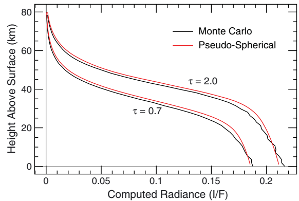
Figure 6. A comparison of computed radiance at a wavelength of 1 \mu\text{m} in the limb geometry between the “exact” Monte Carlo results (black lines) and the pseudo-spherical approximation (red lines) for two different column optical depths of dust aerosol, \tau . The pseudo-spherical approximation is accurate to within a few percent over a wide range of conditions and is two orders of magnitude faster than the Monte Carlo calculation.
