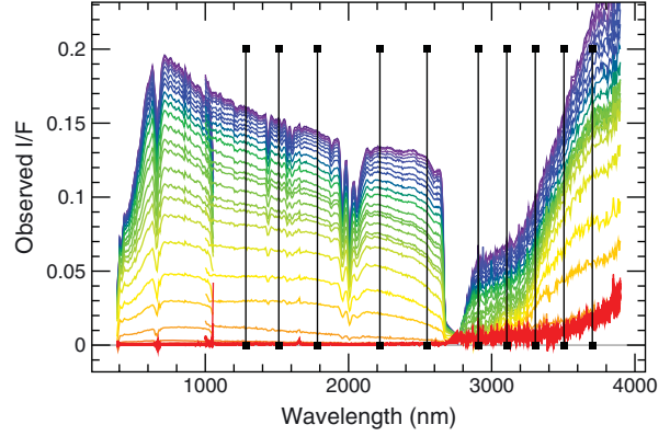
Figure 3. A typical CRISM limb scan from the limb set taken in July 2009 (MY 29, L_s = 301^\circ , 19^\circ\text{S} latitude, 290^\circ\text{W} longitude). Color indicates tangent height above the surface, from purple (0 km) to red (50 km). The black vertical lines indicate the 10 wavelengths used to retrieve aerosol vertical profiles.
