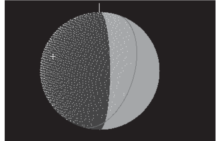
Geminids 12/13/1972
