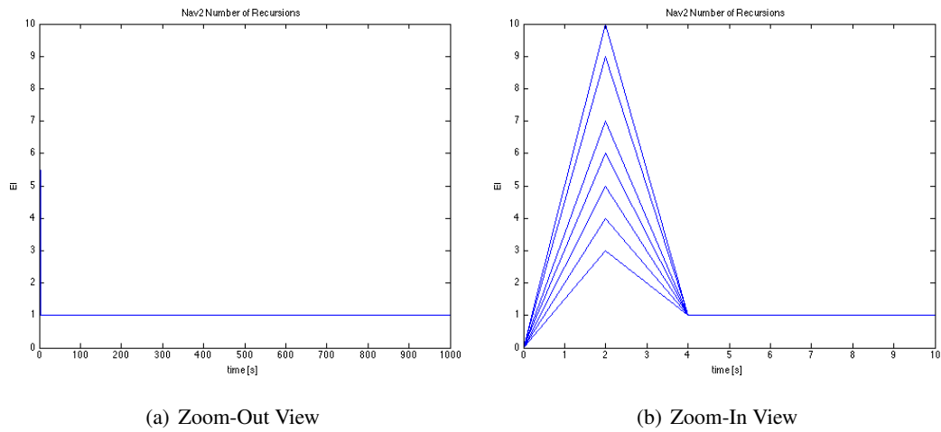
Figure 4. Number of Recursions Selected by Algorithm.
