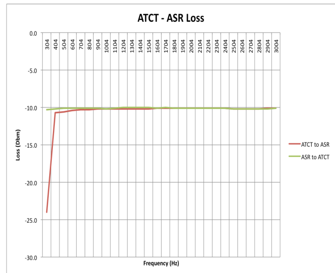
Figure 9 – AeroMACS-ASR-9 Test Voice Grade Line Performance
