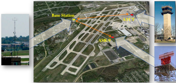
Figure 7 – Wireless Configuration for ASR-9 Safety Critical Fixed Asset Tests.
