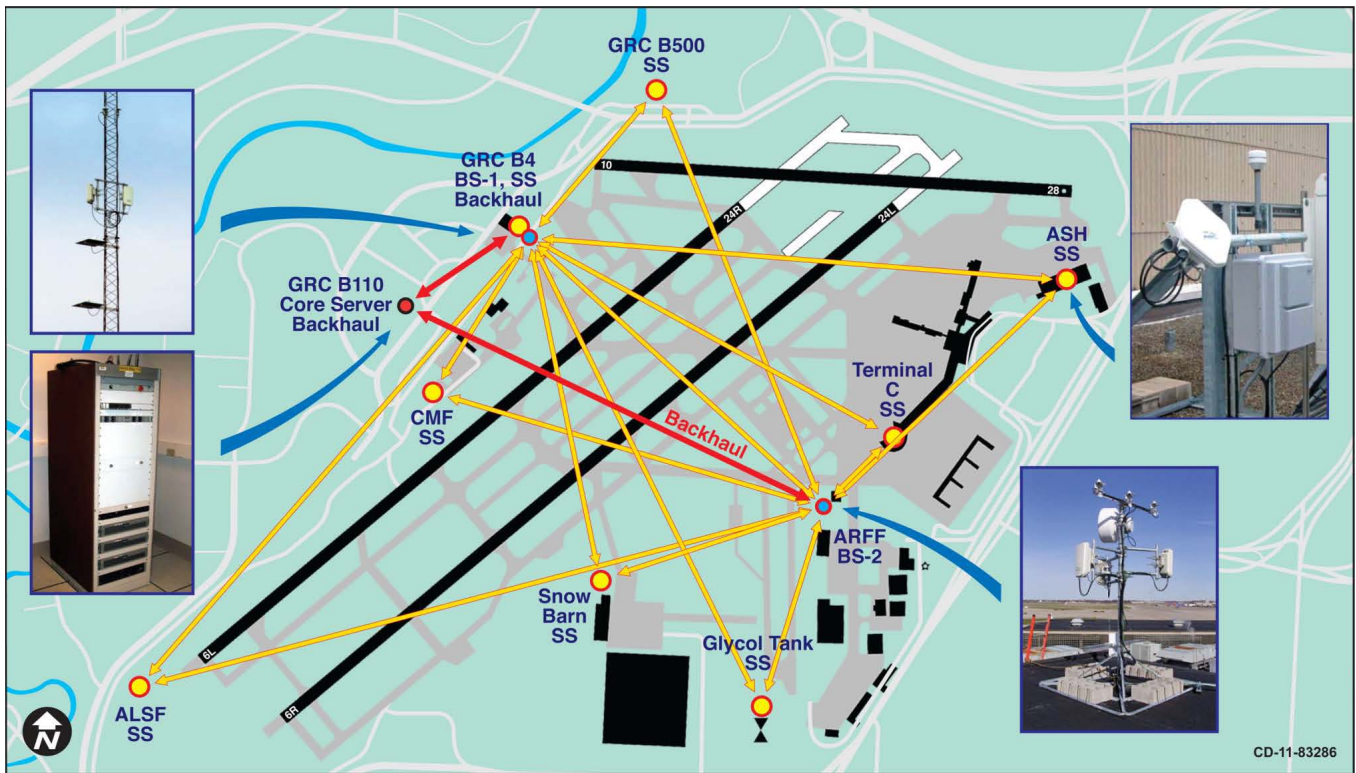
Figure 1 – AeroMACS Prototype Testbed.
