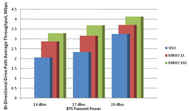
Figure 3 – Average Throughput Rate for the Service Road Drive Test
