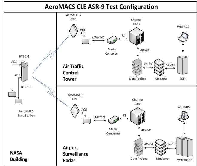
Figure 8 – AeroMACS-ATCT-ASR-9 Interfaces
