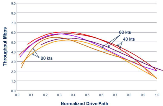
Figure 5 – Effects of Vehicle Velocity on Throughput from Runway 24L Taxi Tests.
