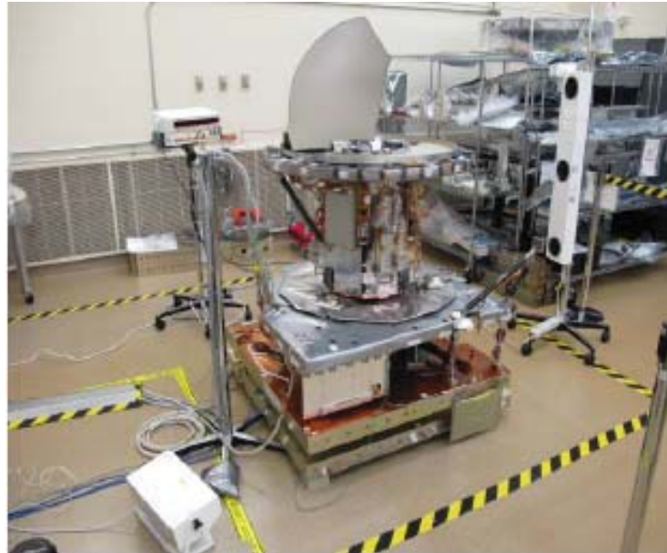
Figure 1. Dynamometer Assembly Setup in Calibration and GMI without RDA and MR Assys Integrated
