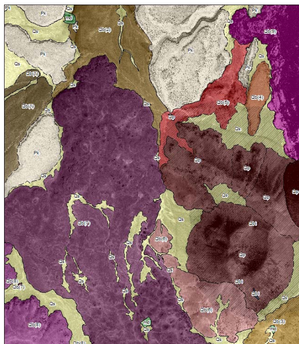
Figure 1. Geologic map of the V7504 field area, San Francisco Volcanic Field, north-central AZ. A chief question of the field mapping was the nature and evolution of the V7504 vent complex, identified here in brown.
