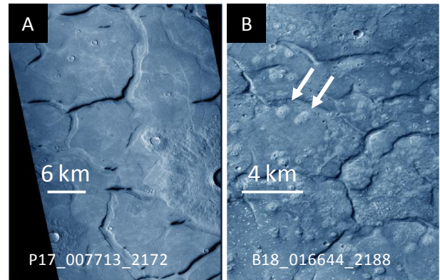
Fig. 2. Giant polygons - Mars. A. S. Utopia. B. Acidalia showing associated mounds (arrows).
